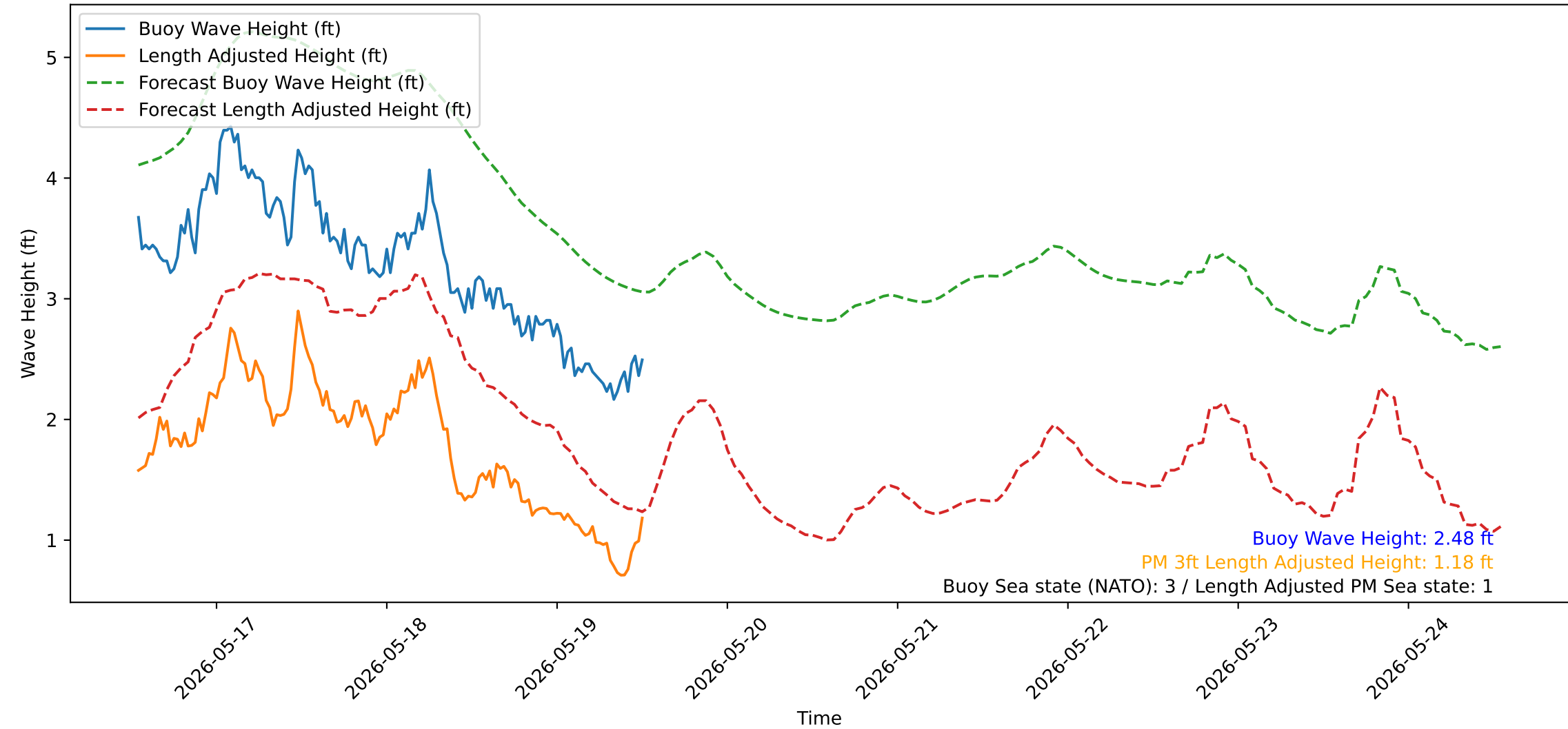
Wave Heights over Time for Green Beach at 2026-05-19 12:51:14
