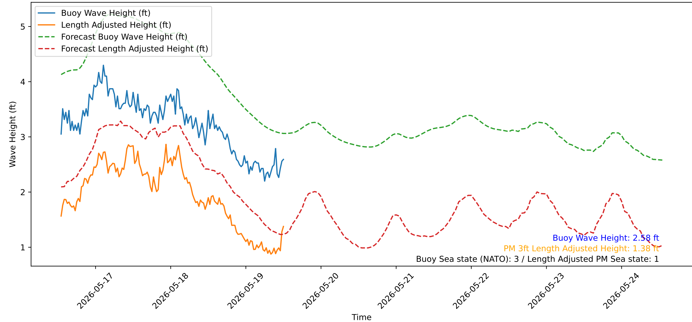
Wave Heights over Time for Oceanside Harbor at 2026-05-19 12:50:31
