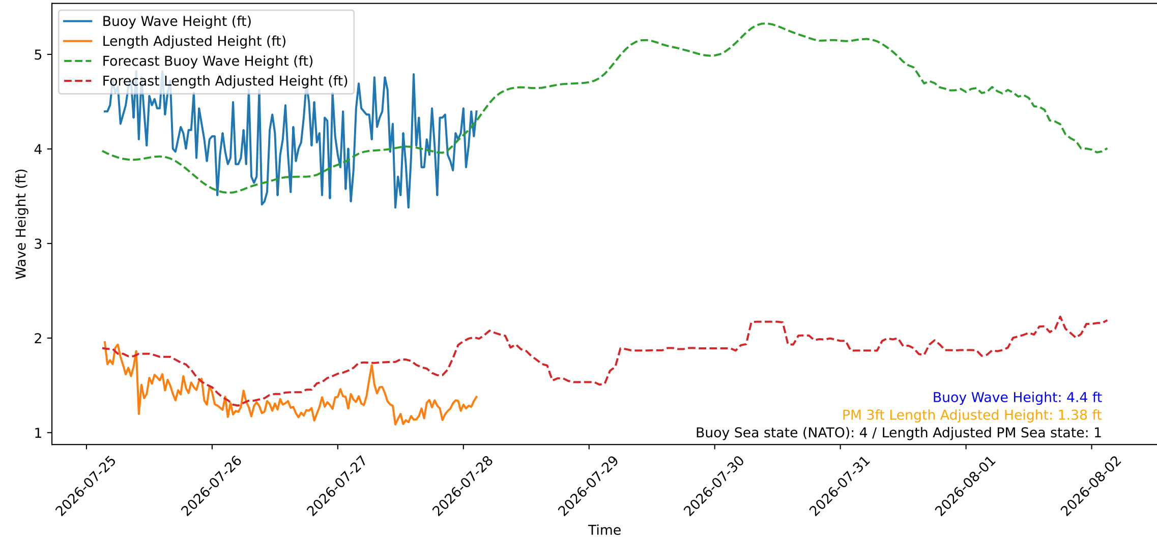
Wave Heights over Time for Green Beach at 2026-07-28 03:21:10
