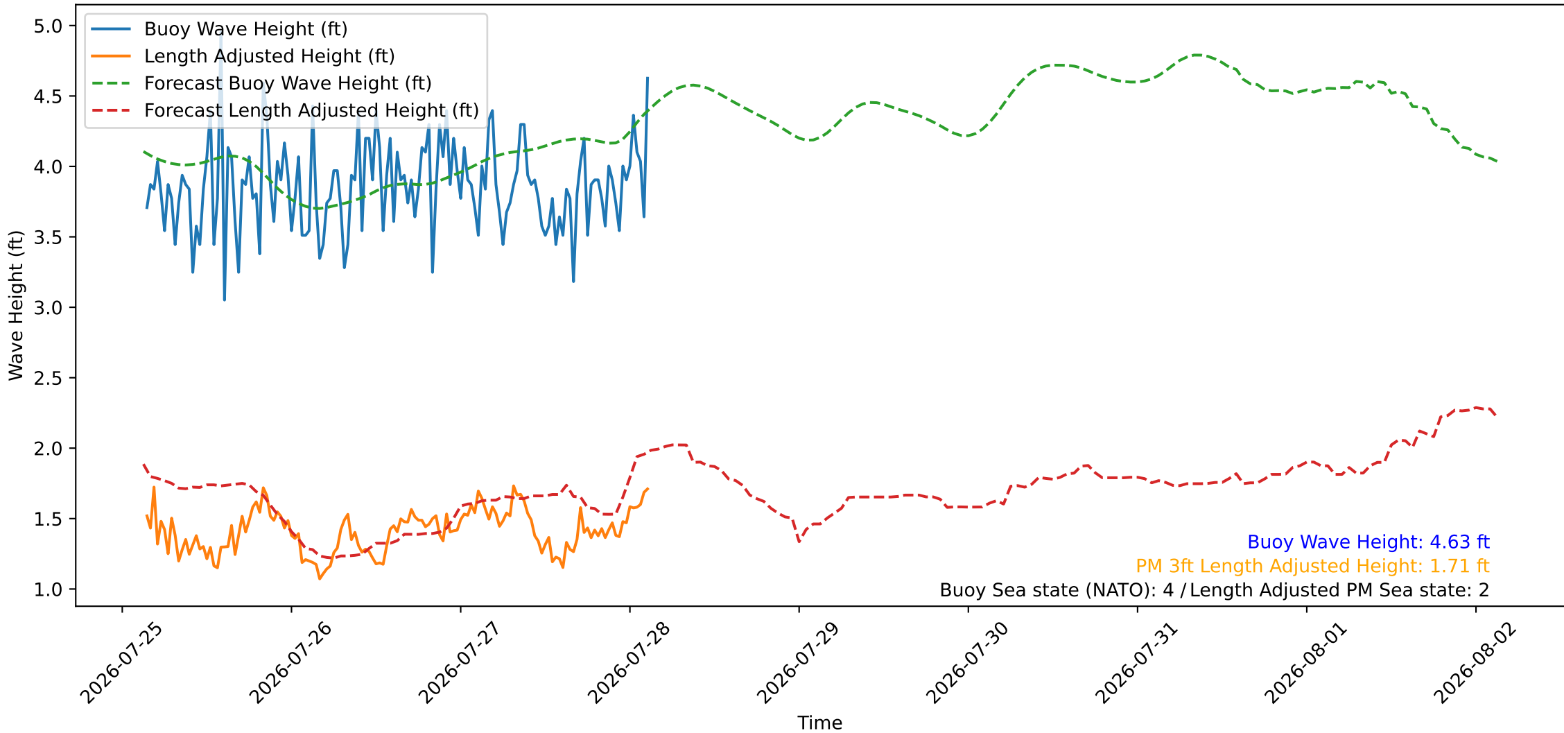
Wave Heights over Time for Oceanside Harbor at 2026-07-28 03:20:26
