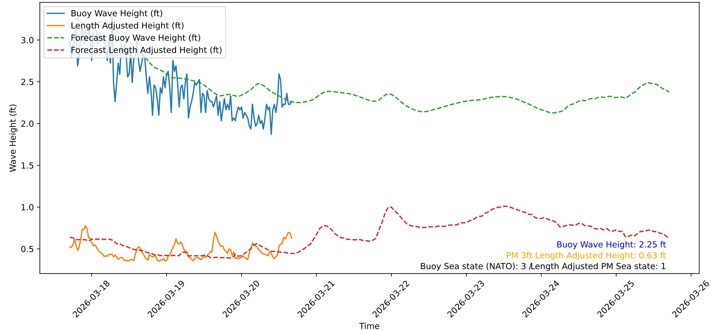
Wave Heights over Time for Red Beach at 2026-03-20 16:40:47
