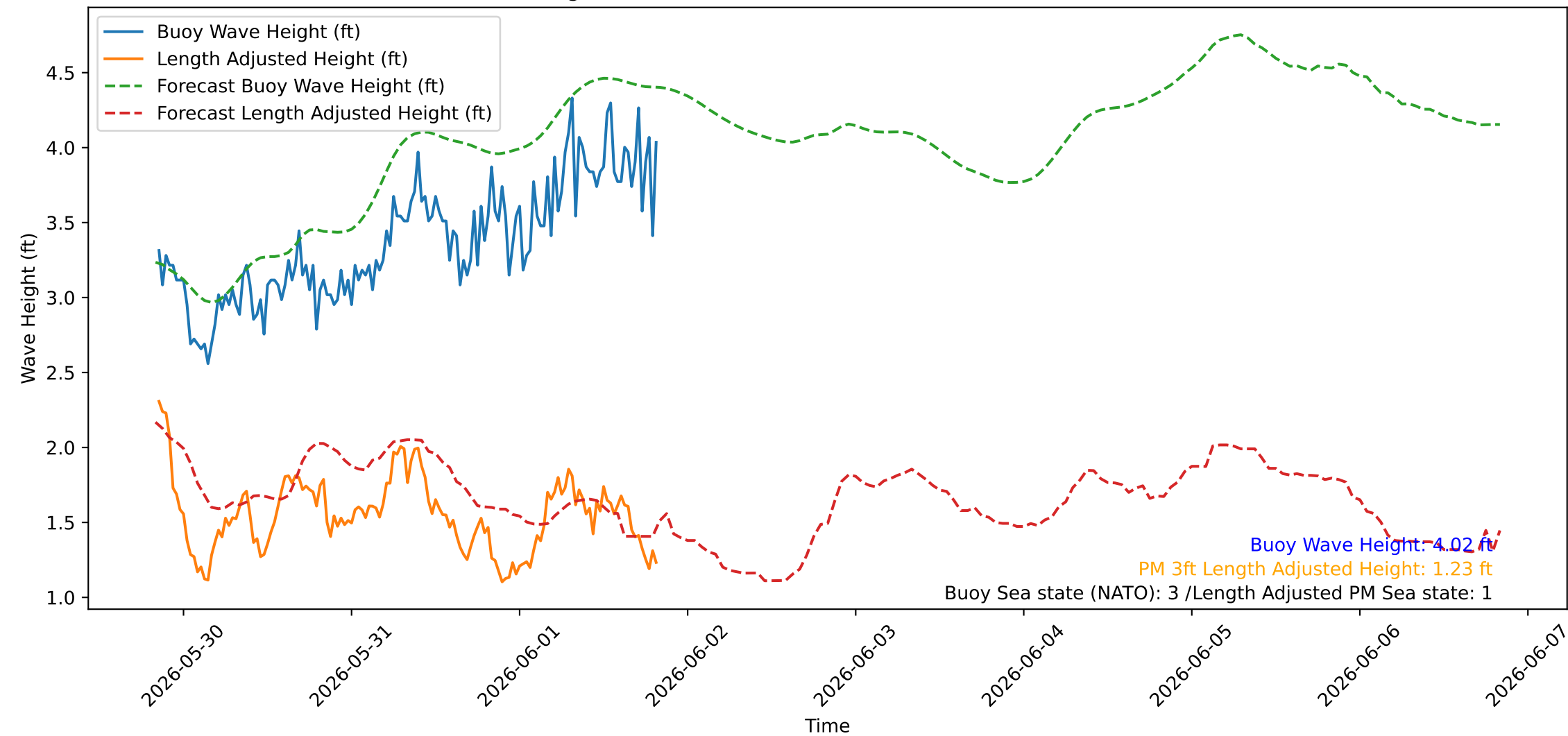
Wave Heights over Time for Green Beach at 2026-06-01 20:21:09
