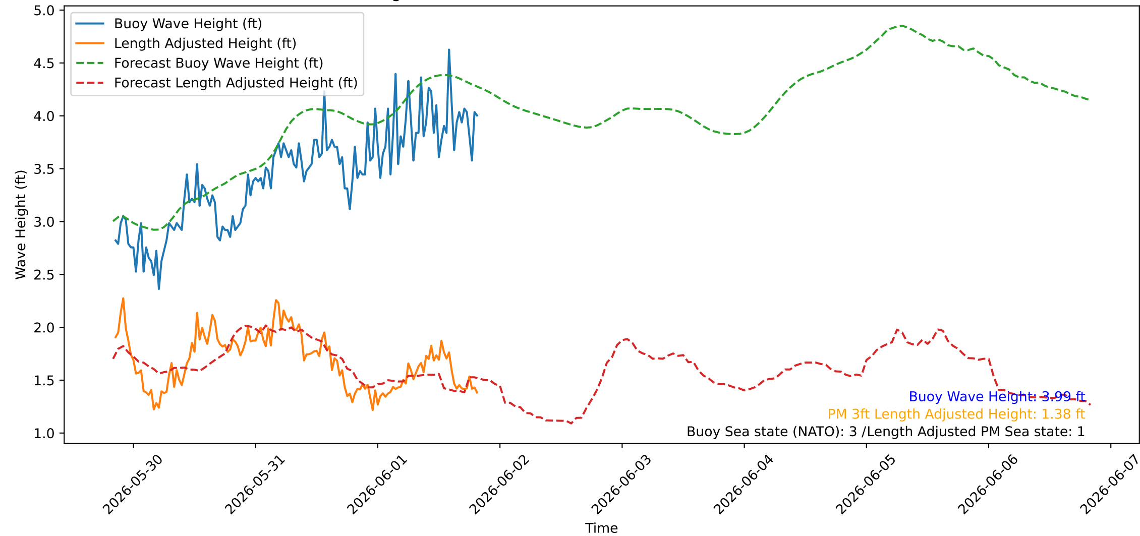
Wave Heights over Time for Oceanside Harbor at 2026-06-01 20:20:26
