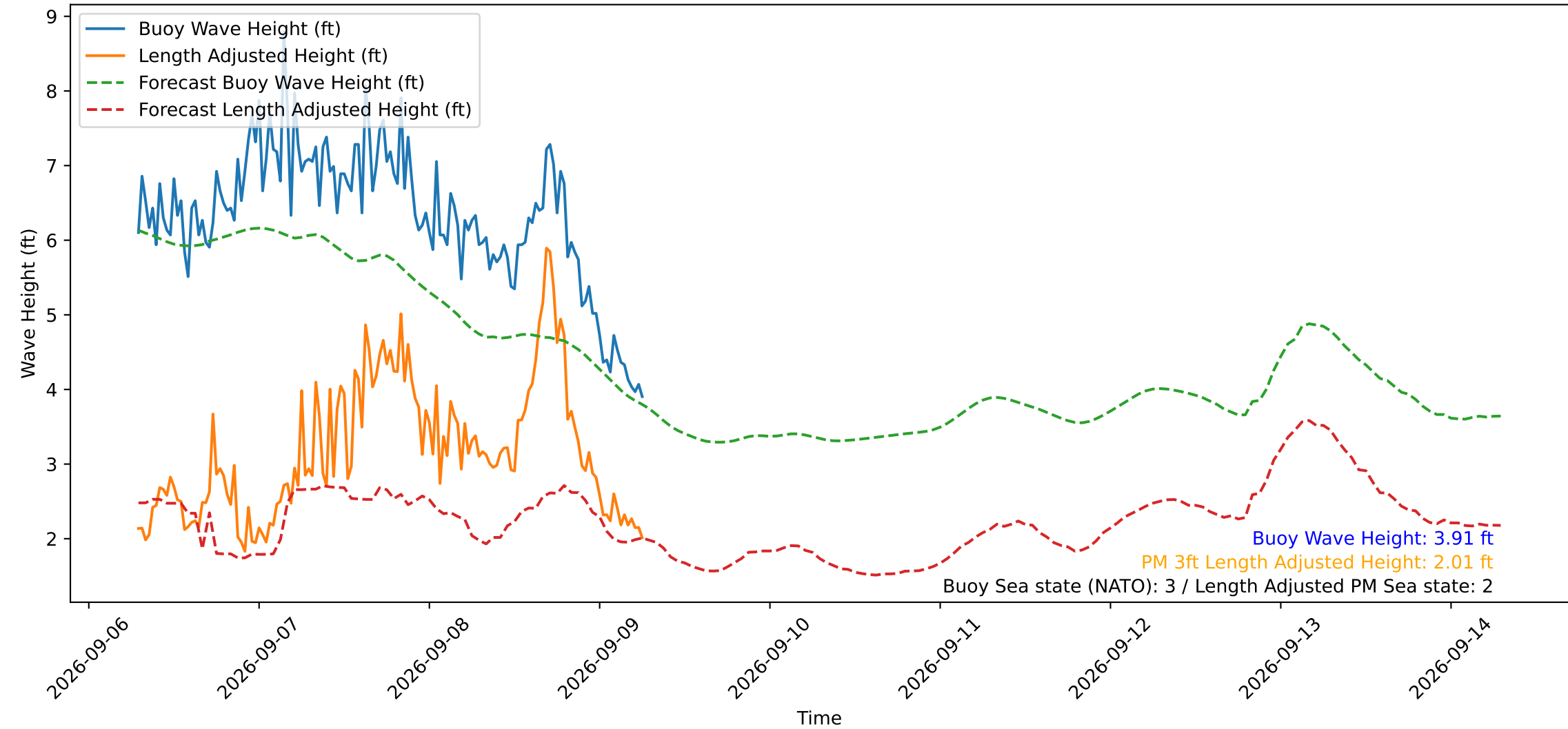
Wave Heights over Time for Green Beach at 2026-09-09 06:51:14
