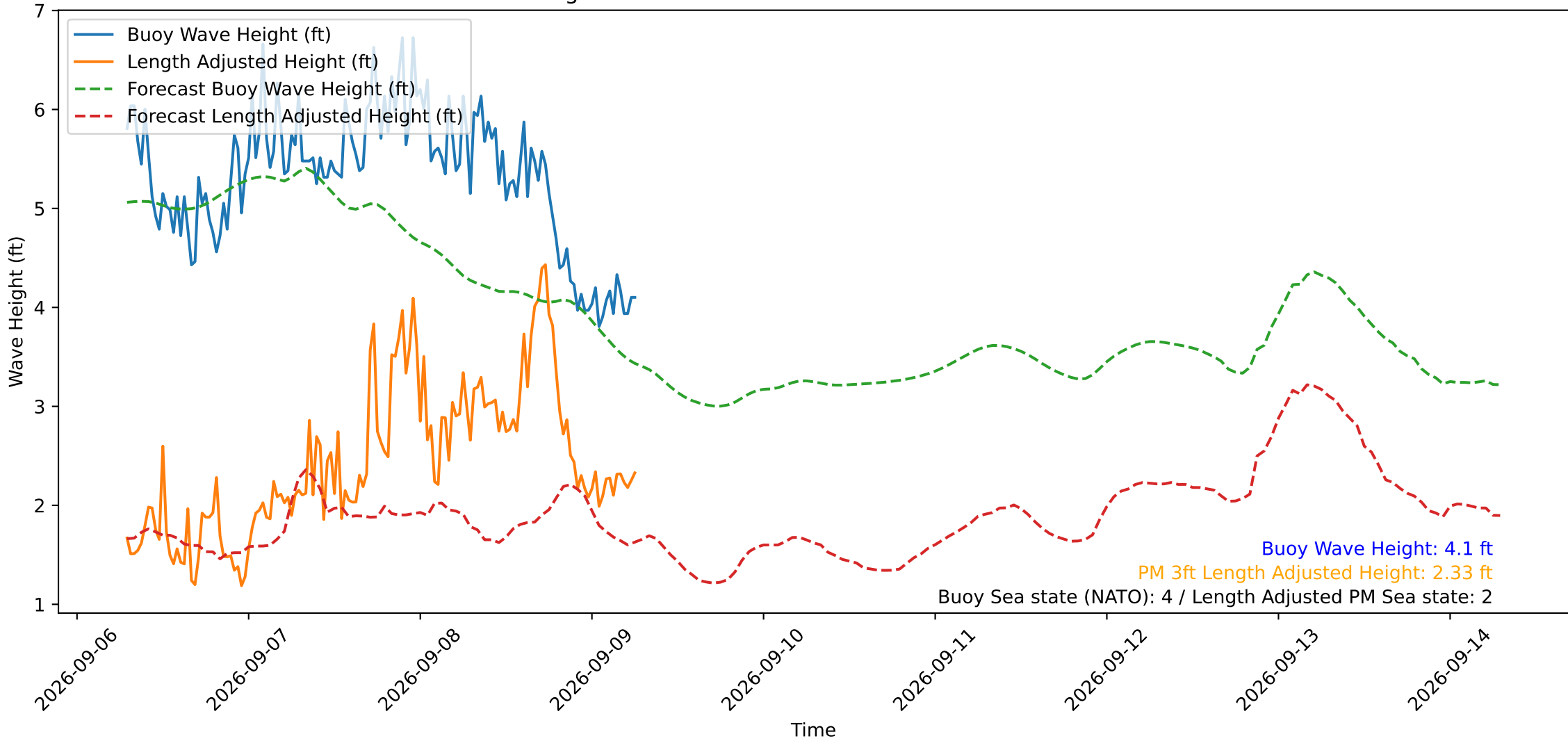
Wave Heights over Time for Red Beach at 2026-09-09 06:50:50
