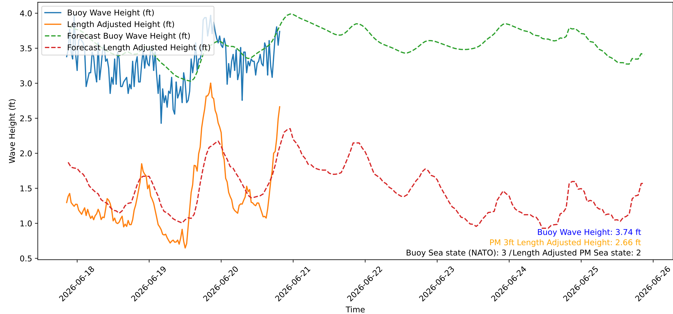
Wave Heights over Time for Green Beach at 2026-06-20 20:41:07
