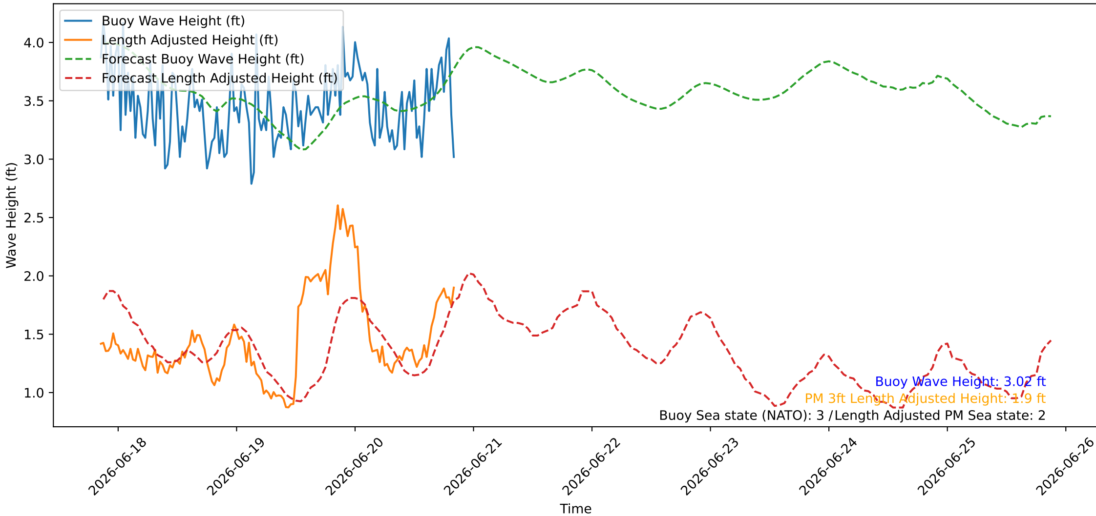
Wave Heights over Time for Oceanside Harbor at 2026-06-20 20:40:26
