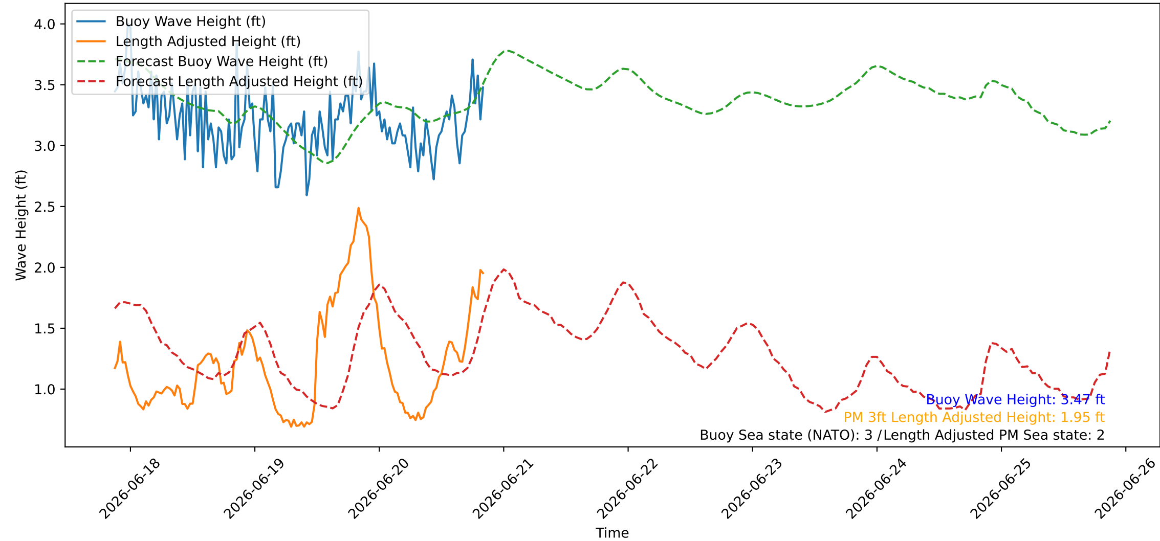
Wave Heights over Time for Red Beach at 2026-06-20 20:40:45
