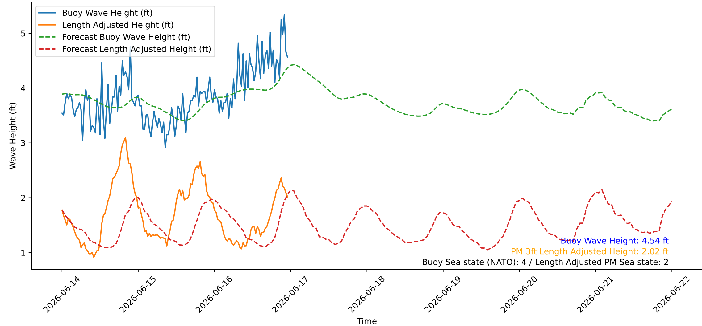
Wave Heights over Time for Red Beach at 2026-06-16 23:50:47
