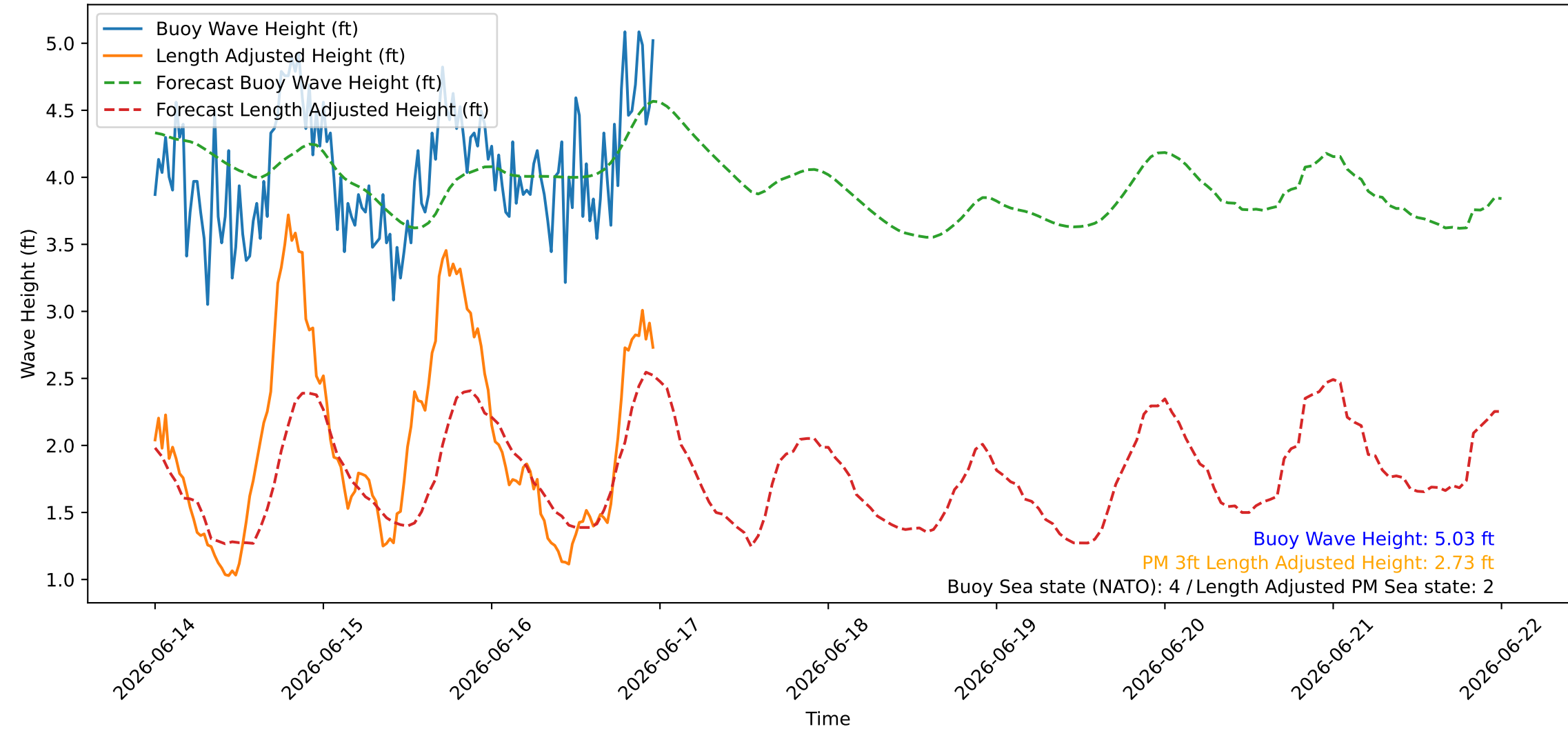
Wave Heights over Time for Green Beach at 2026-06-16 23:51:10
