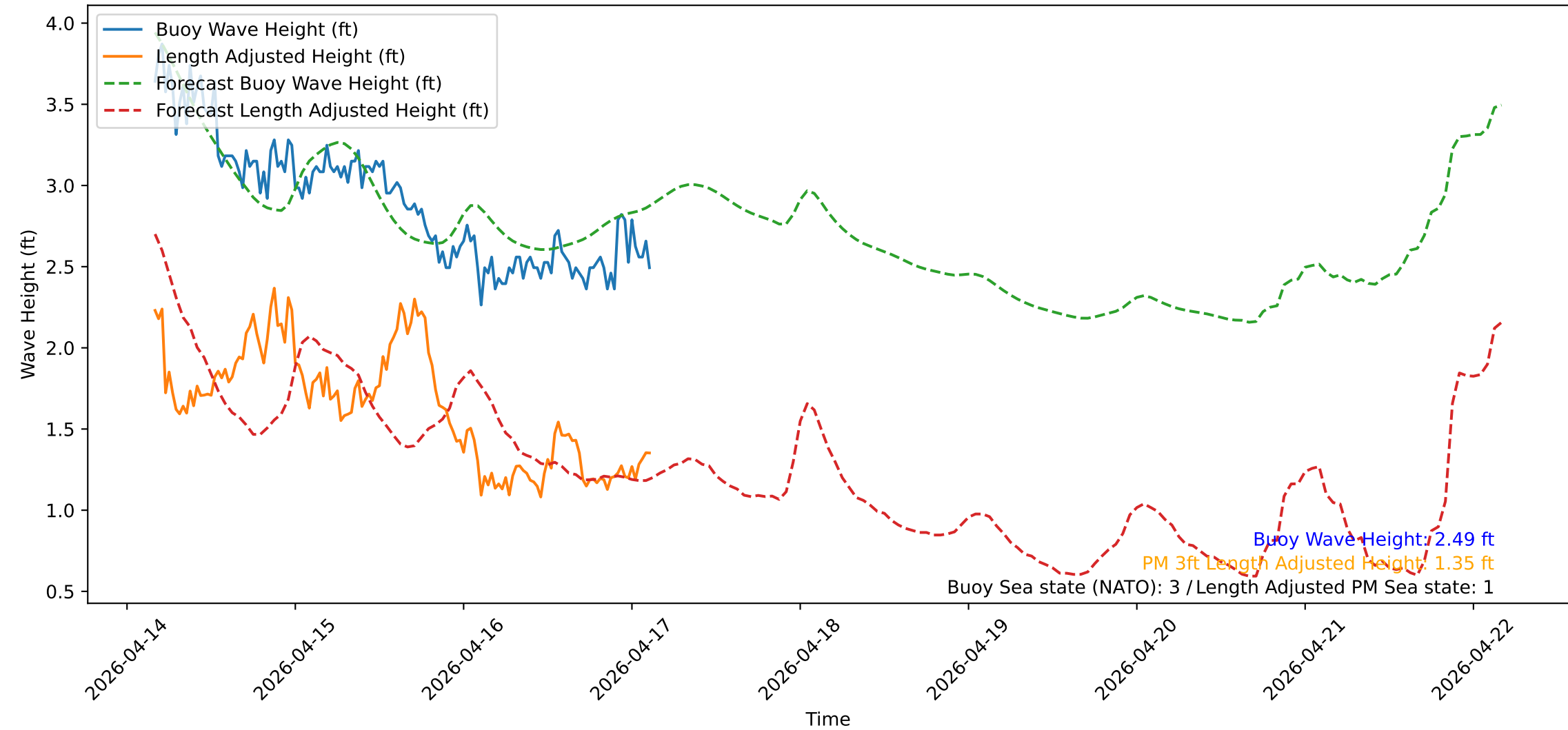
Wave Heights over Time for Red Beach at 2026-04-17 03:30:51
