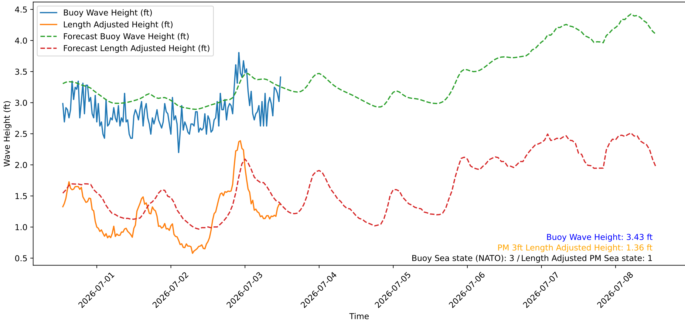
Wave Heights over Time for Red Beach at 2026-07-03 12:40:46
