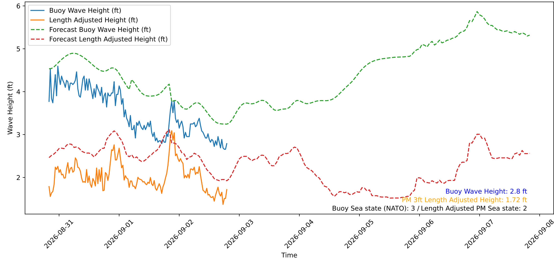
Wave Heights over Time for Green Beach at 2026-09-02 19:51:16
