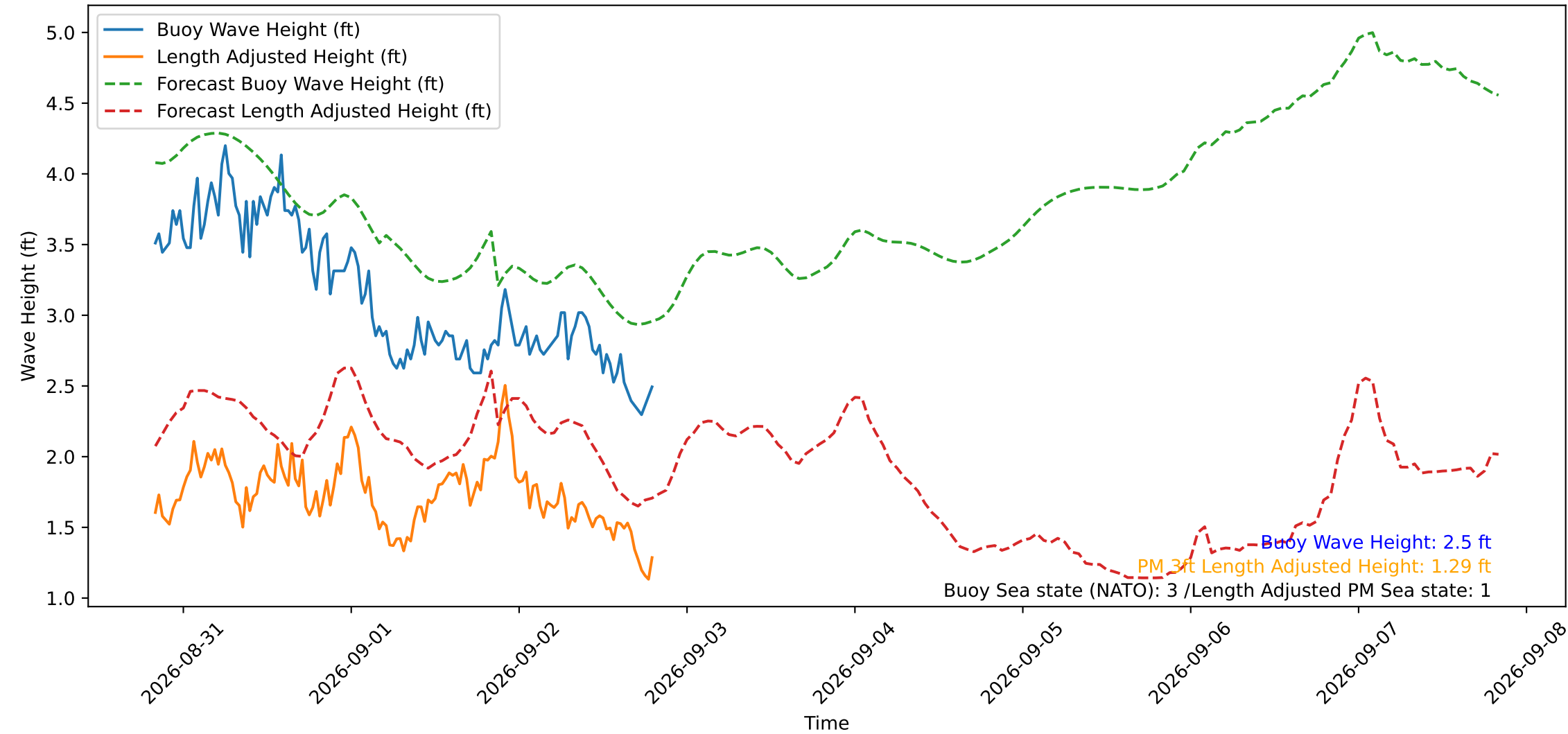
Wave Heights over Time for Red Beach at 2026-09-02 19:50:51
