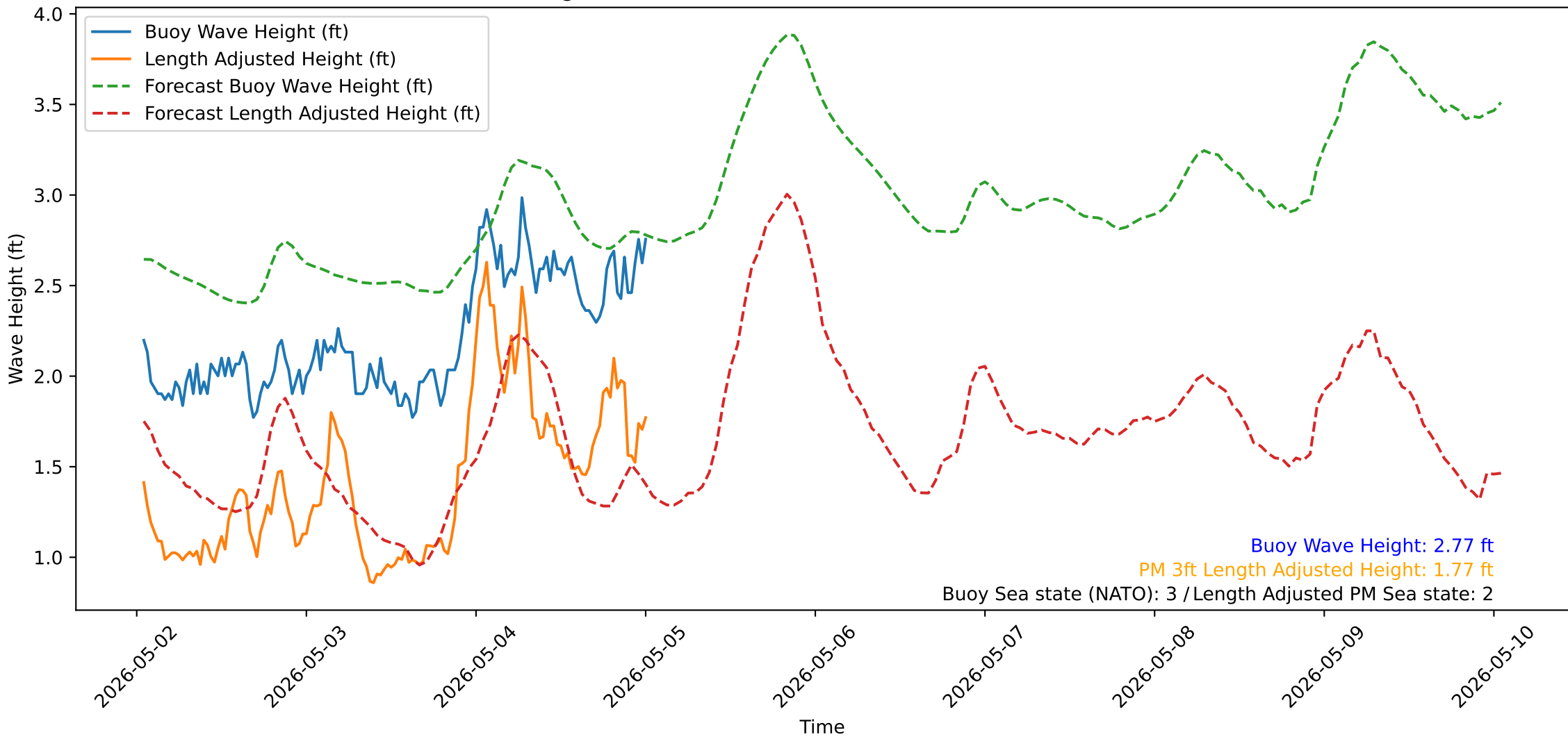
Wave Heights over Time for Green Beach at 2026-05-05 01:01:12
