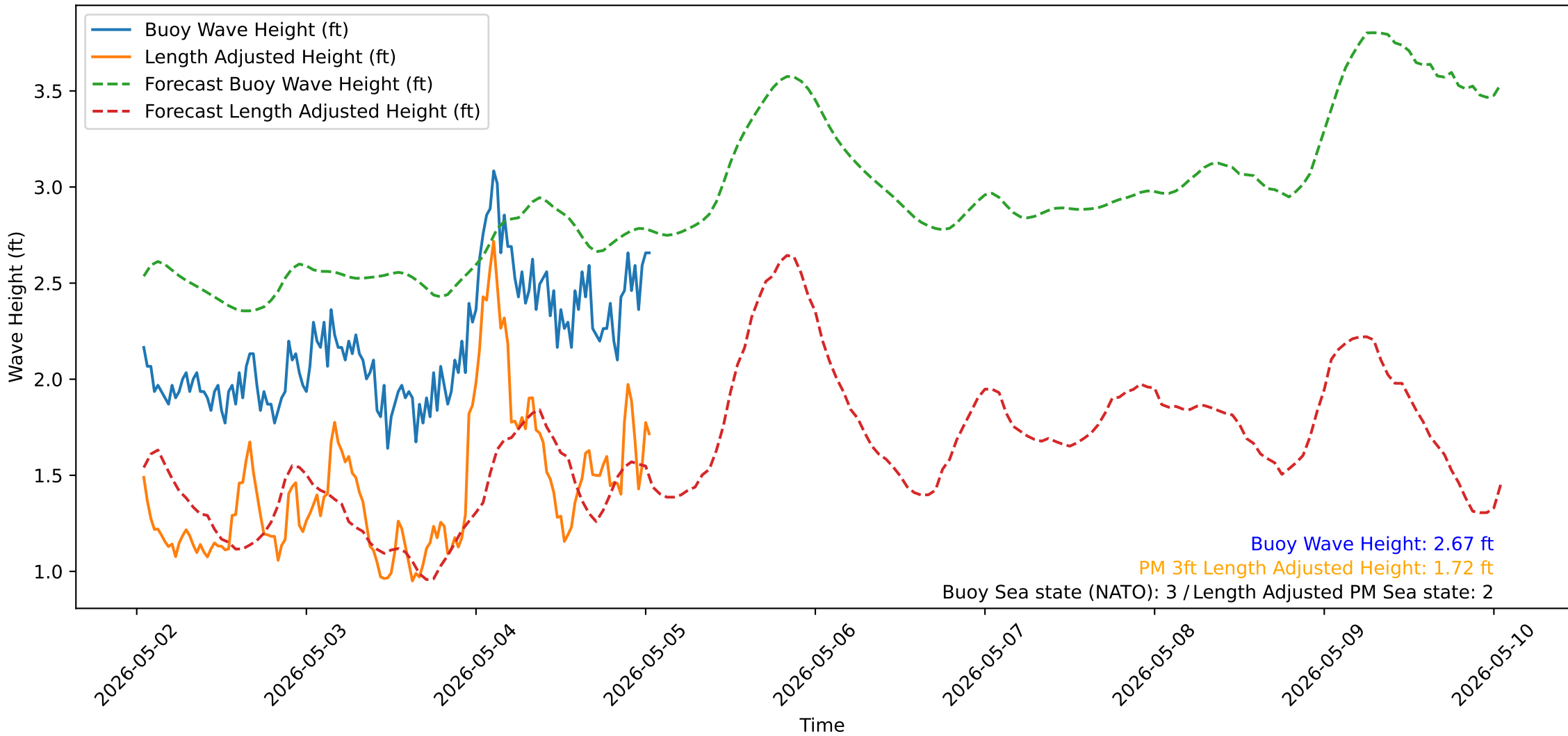
Wave Heights over Time for Oceanside Harbor at 2026-05-05 01:00:31
