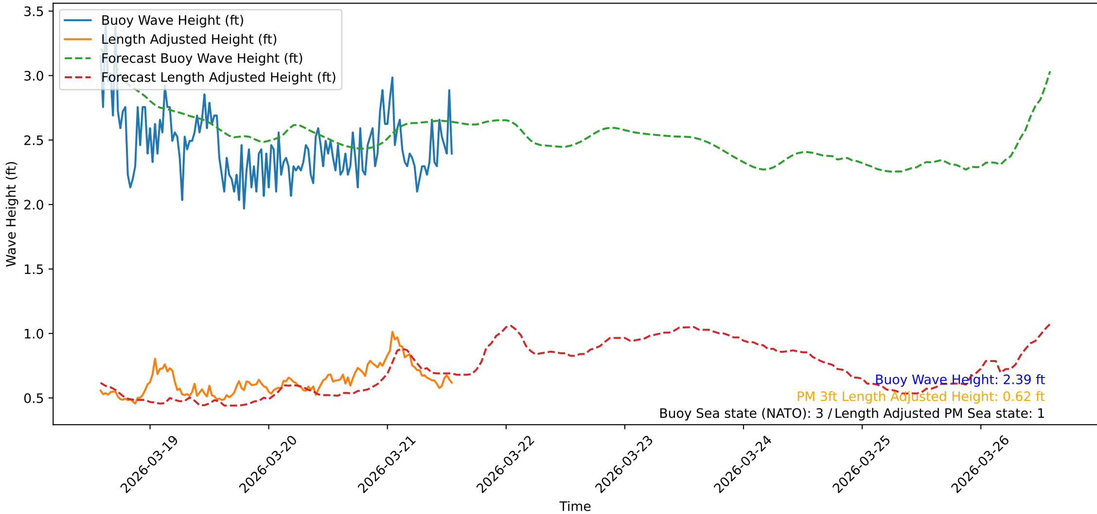
Wave Heights over Time for Oceanside Harbor at 2026-03-21 14:00:31
