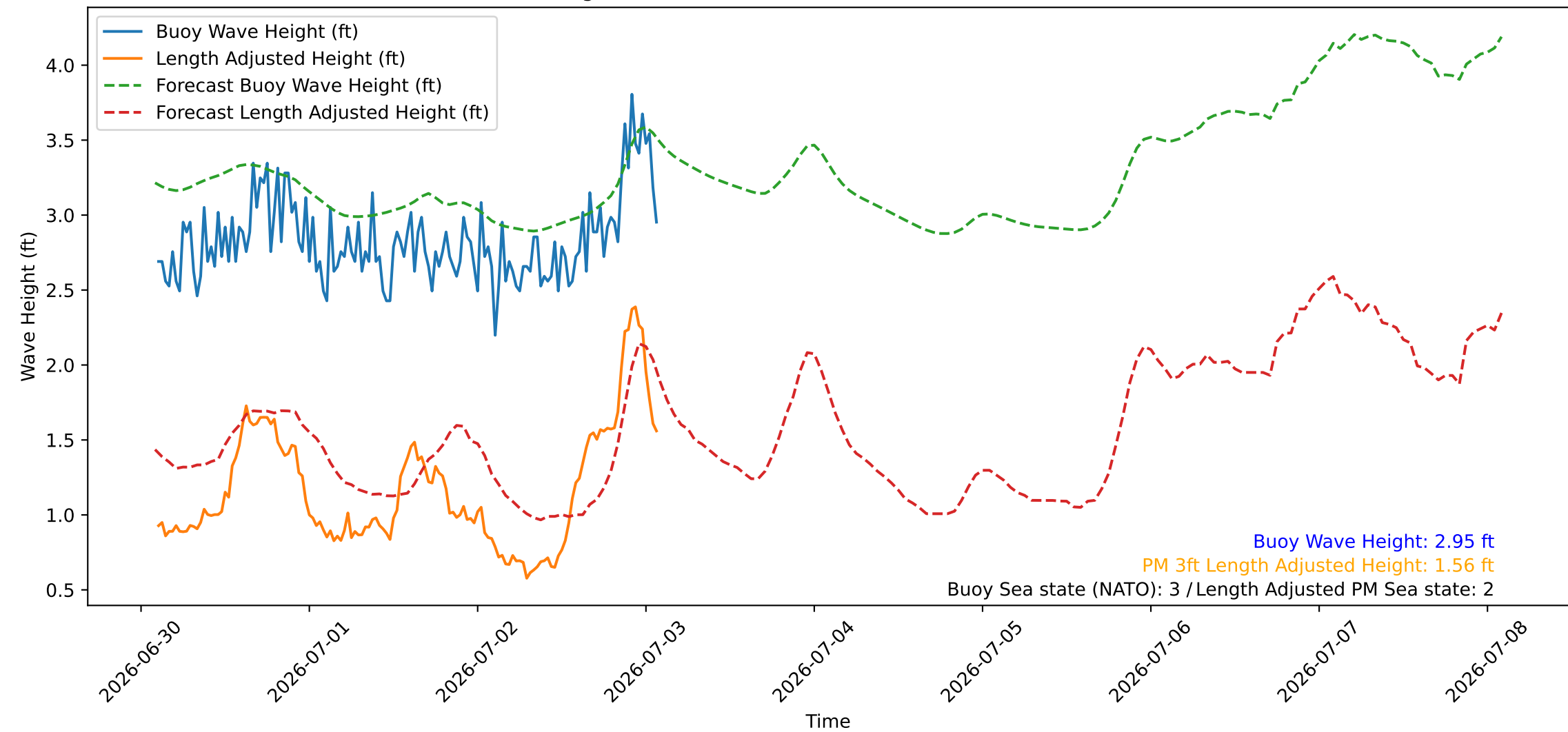
Wave Heights over Time for Red Beach at 2026-07-03 02:10:44
