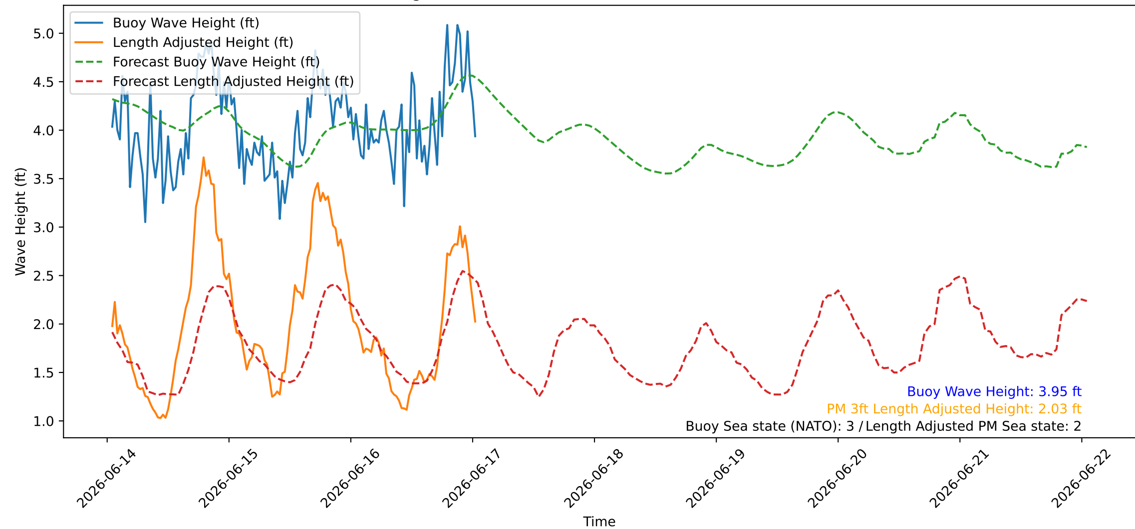
Wave Heights over Time for Green Beach at 2026-06-17 01:11:06
