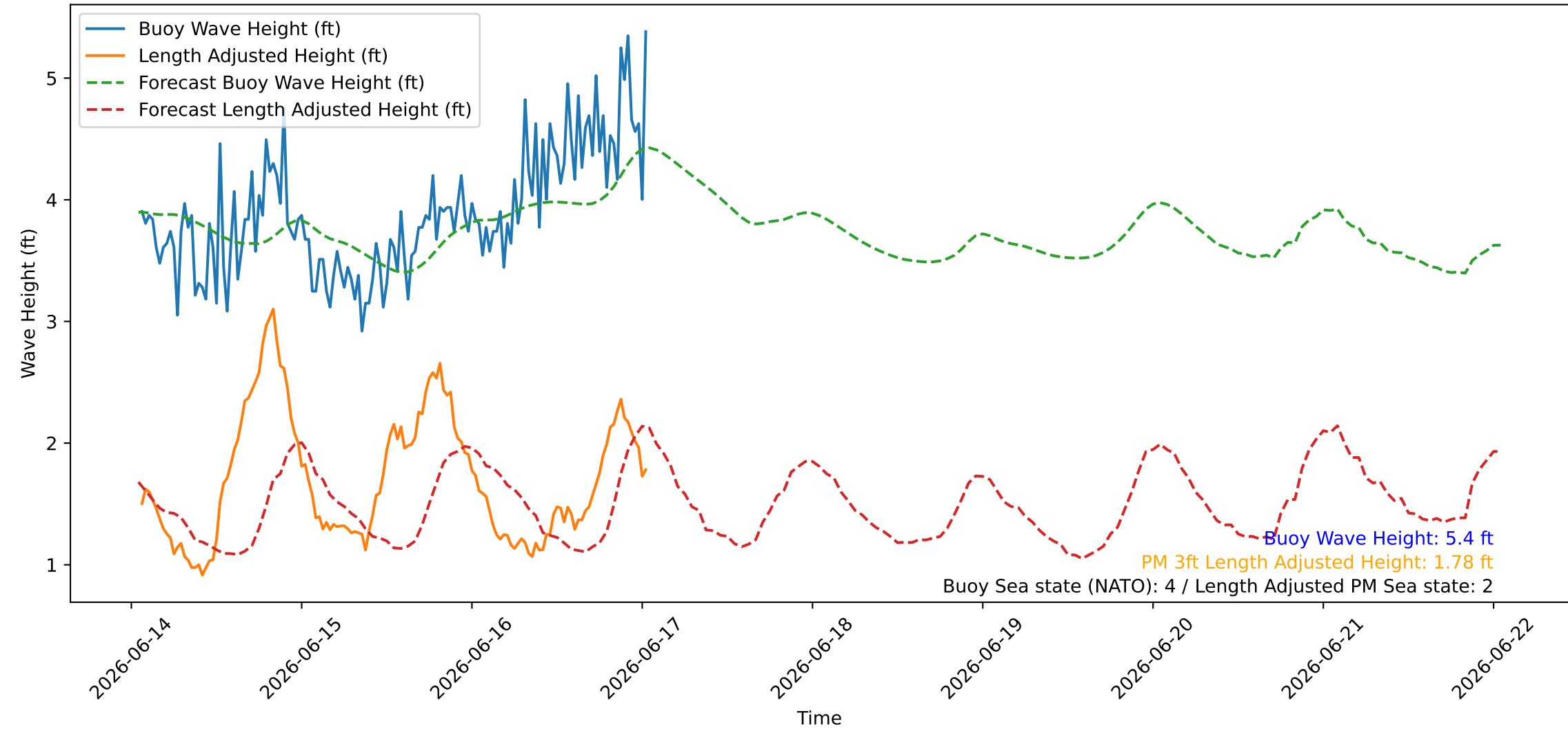
Wave Heights over Time for Red Beach at 2026-06-17 01:10:44
