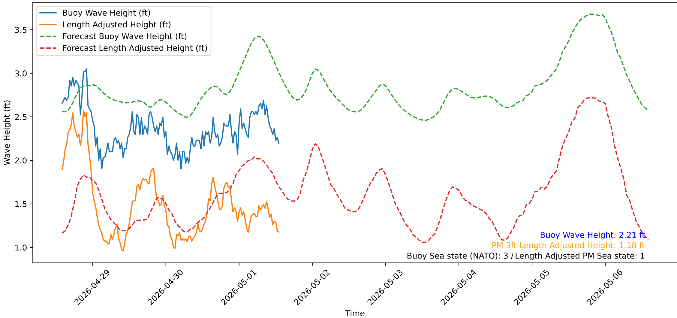
Wave Heights over Time for Oceanside Harbor at 2026-05-01 13:50:32
