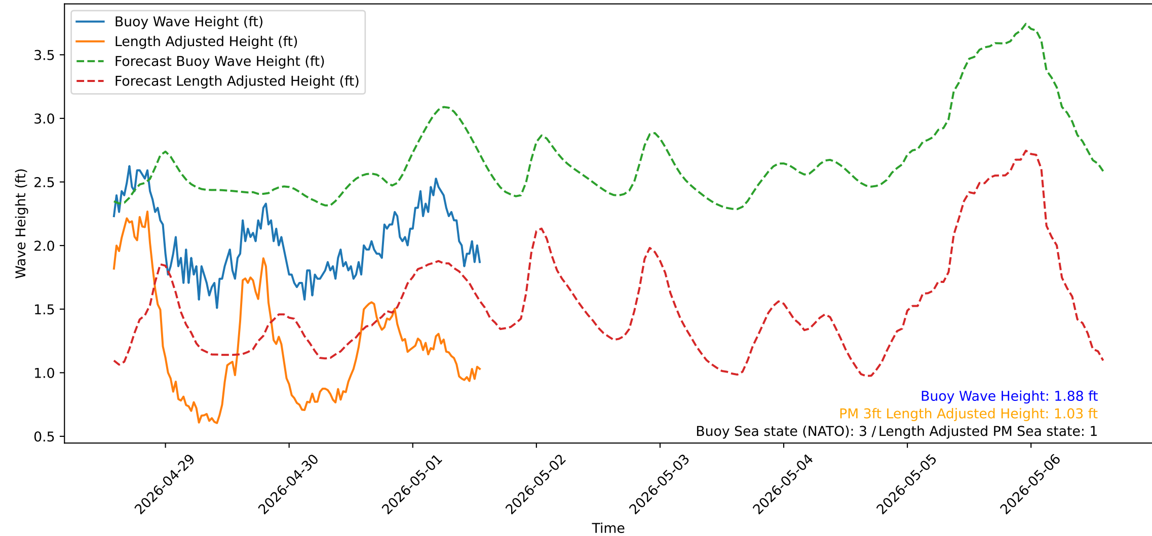
Wave Heights over Time for Red Beach at 2026-05-01 13:50:52
