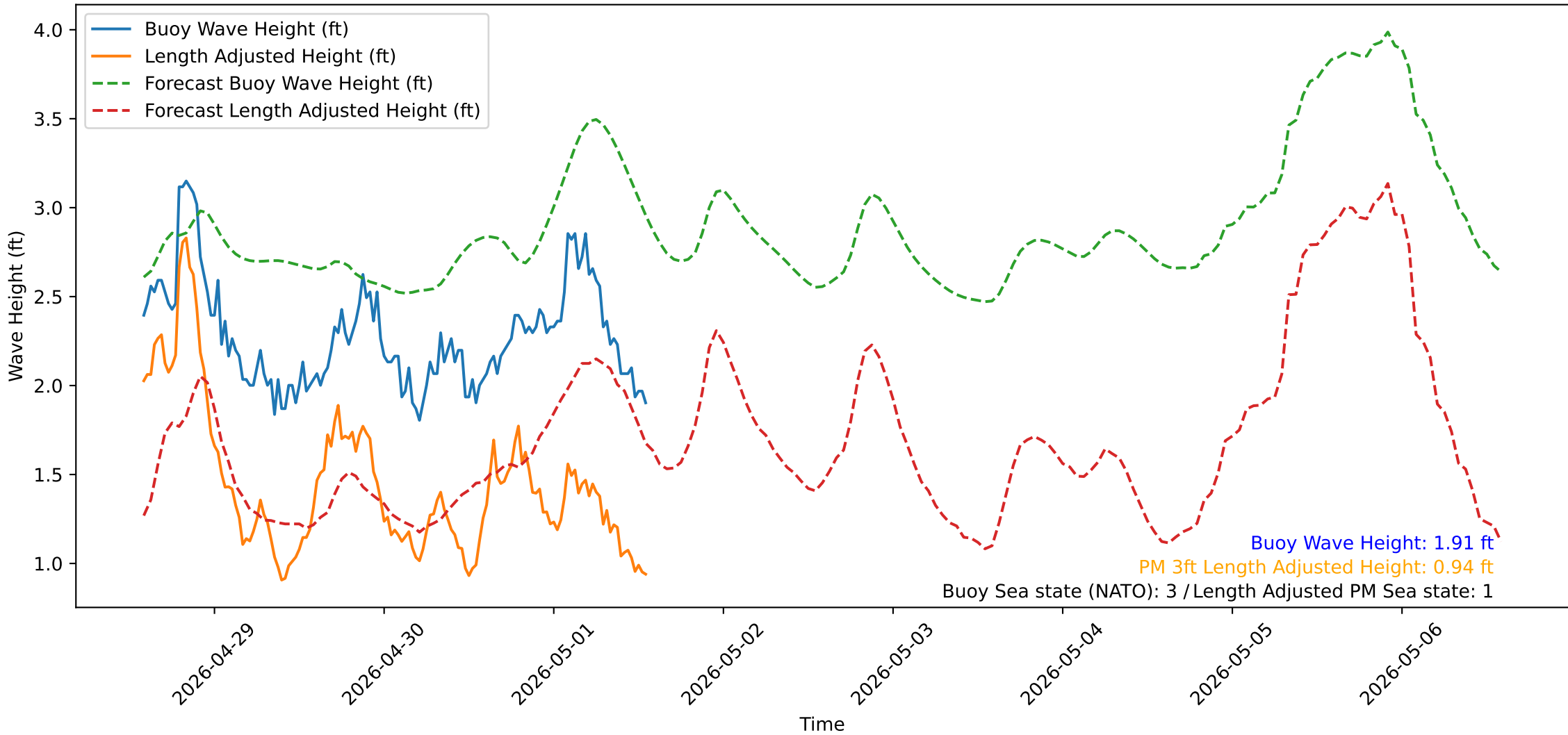
Wave Heights over Time for Green Beach at 2026-05-01 13:51:14
