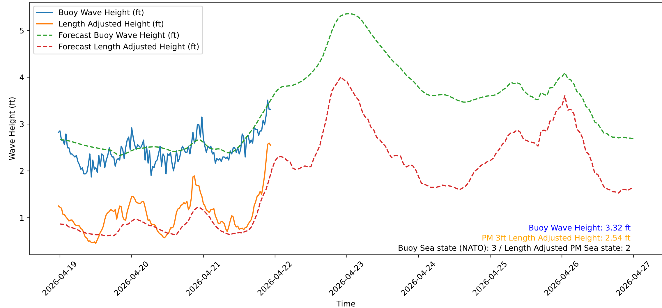
Wave Heights over Time for Green Beach at 2026-04-21 23:31:13
