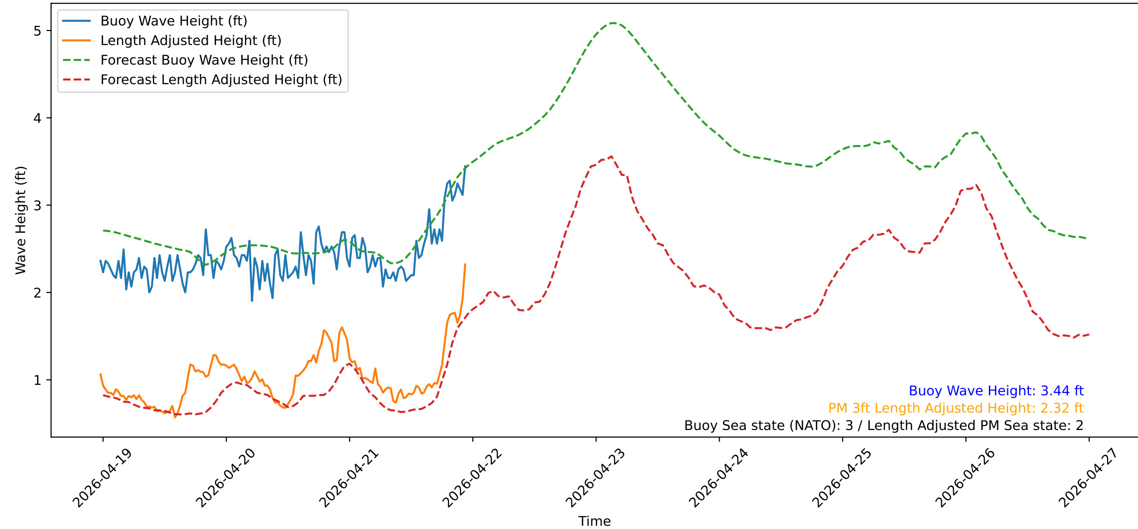
Wave Heights over Time for Oceanside Harbor at 2026-04-21 23:30:32
