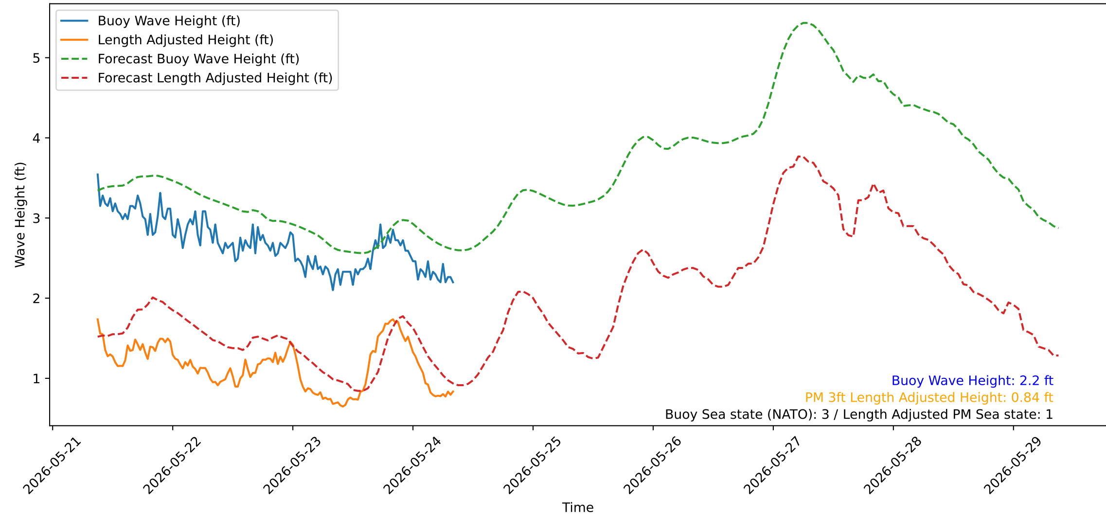
Wave Heights over Time for Green Beach at 2026-05-24 09:01:15
