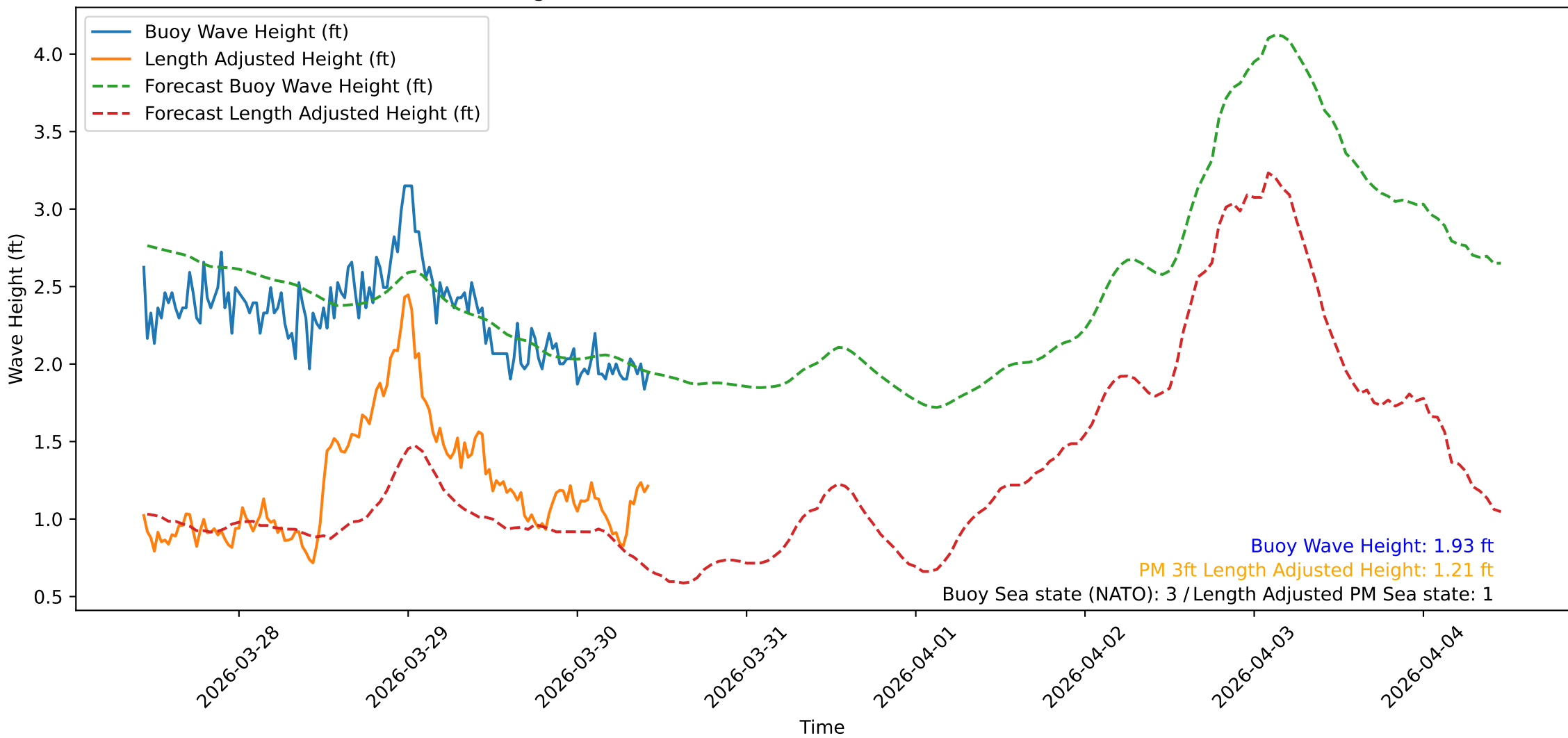
Wave Heights over Time for Oceanside Harbor at 2026-03-30 10:30:32
