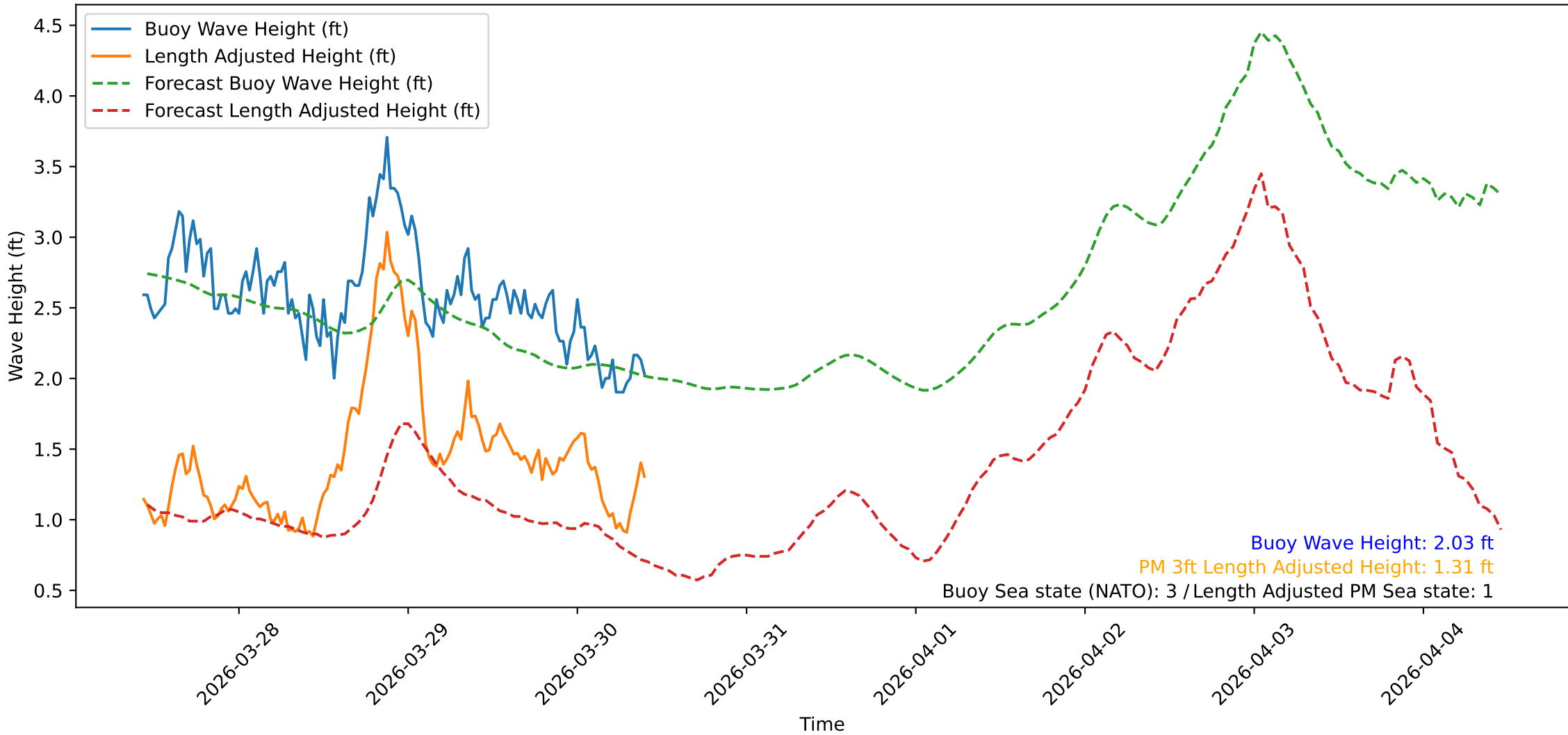
Wave Heights over Time for Green Beach at 2026-03-30 10:31:09
