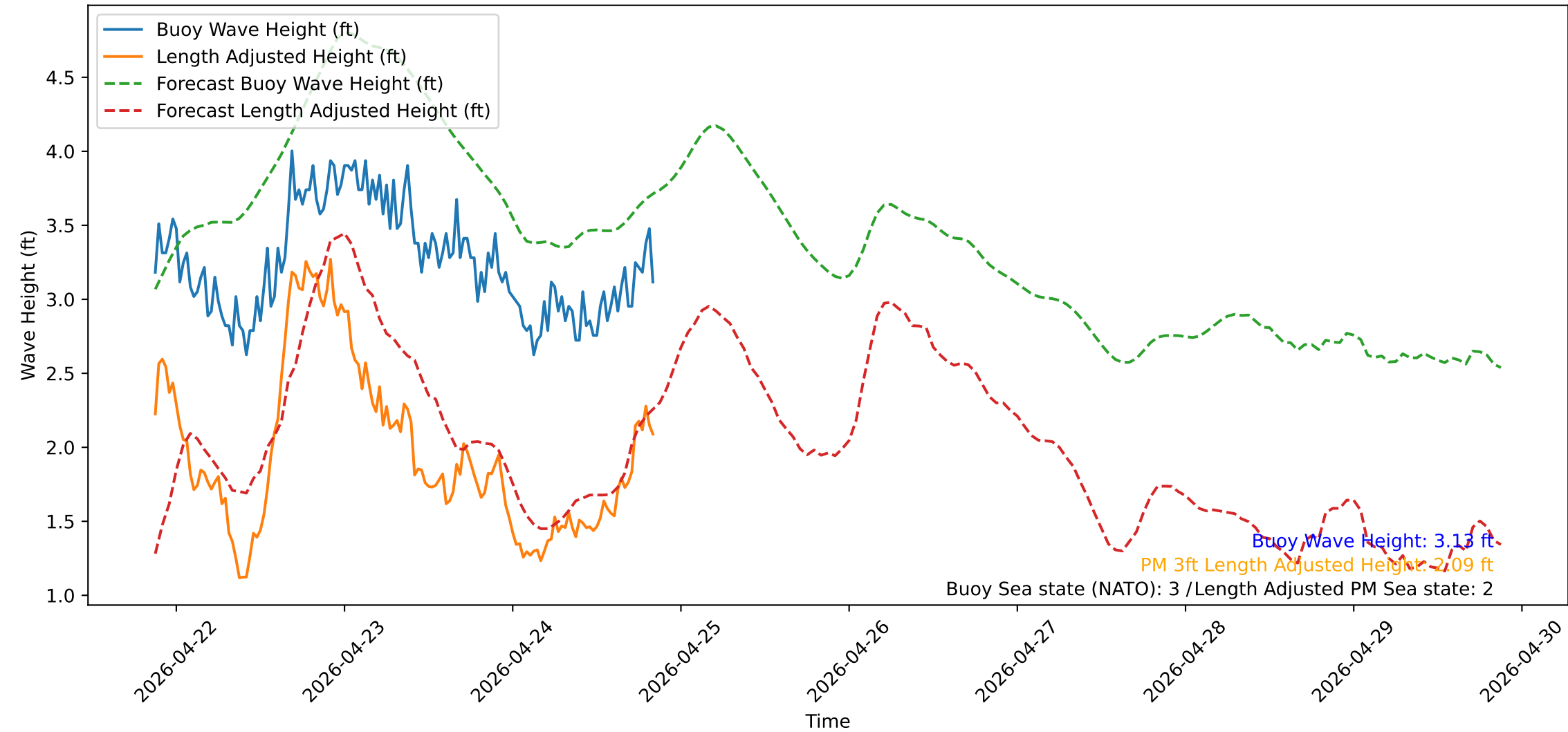
Wave Heights over Time for Green Beach at 2026-04-24 21:01:13
