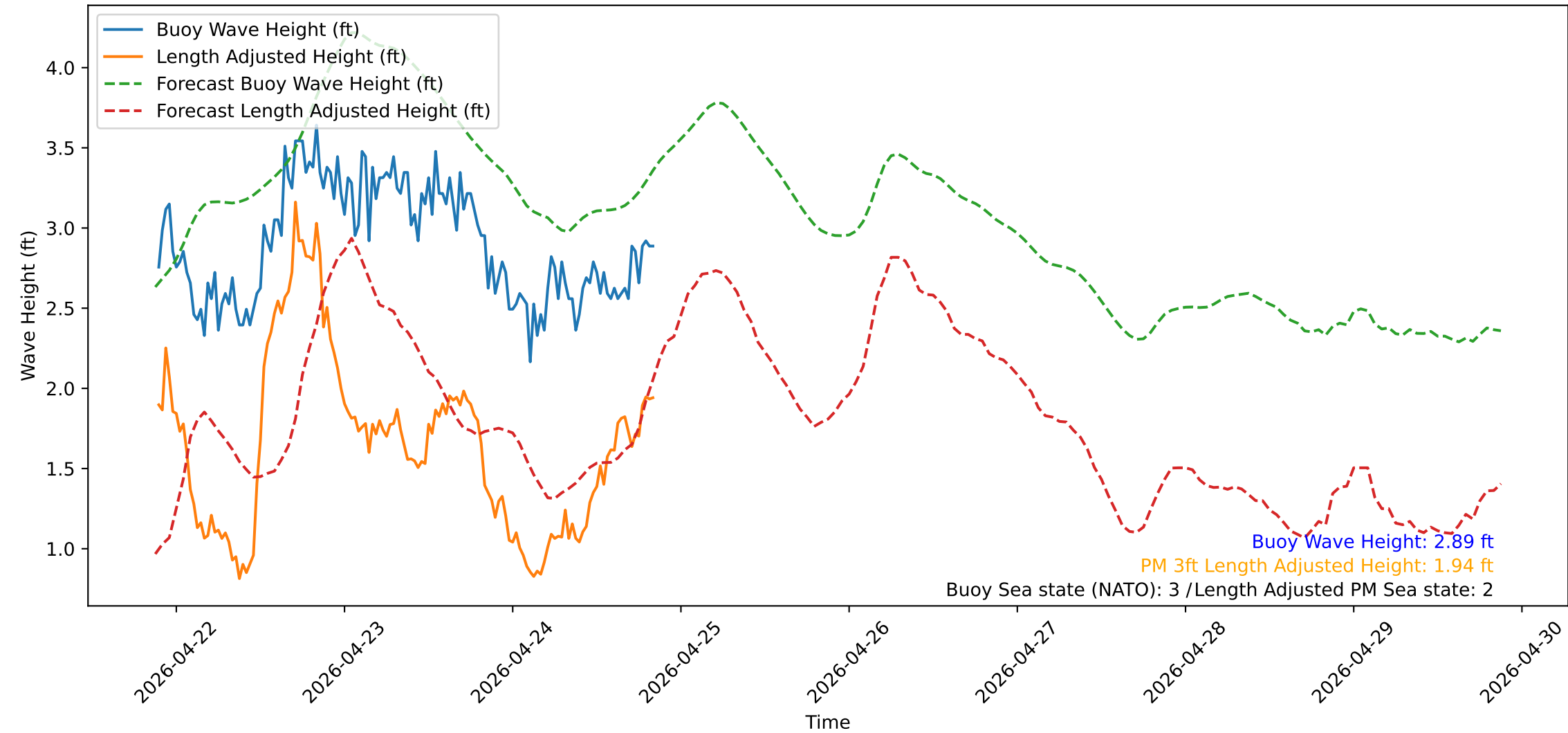
Wave Heights over Time for Red Beach at 2026-04-24 21:00:51
