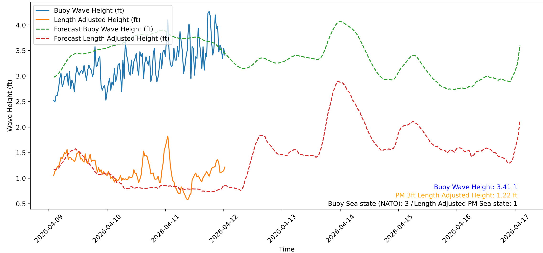
Wave Heights over Time for Red Beach at 2026-04-12 01:50:52
