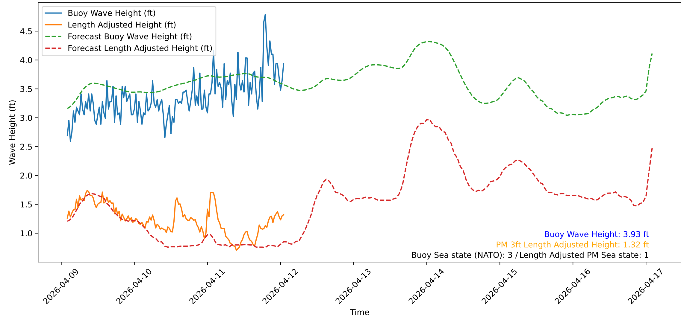
Wave Heights over Time for Oceanside Harbor at 2026-04-12 01:50:31
