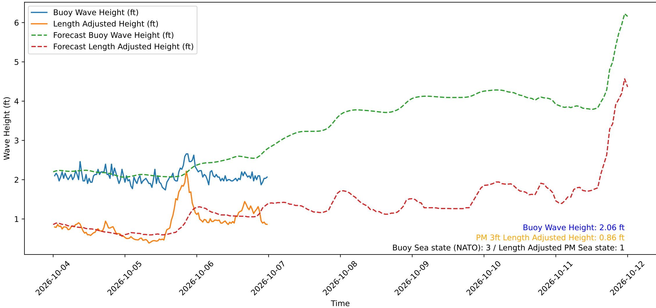
Wave Heights over Time for Red Beach at 2026-10-07 00:20:51
