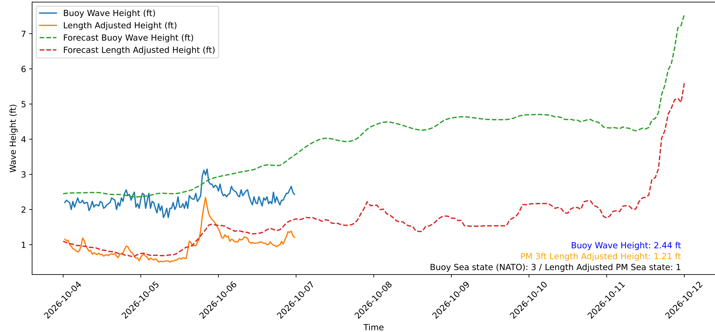
Wave Heights over Time for Green Beach at 2026-10-07 00:21:15
