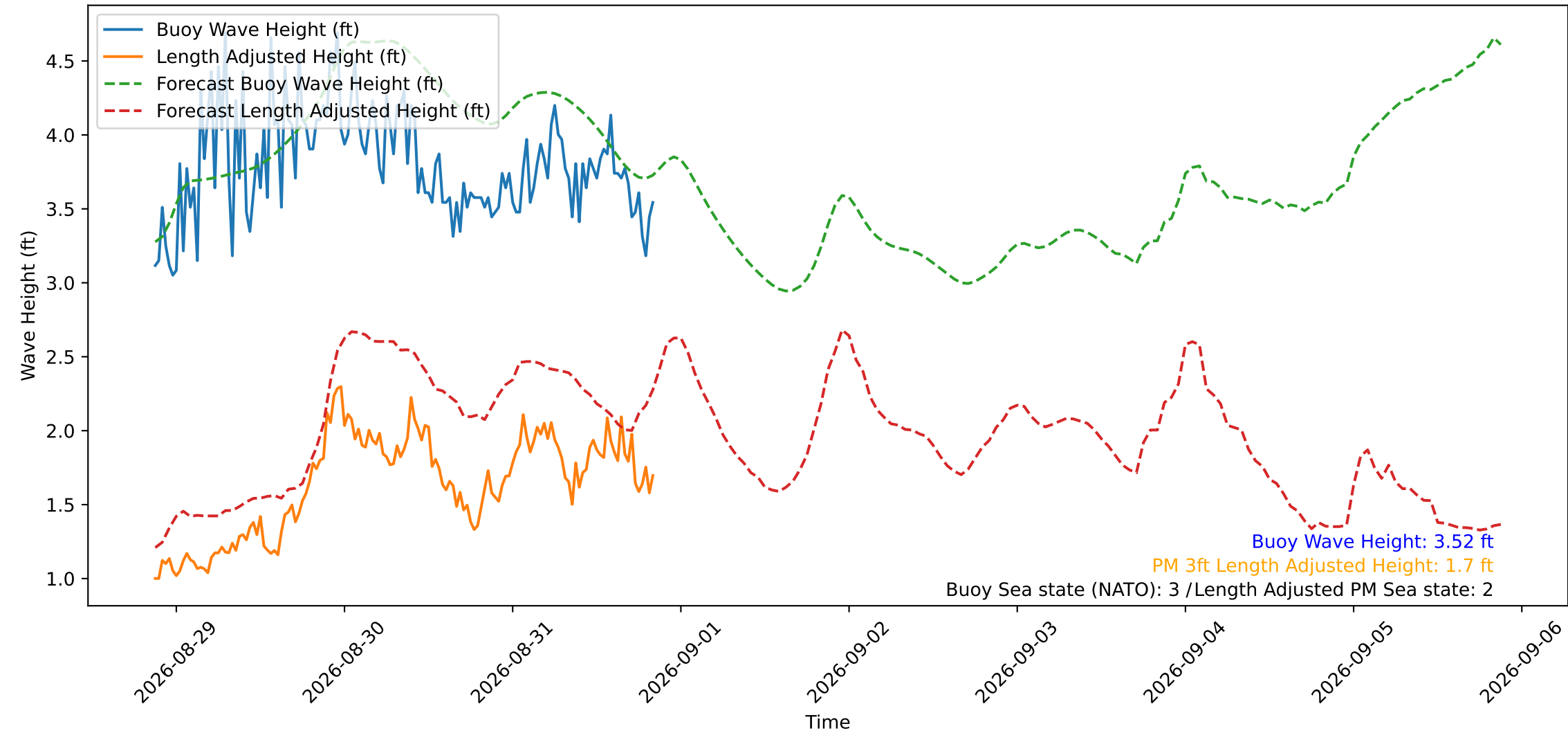
Wave Heights over Time for Red Beach at 2026-08-31 20:50:51
