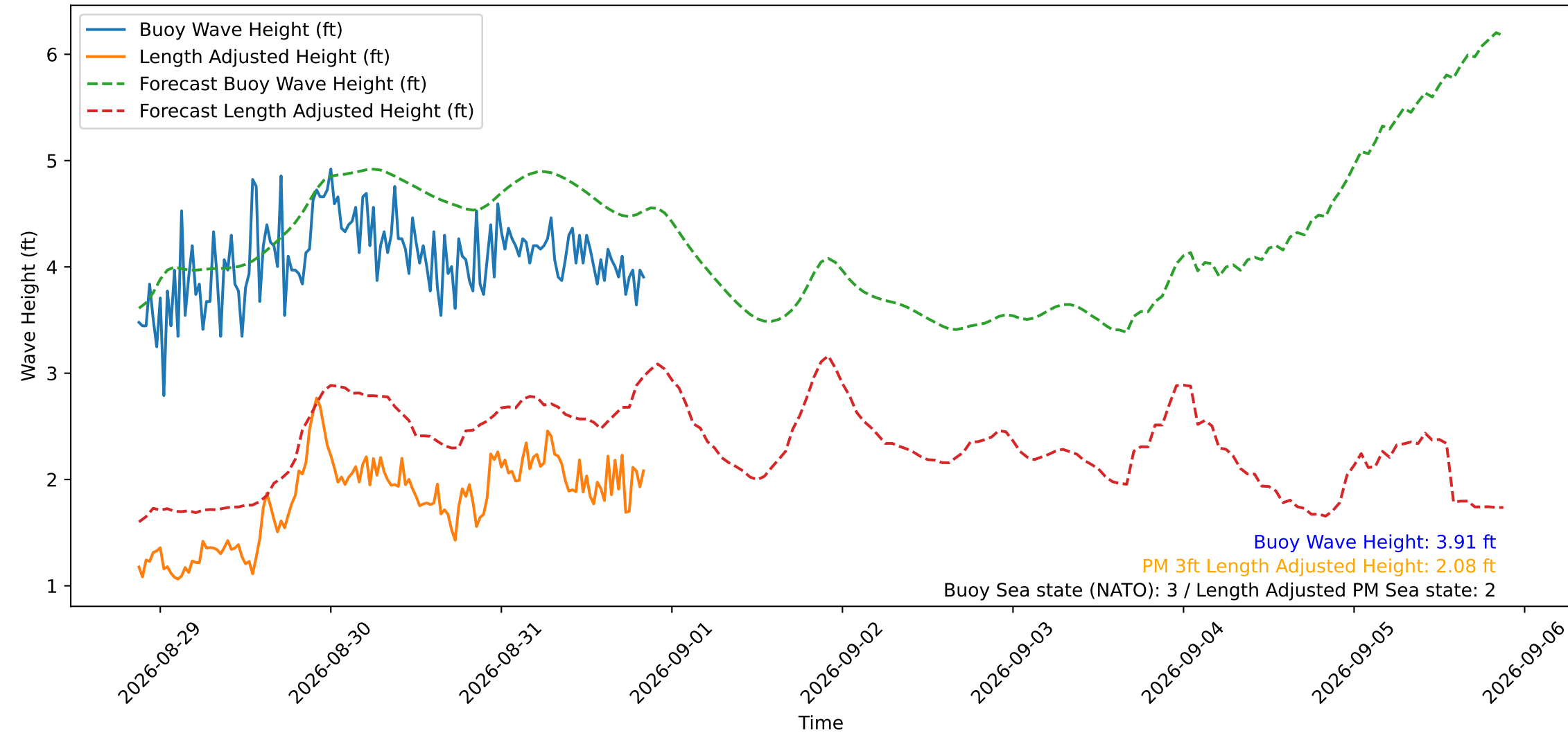
Wave Heights over Time for Green Beach at 2026-08-31 20:51:15
