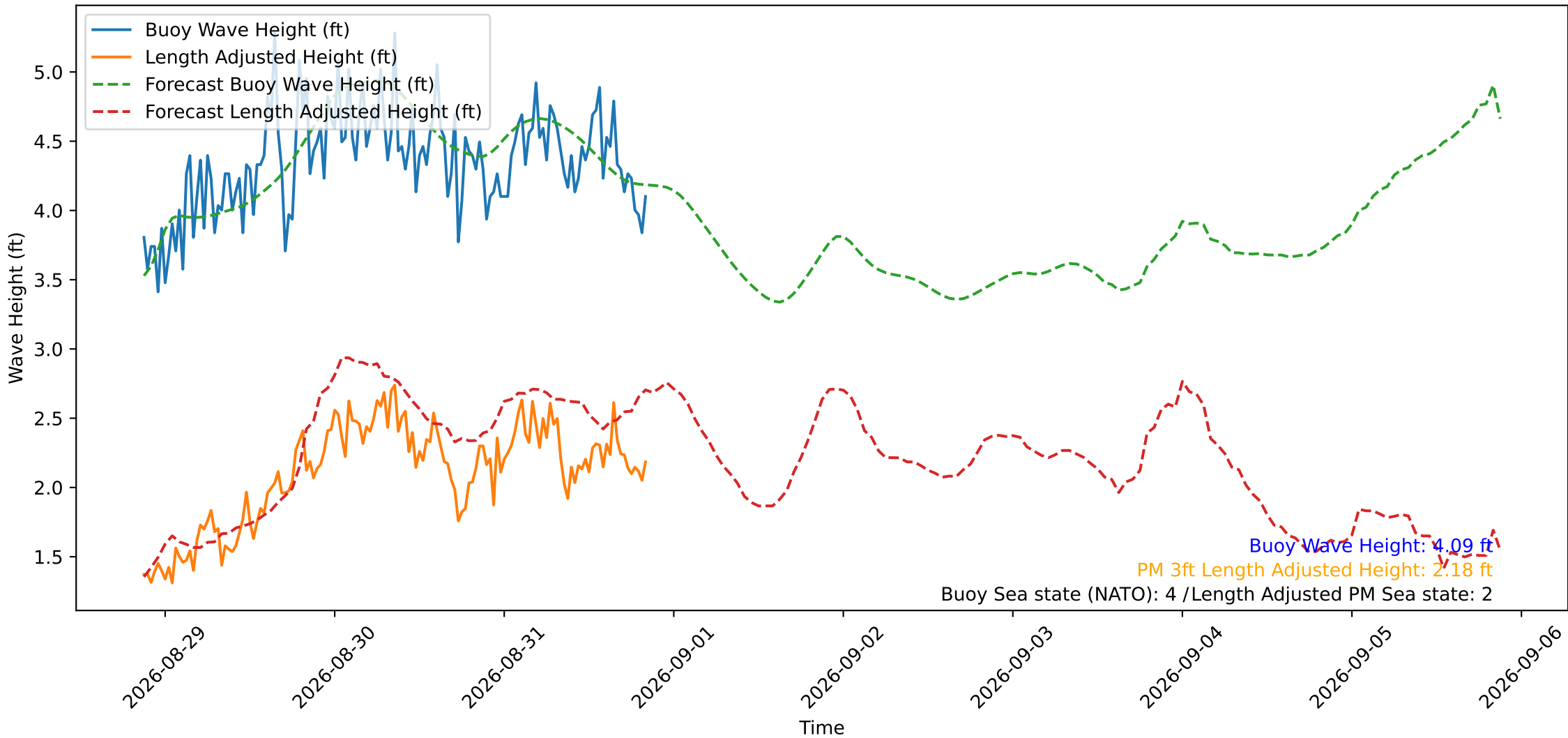
Wave Heights over Time for Oceanside Harbor at 2026-08-31 20:50:30
