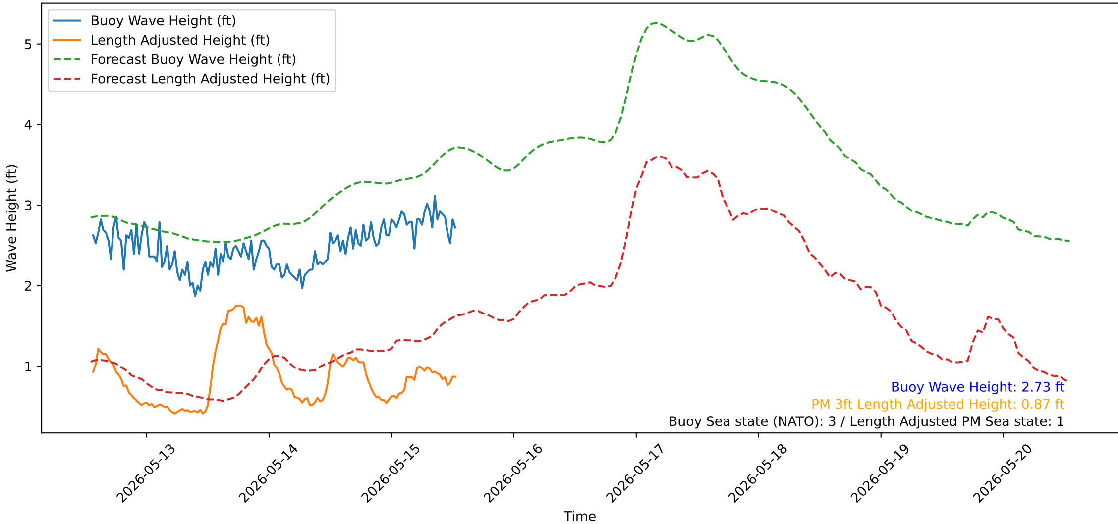
Wave Heights over Time for Red Beach at 2026-05-15 13:10:50
