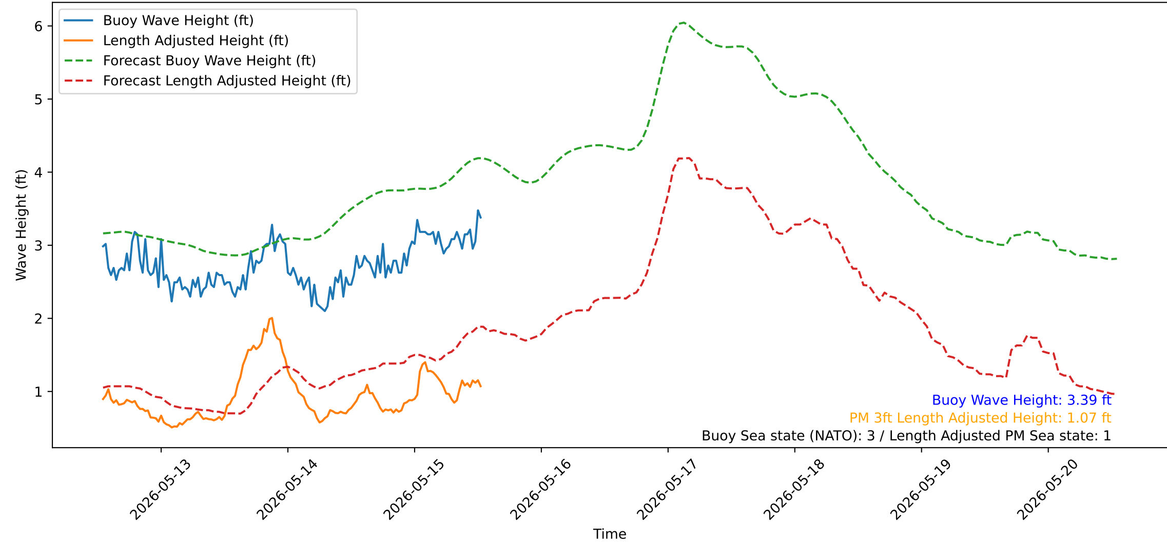
Wave Heights over Time for Green Beach at 2026-05-15 13:11:13
