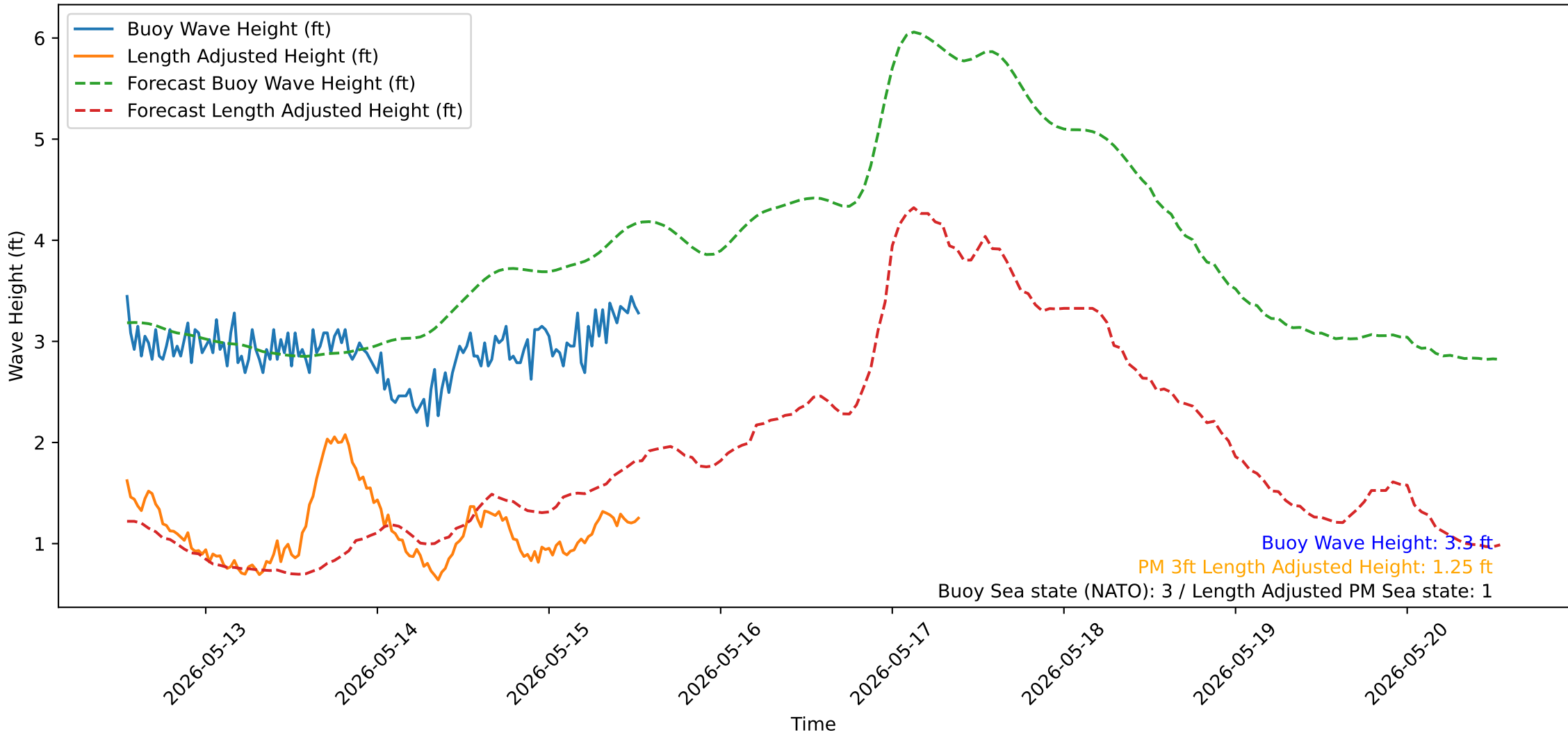
Wave Heights over Time for Oceanside Harbor at 2026-05-15 13:10:31
