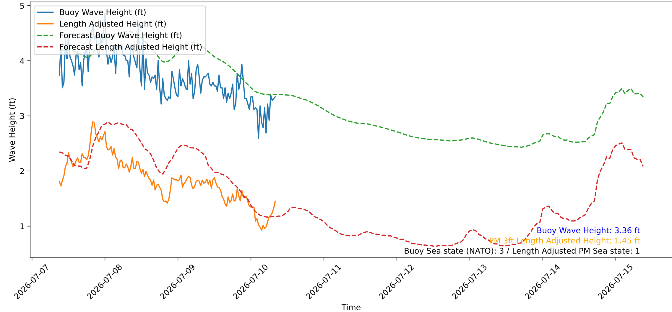
Wave Heights over Time for Red Beach at 2026-07-10 08:50:47
