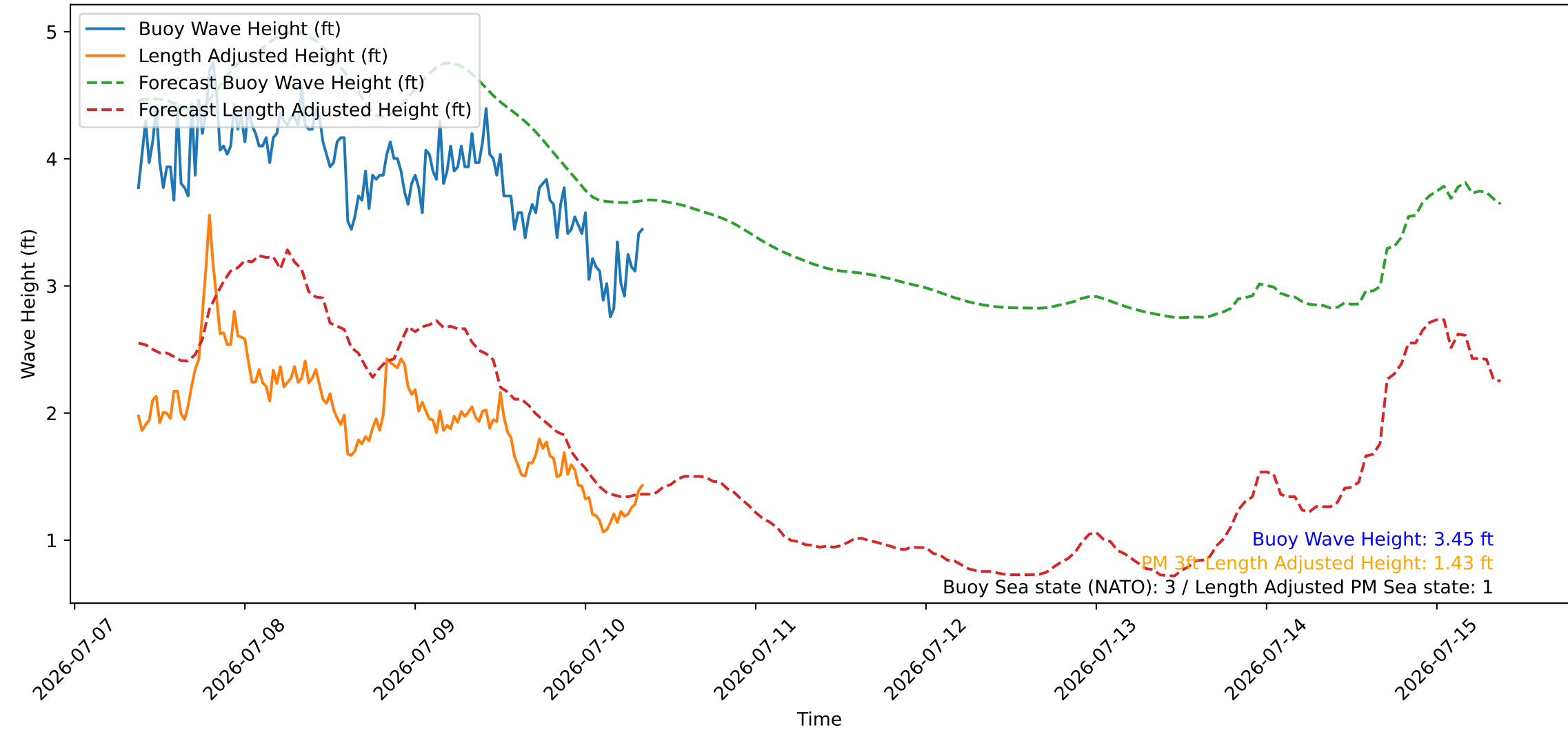
Wave Heights over Time for Green Beach at 2026-07-10 08:51:09
