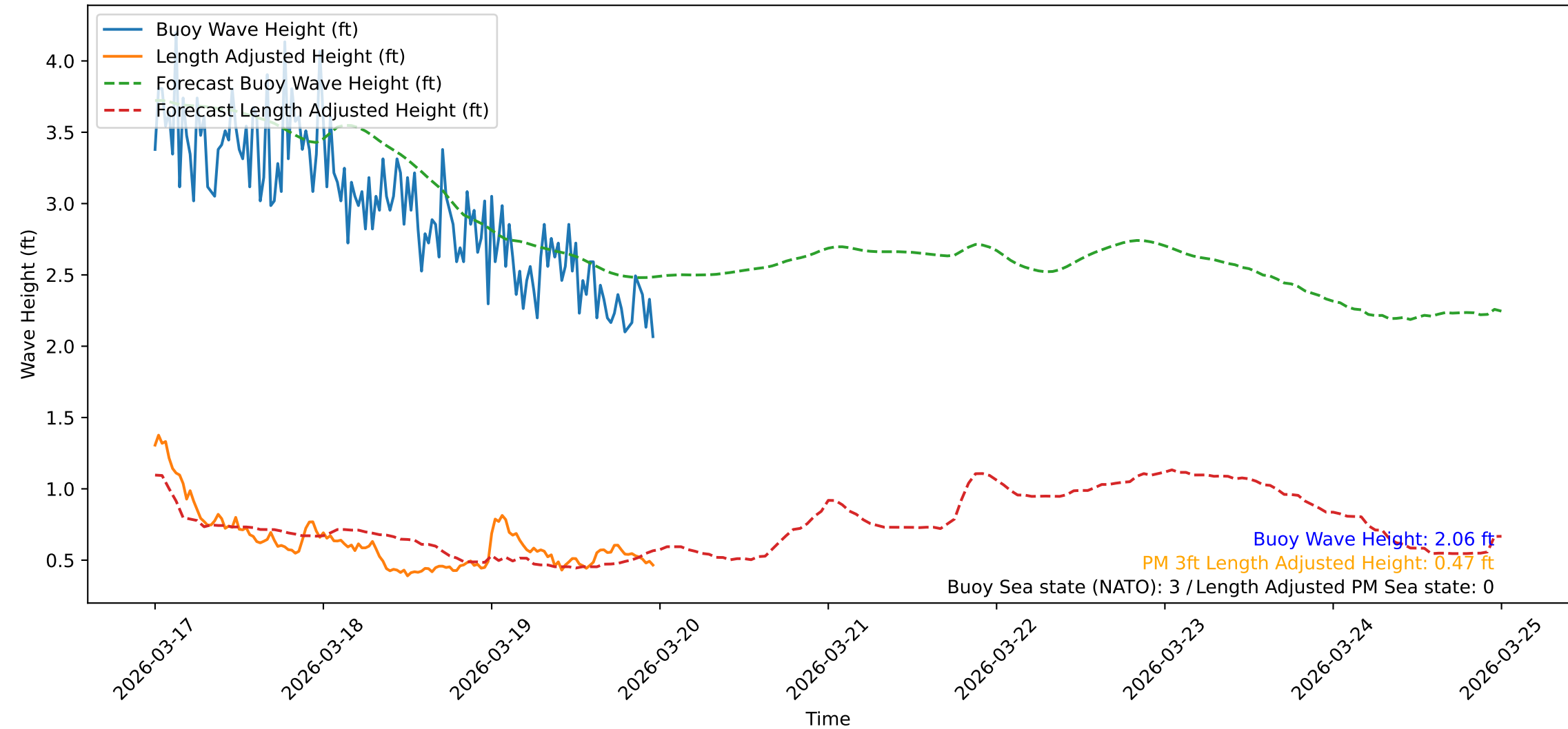
Wave Heights over Time for Green Beach at 2026-03-19 23:51:11
