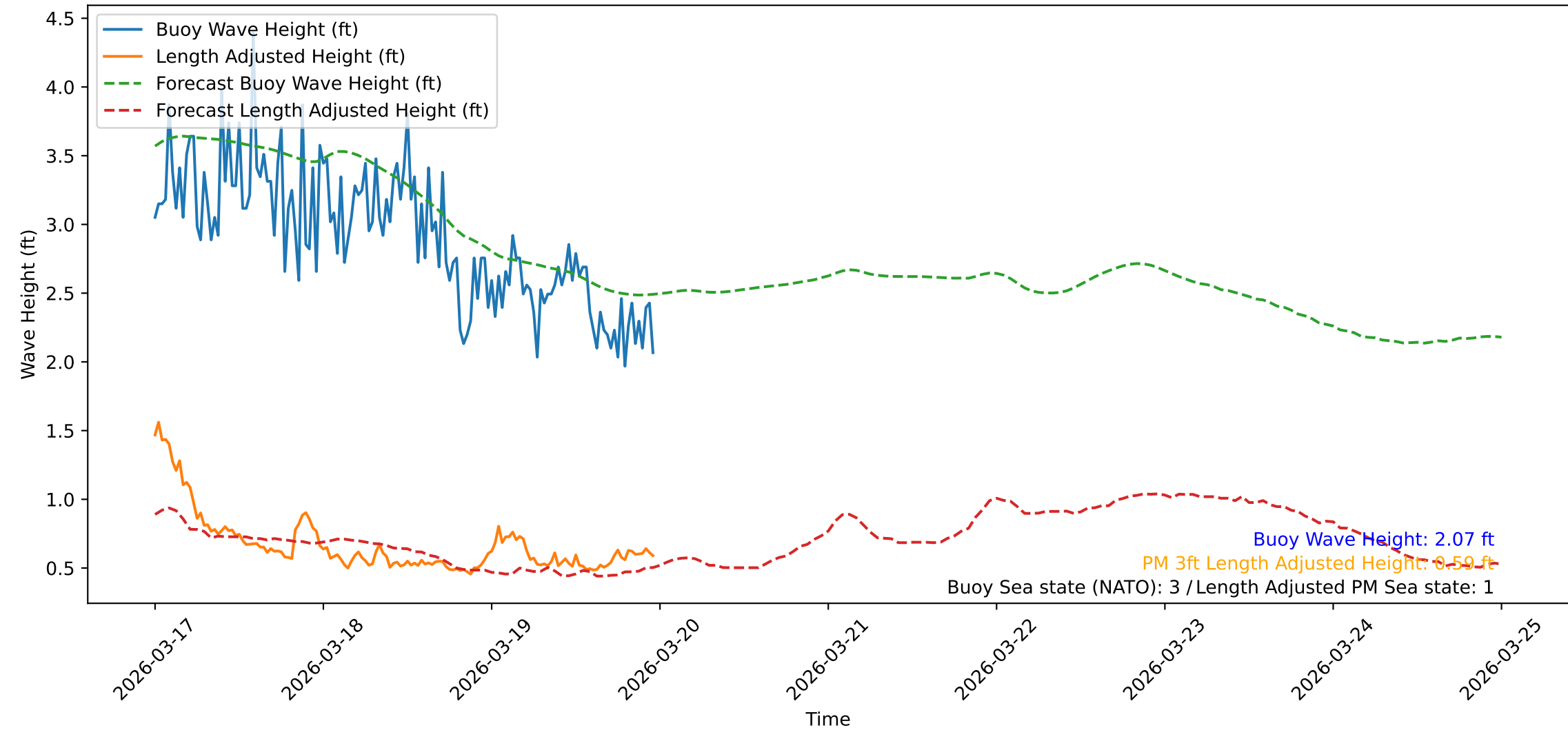
Wave Heights over Time for Oceanside Harbor at 2026-03-19 23:50:32
