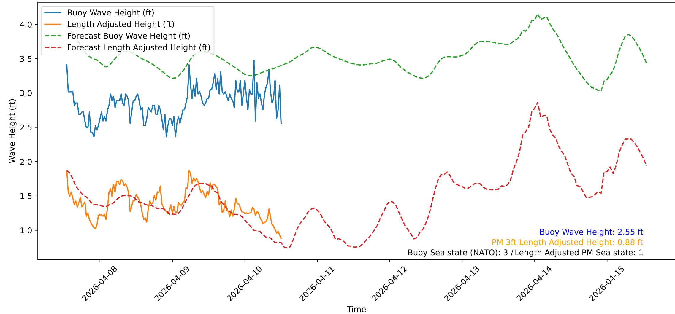
Wave Heights over Time for Green Beach at 2026-04-10 13:01:12
