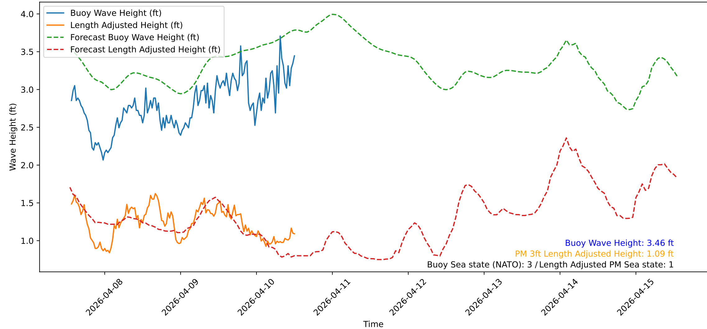
Wave Heights over Time for Red Beach at 2026-04-10 13:00:50
