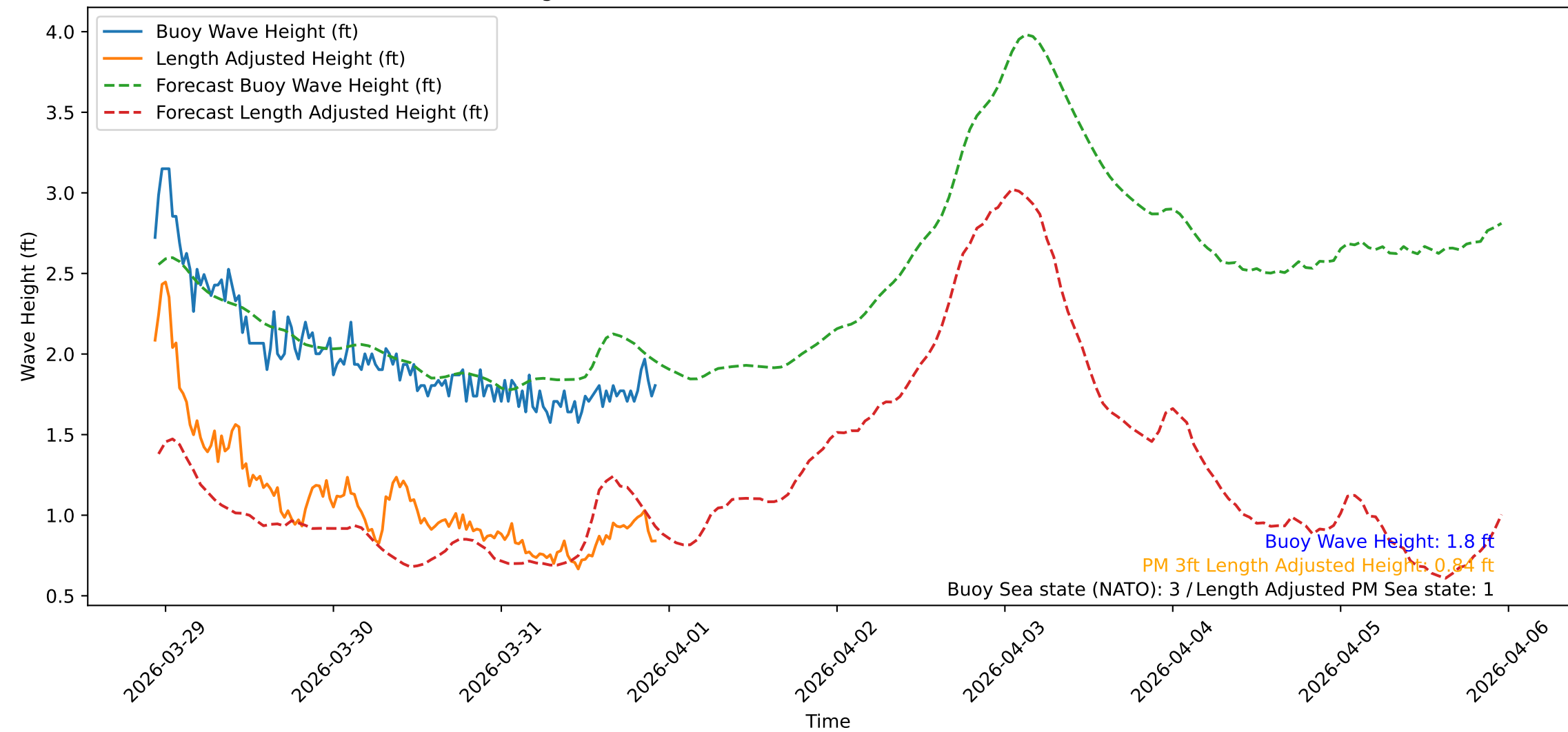
Wave Heights over Time for Oceanside Harbor at 2026-03-31 22:40:31
