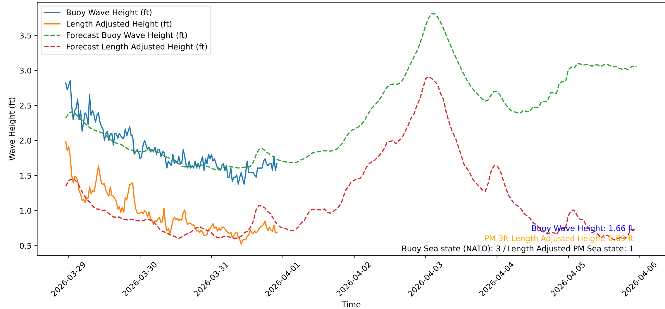
Wave Heights over Time for Red Beach at 2026-03-31 22:40:47
