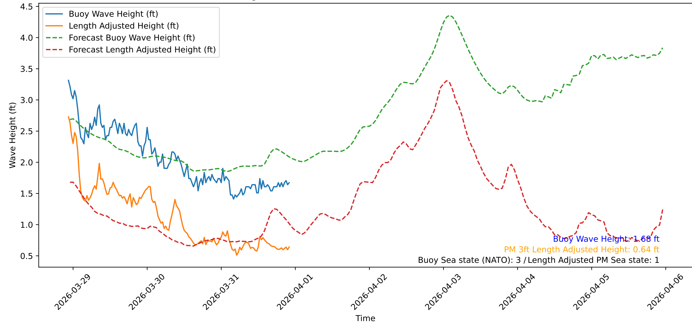
Wave Heights over Time for Green Beach at 2026-03-31 22:41:09
