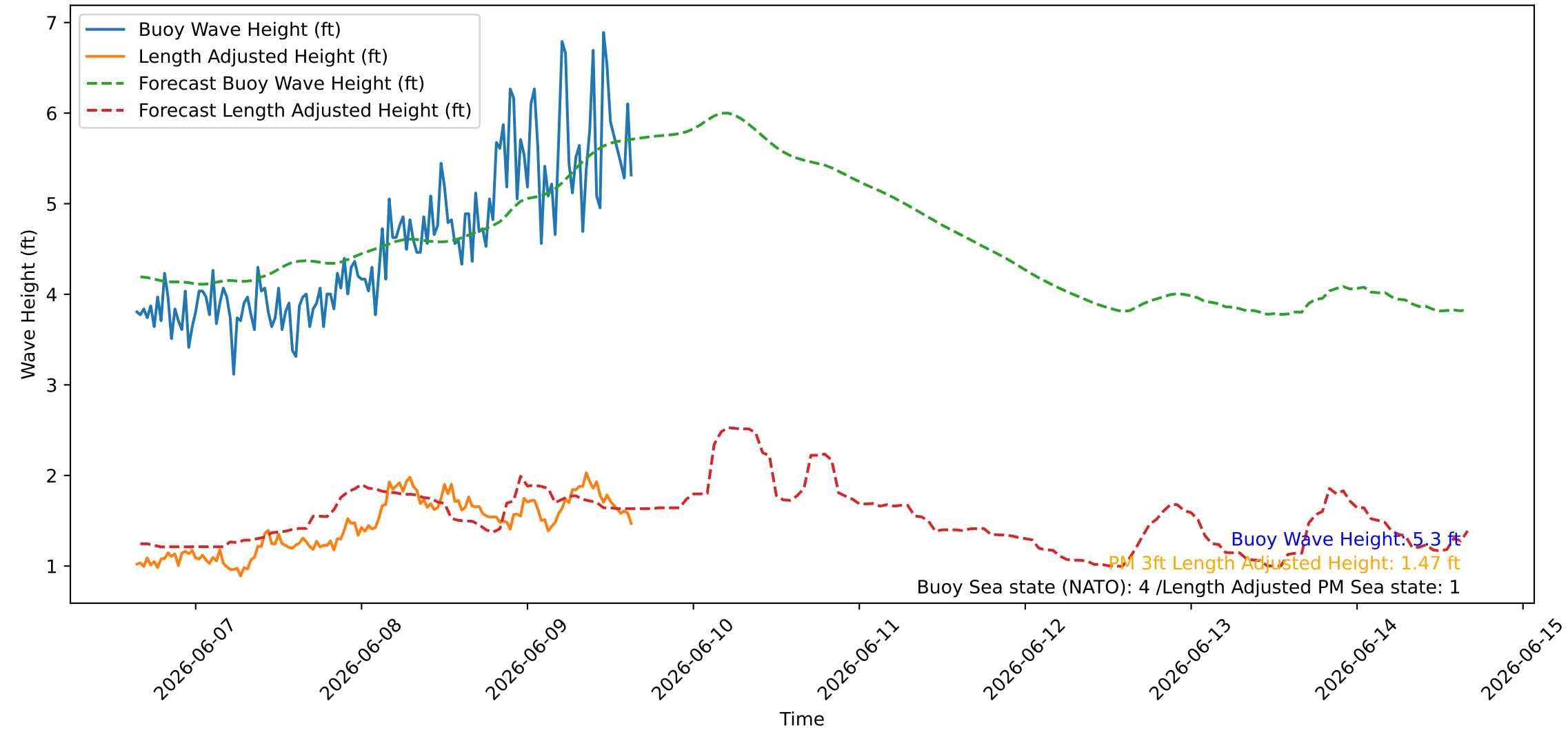
Wave Heights over Time for Green Beach at 2026-06-09 15:41:08
