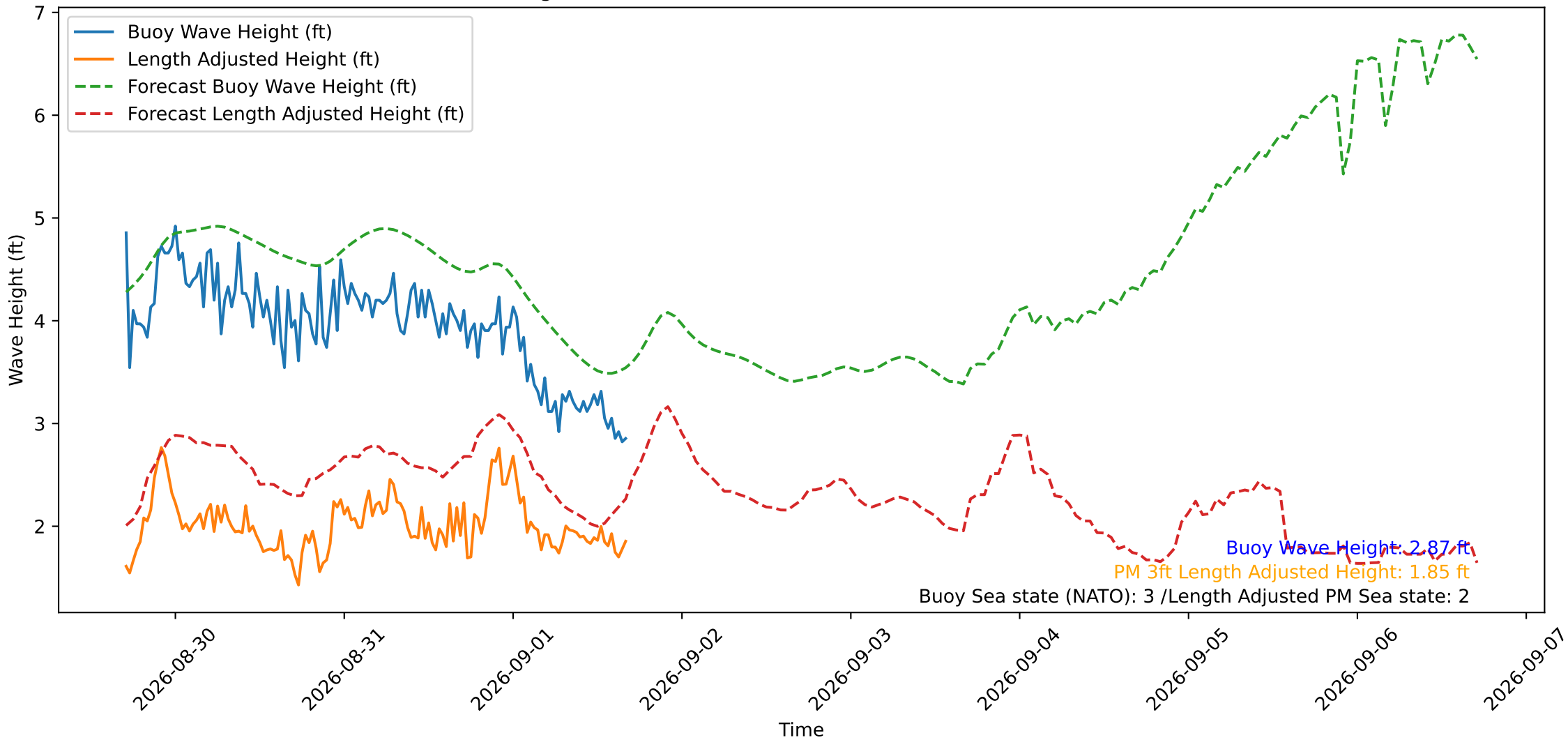
Wave Heights over Time for Green Beach at 2026-09-01 16:41:12
