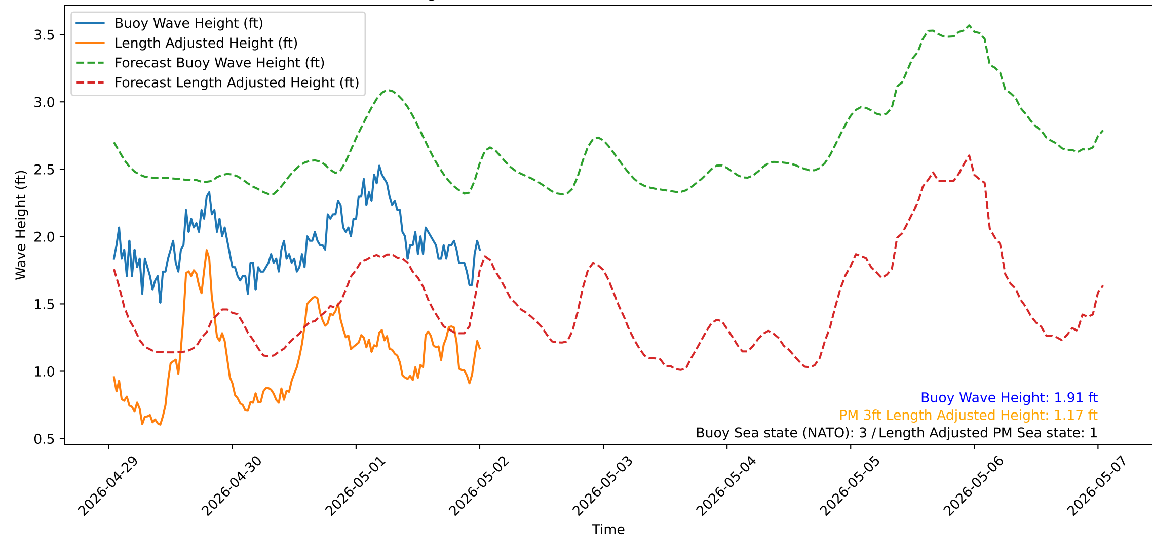
Wave Heights over Time for Red Beach at 2026-05-02 00:50:52
