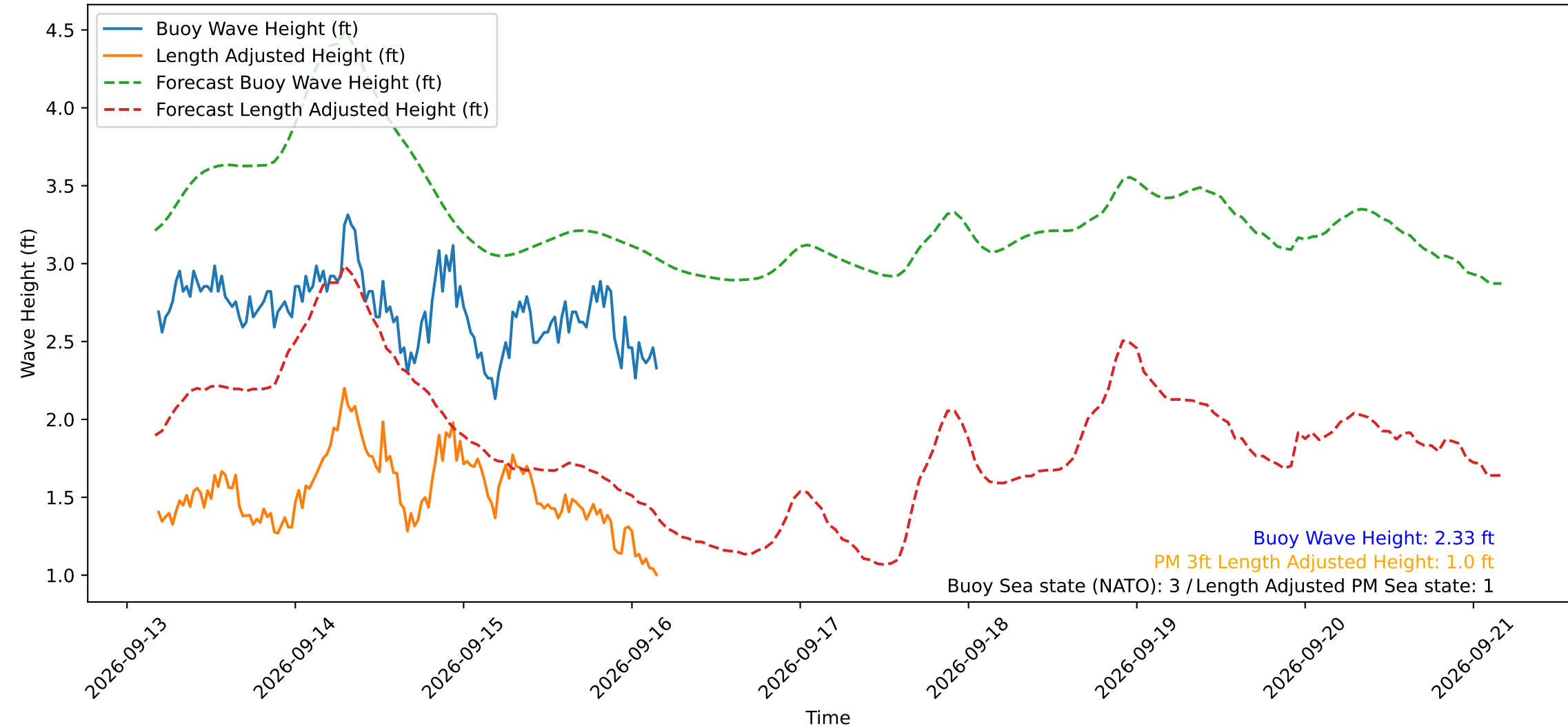
Wave Heights over Time for Green Beach at 2026-09-16 04:21:14
