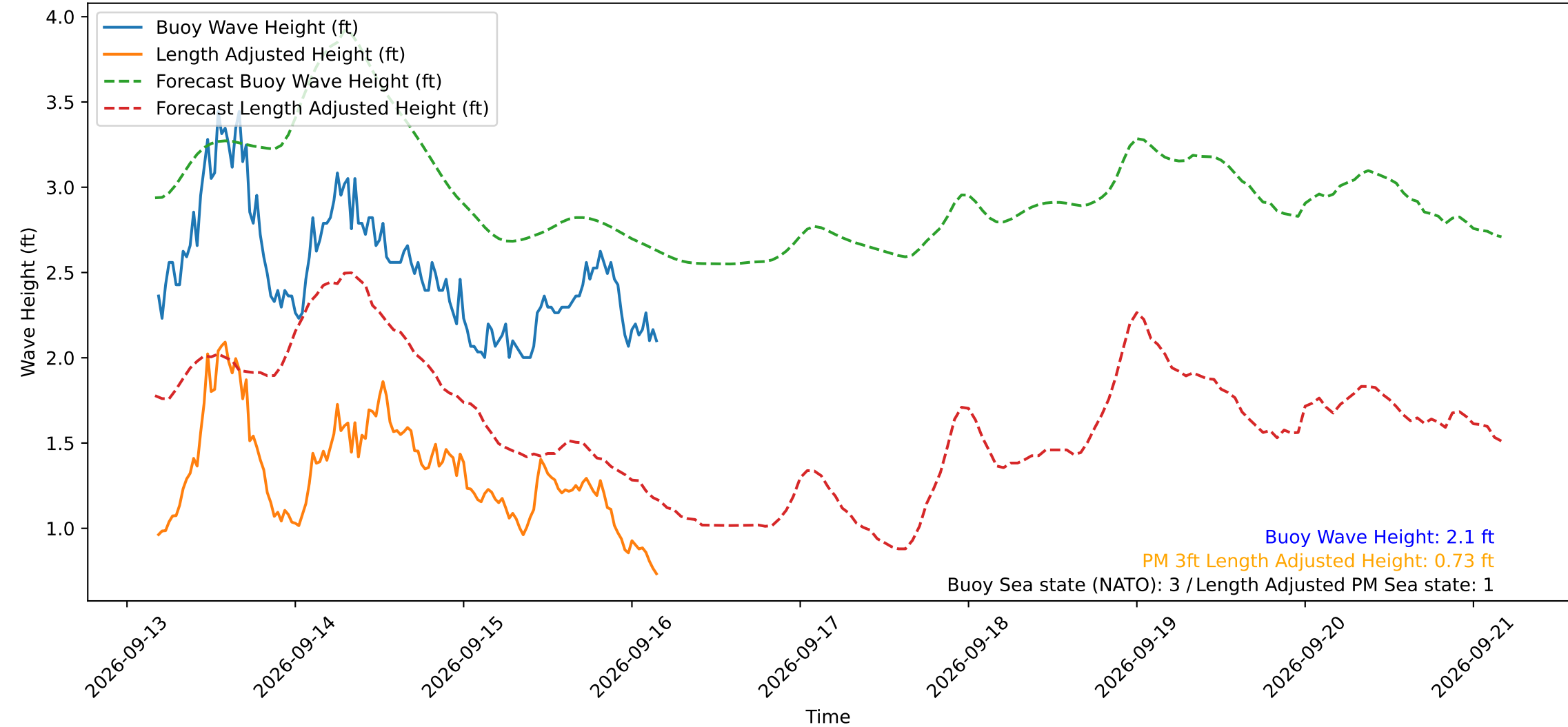
Wave Heights over Time for Red Beach at 2026-09-16 04:20:50
