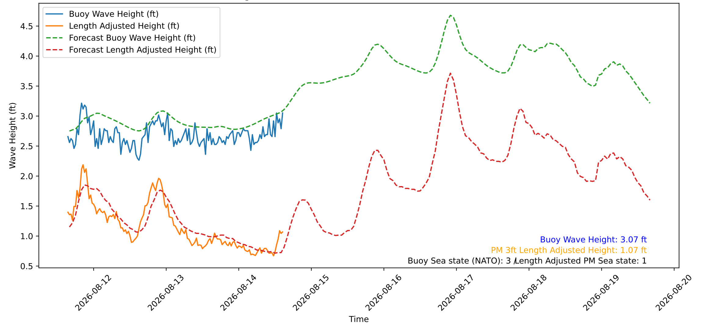
Wave Heights over Time for Green Beach at 2026-08-14 15:31:08
