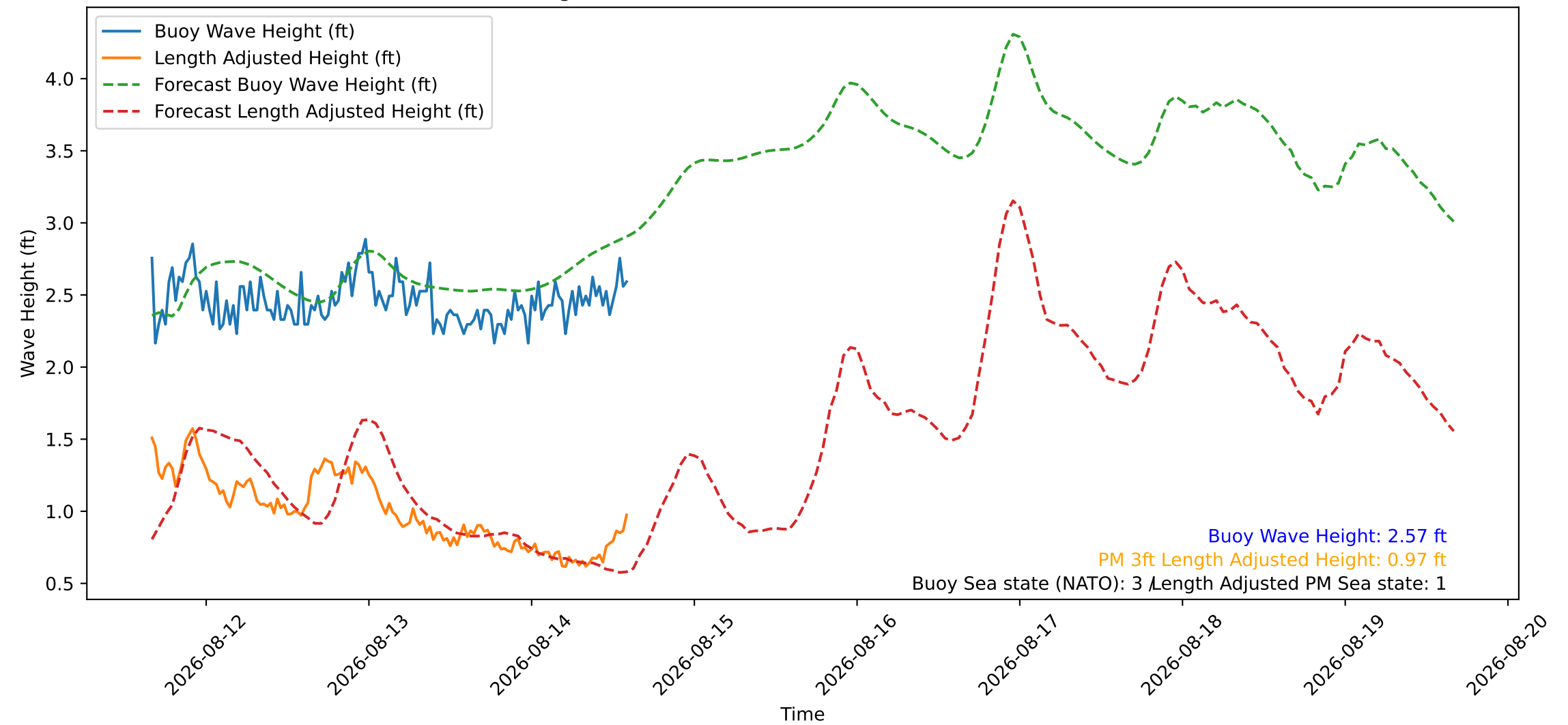
Wave Heights over Time for Red Beach at 2026-08-14 15:30:45
