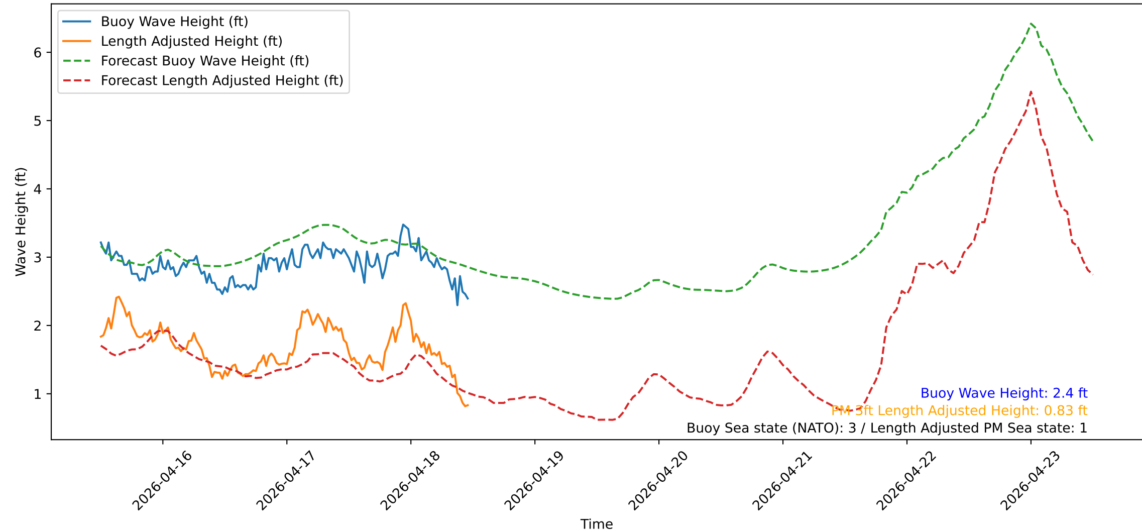
Wave Heights over Time for Green Beach at 2026-04-18 12:01:12
