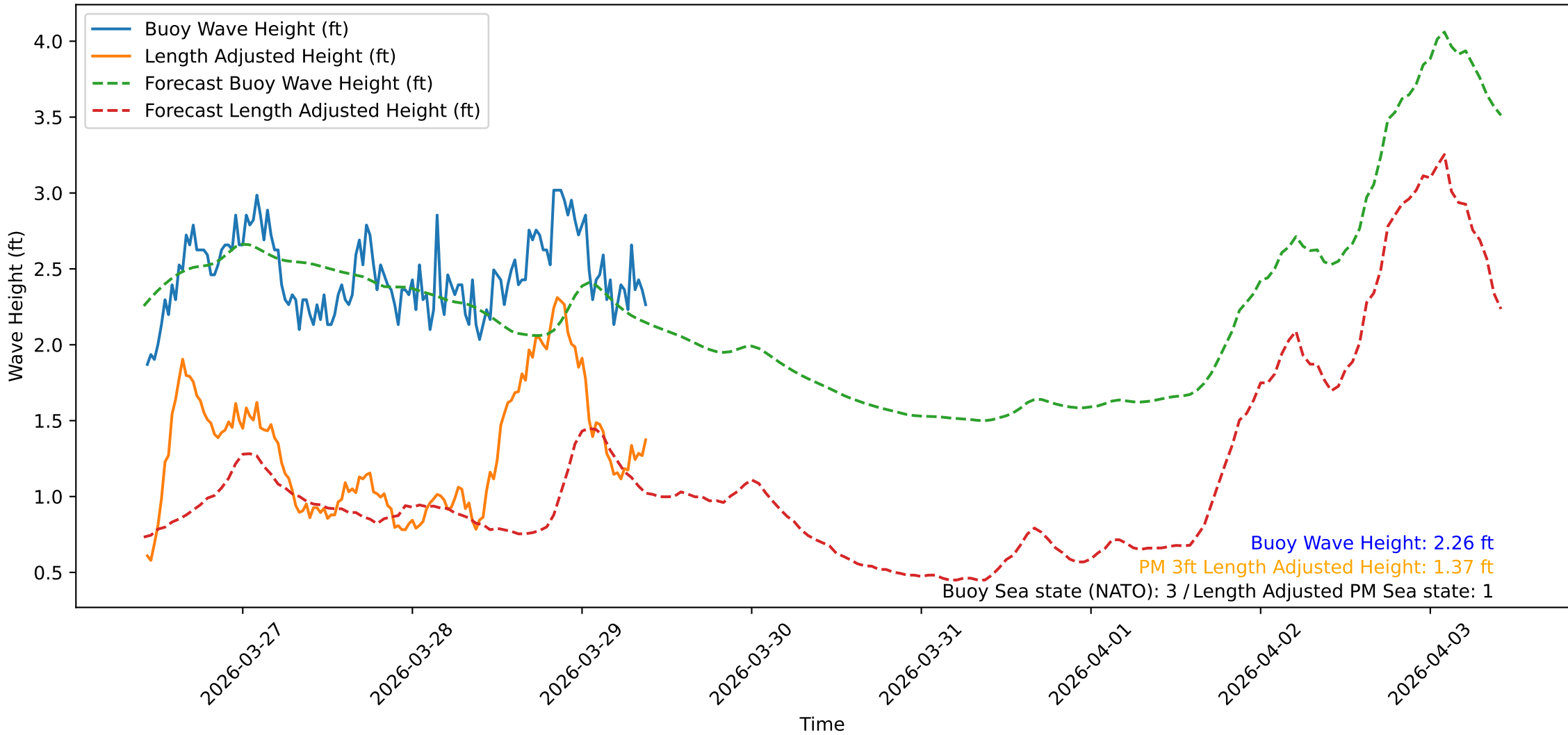
Wave Heights over Time for Red Beach at 2026-03-29 10:00:47
