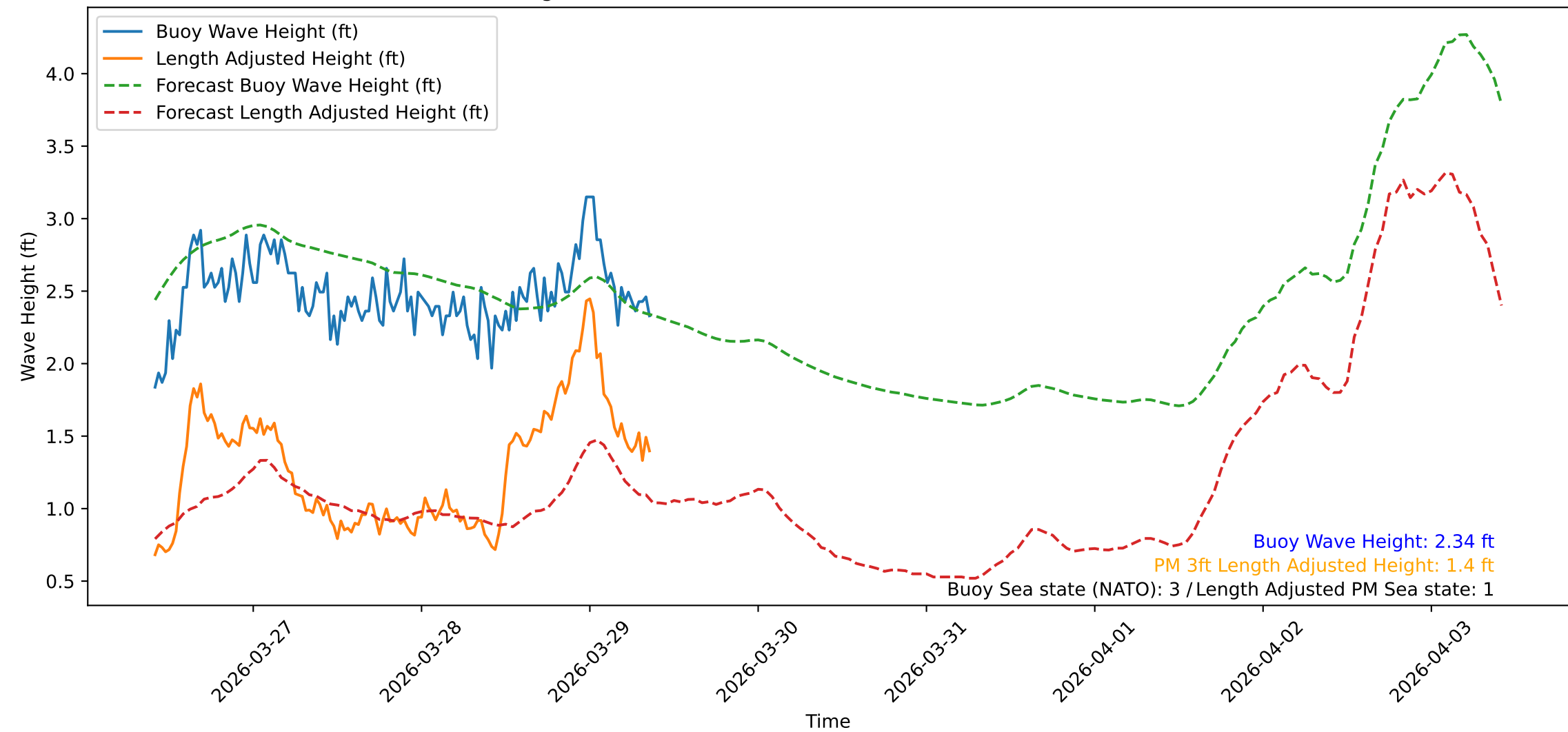
Wave Heights over Time for Oceanside Harbor at 2026-03-29 10:00:31
