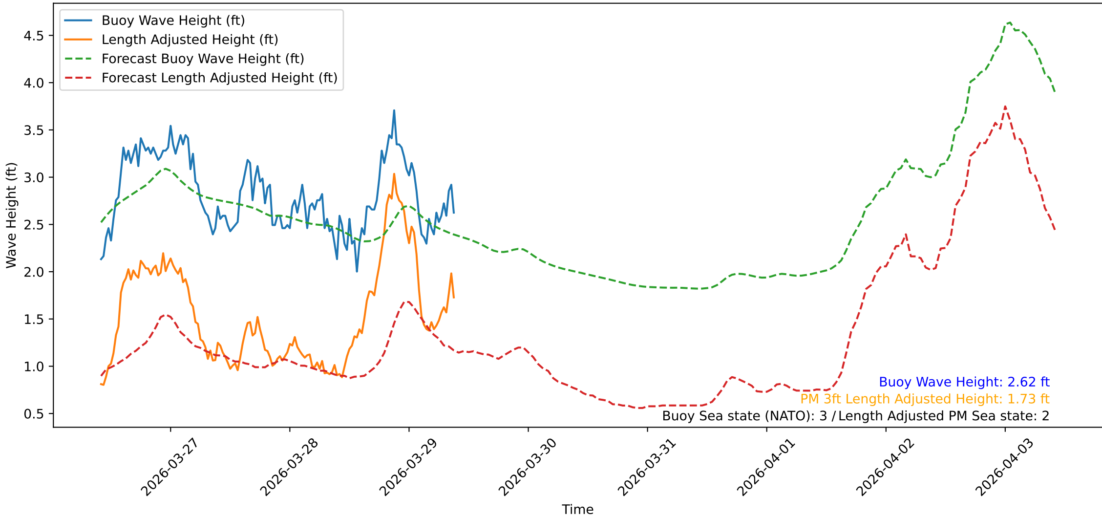
Wave Heights over Time for Green Beach at 2026-03-29 10:01:10
