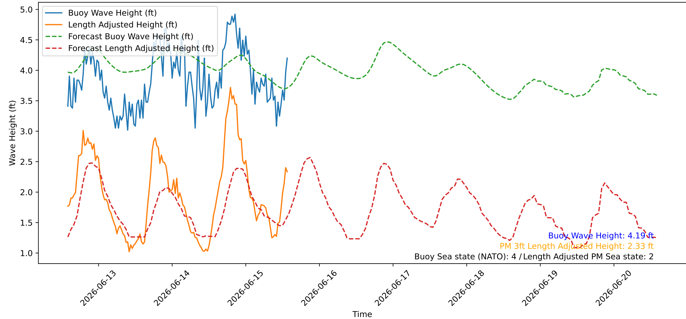
Wave Heights over Time for Green Beach at 2026-06-15 14:11:07
