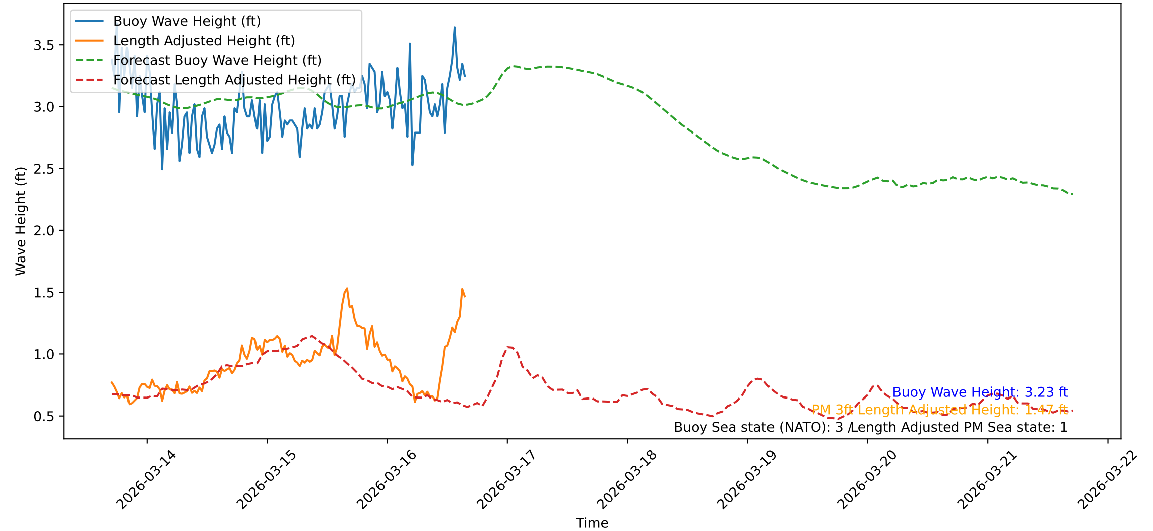
Wave Heights over Time for Red Beach at 2026-03-16 16:31:07
