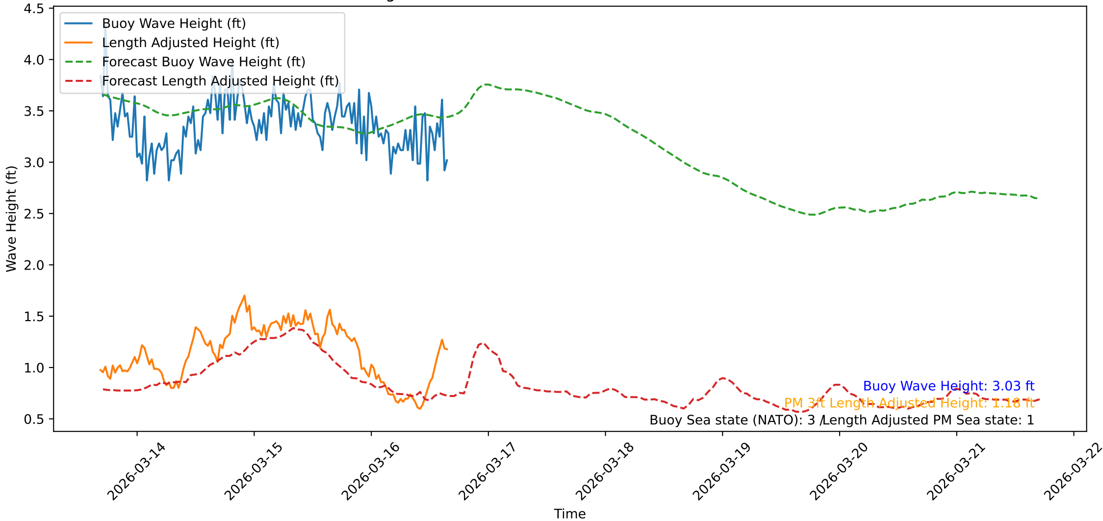
Wave Heights over Time for Green Beach at 2026-03-16 16:31:46
