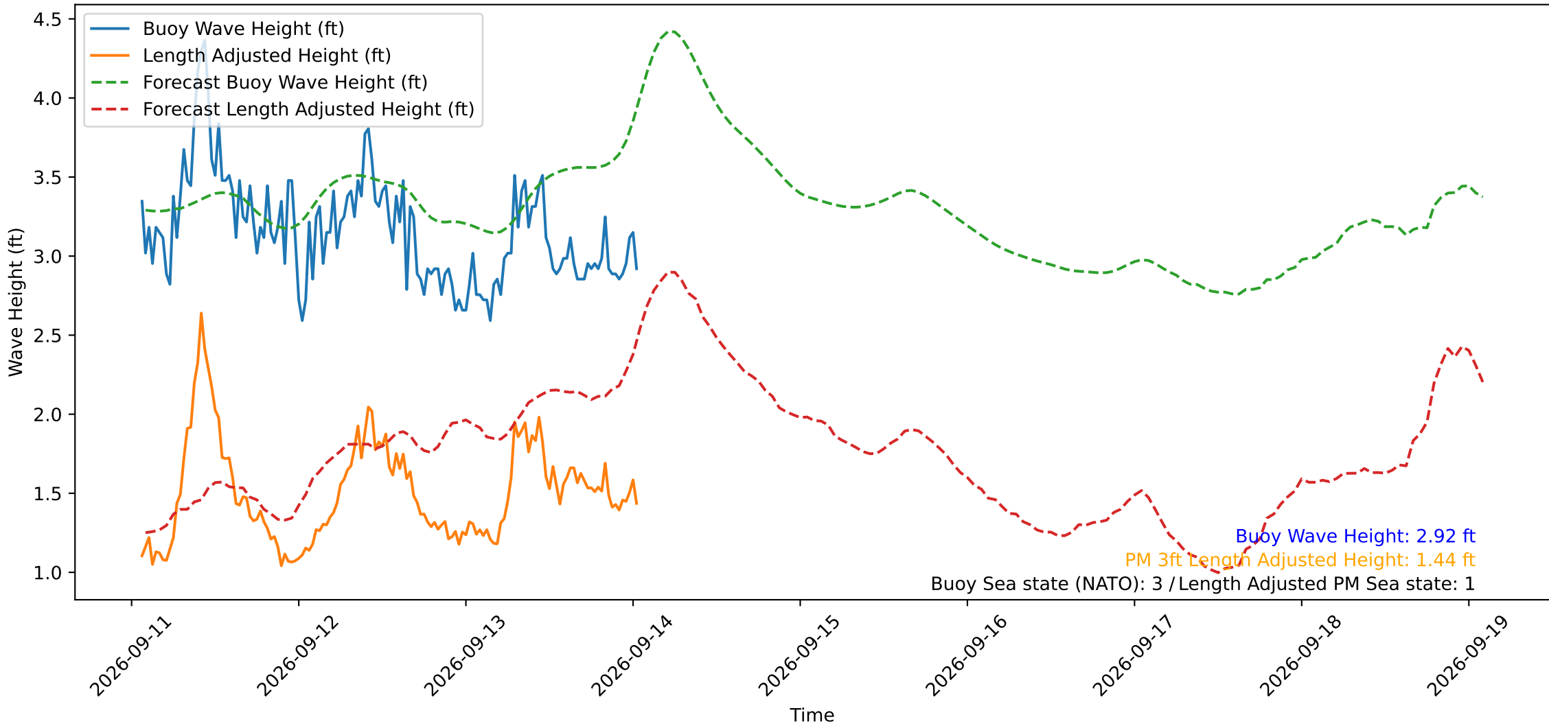
Wave Heights over Time for Oceanside Harbor at 2026-09-14 01:30:29
