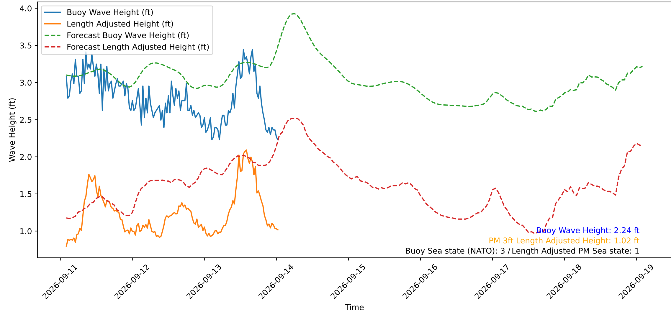
Wave Heights over Time for Red Beach at 2026-09-14 01:30:49
