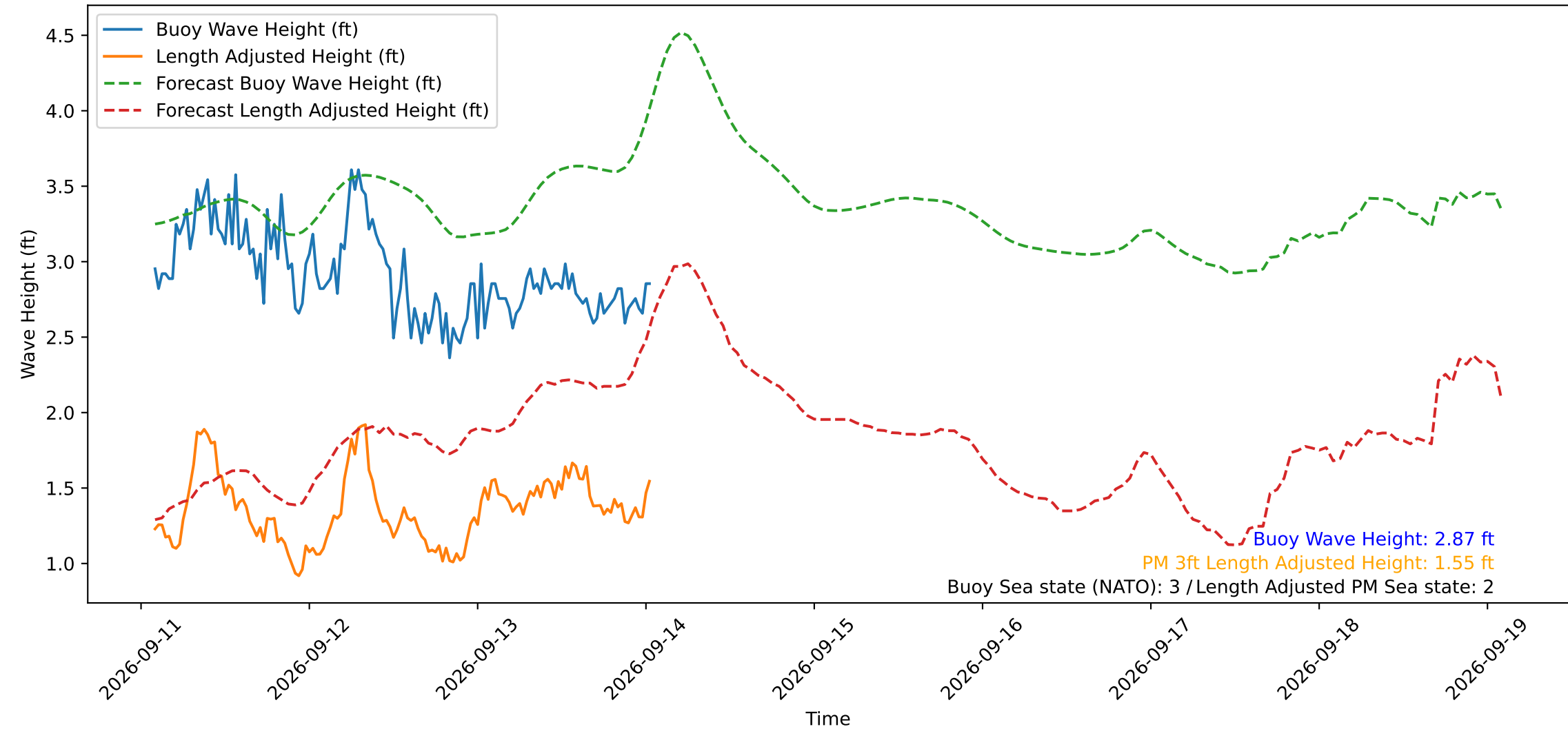
Wave Heights over Time for Green Beach at 2026-09-14 01:31:12
