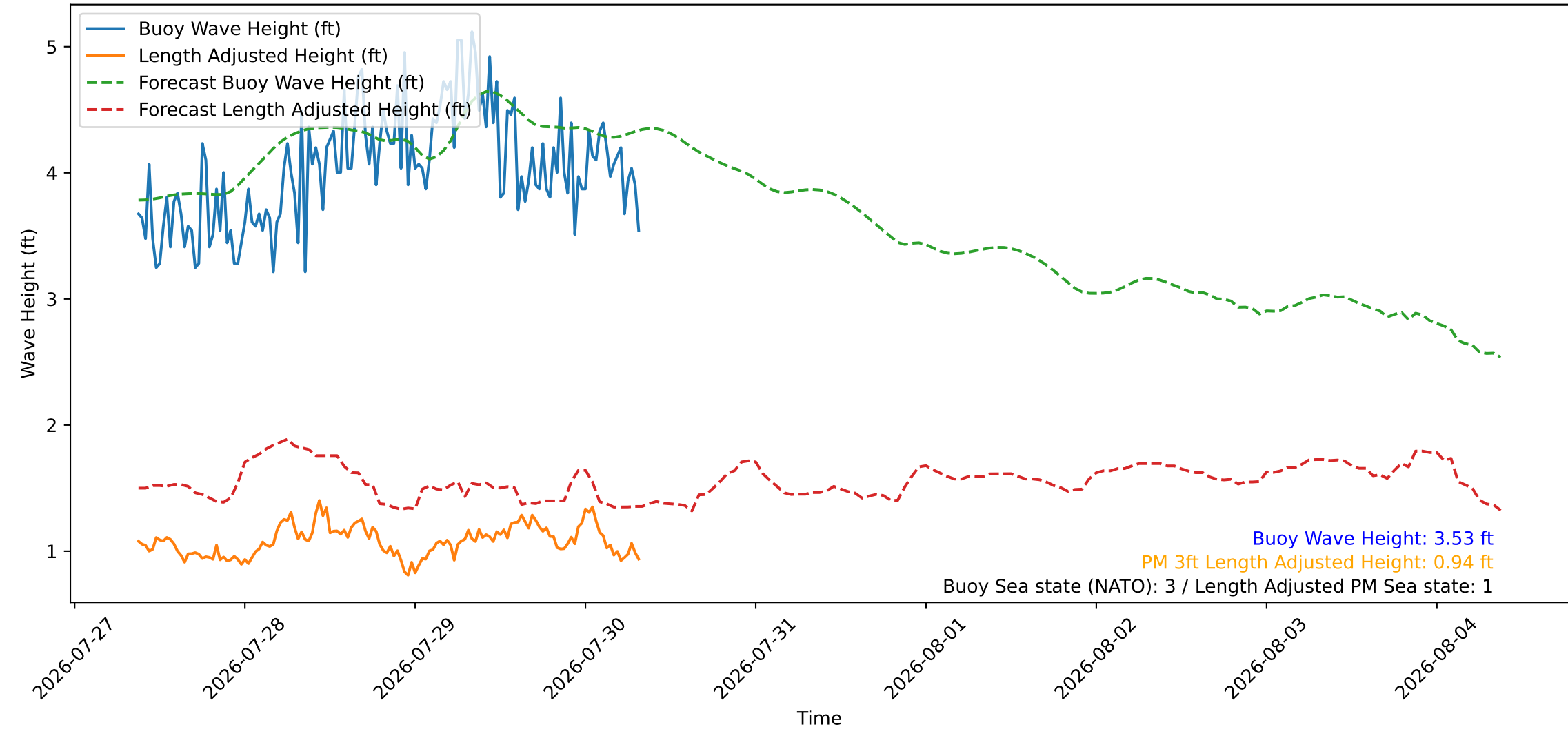
Wave Heights over Time for Red Beach at 2026-07-30 08:30:46
