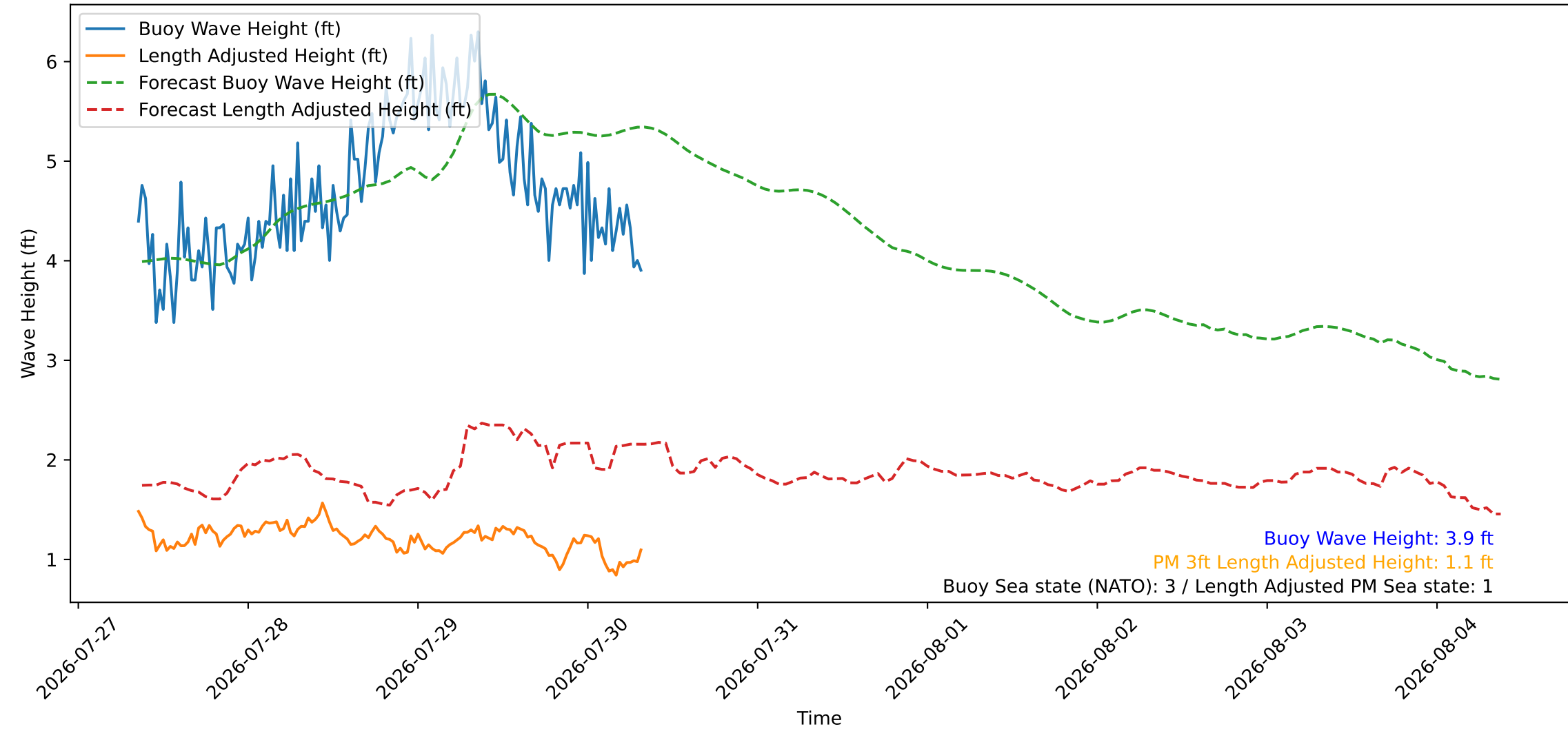
Wave Heights over Time for Green Beach at 2026-07-30 08:31:08
