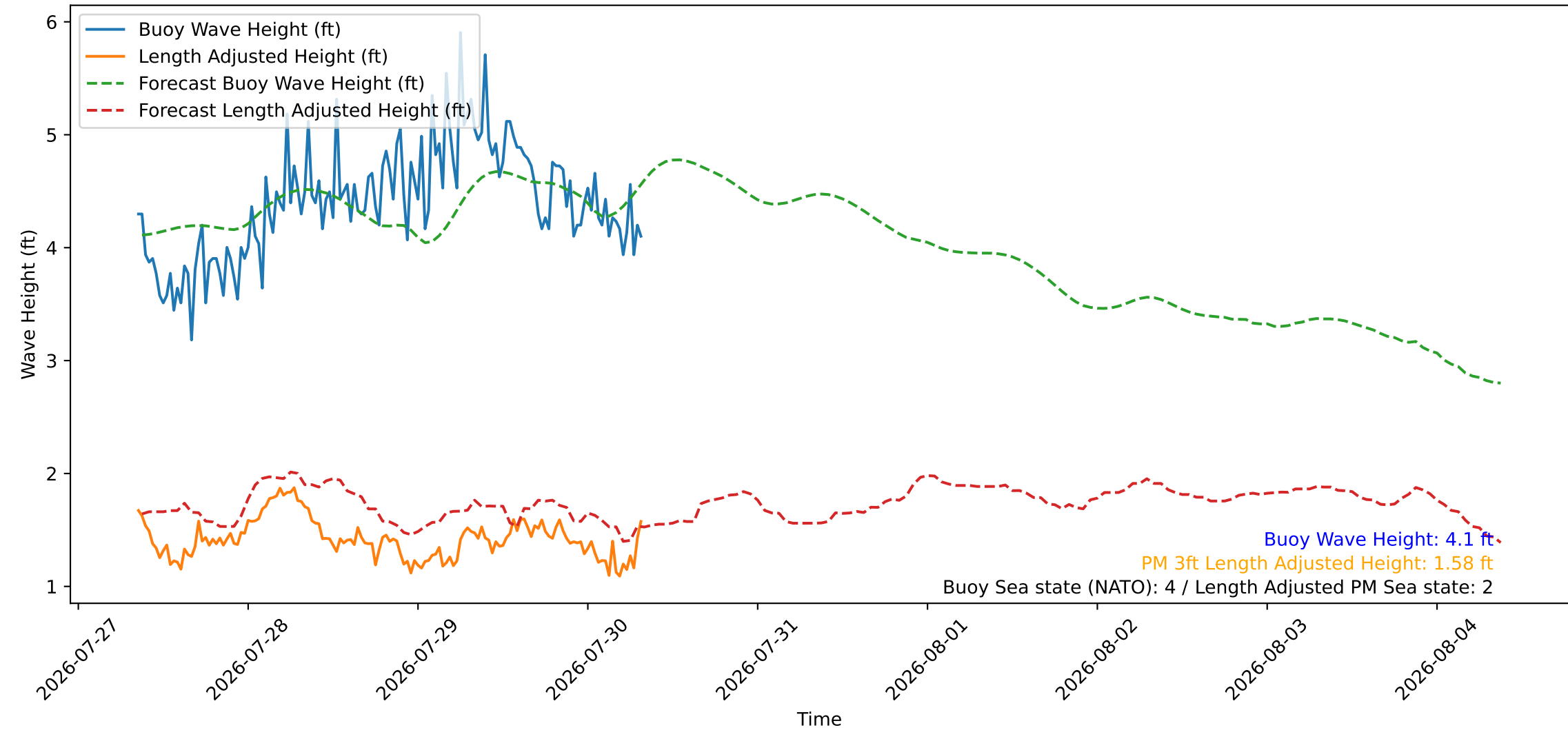
Wave Heights over Time for Oceanside Harbor at 2026-07-30 08:30:27
