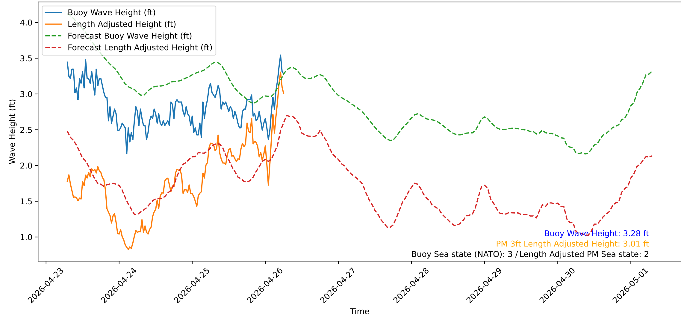
Wave Heights over Time for Red Beach at 2026-04-26 06:40:50
