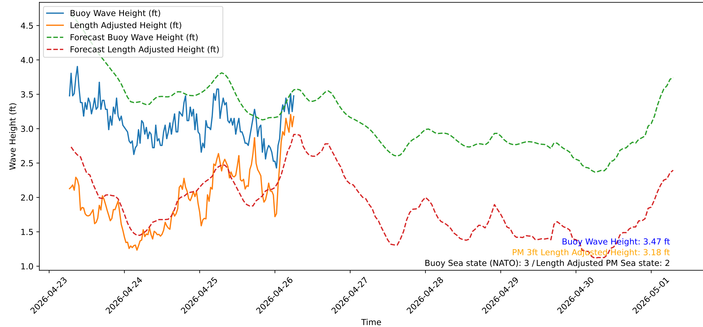
Wave Heights over Time for Green Beach at 2026-04-26 06:41:12
