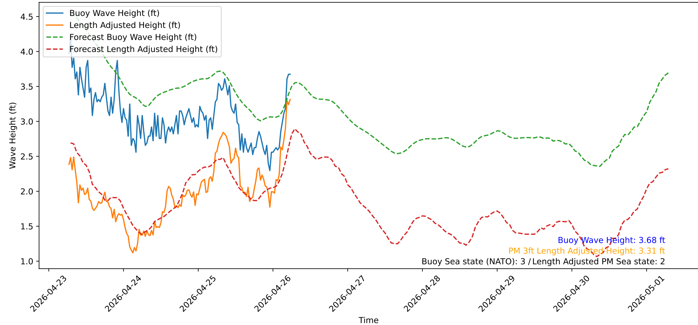
Wave Heights over Time for Oceanside Harbor at 2026-04-26 06:40:31
