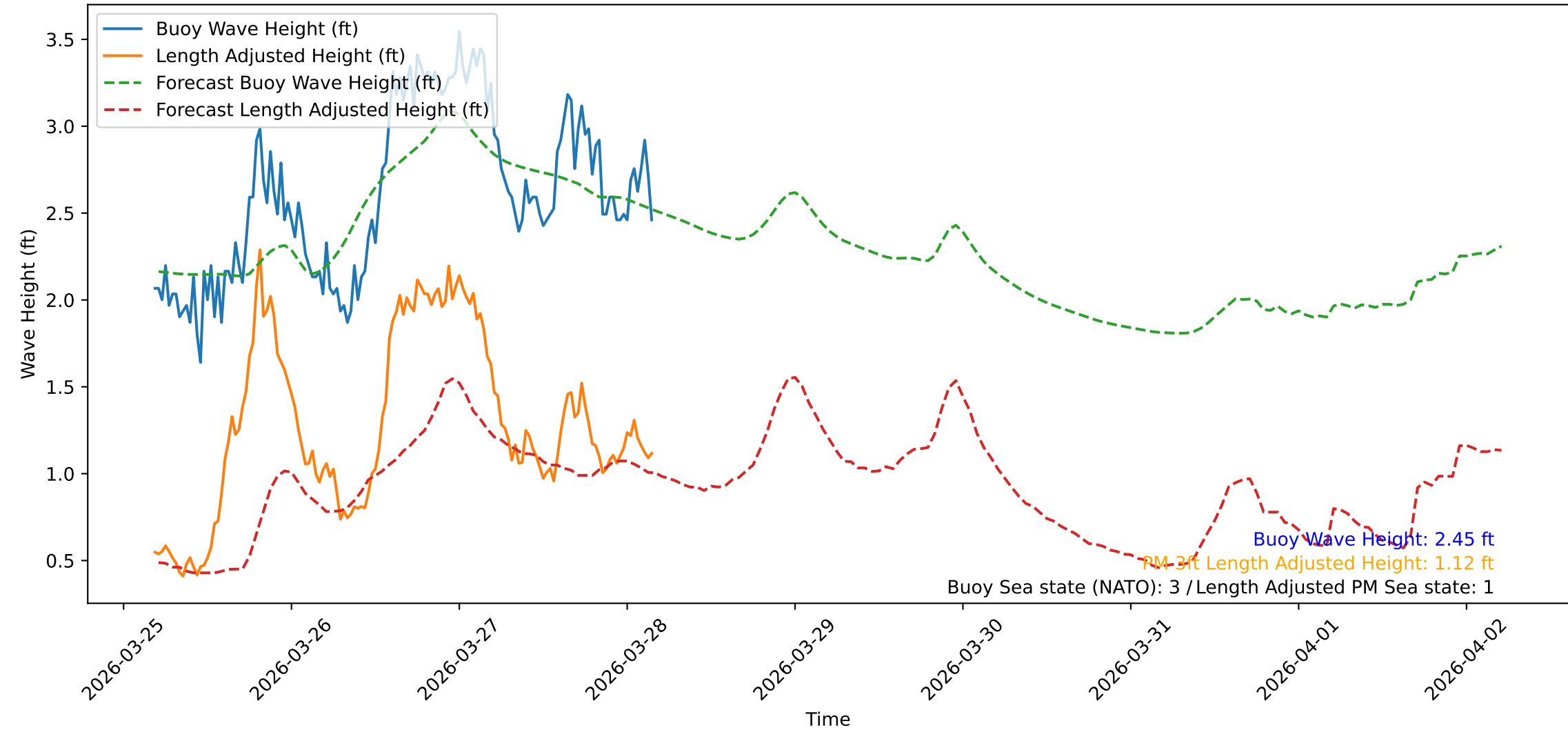
Wave Heights over Time for Green Beach at 2026-03-28 04:41:10
