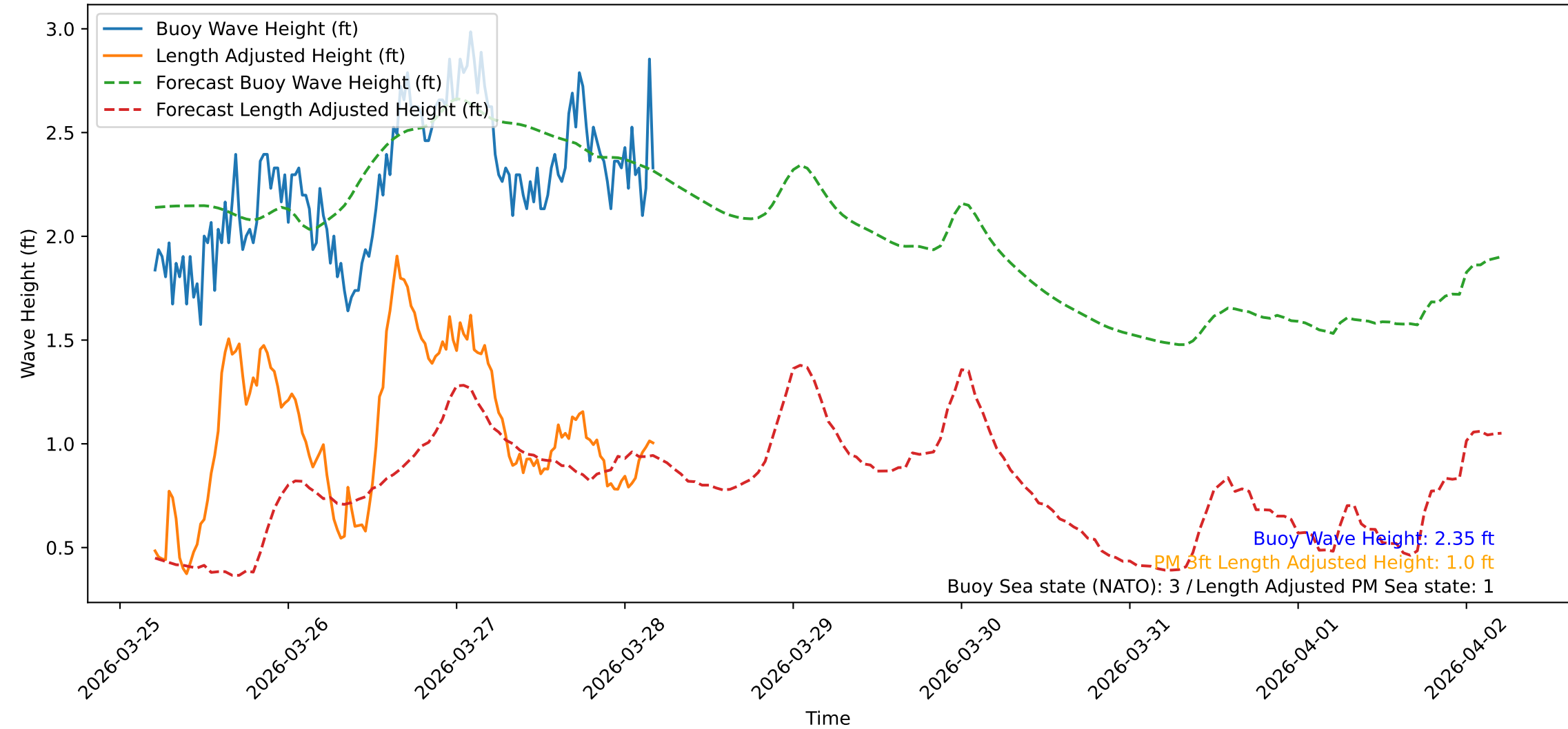
Wave Heights over Time for Red Beach at 2026-03-28 04:40:48
