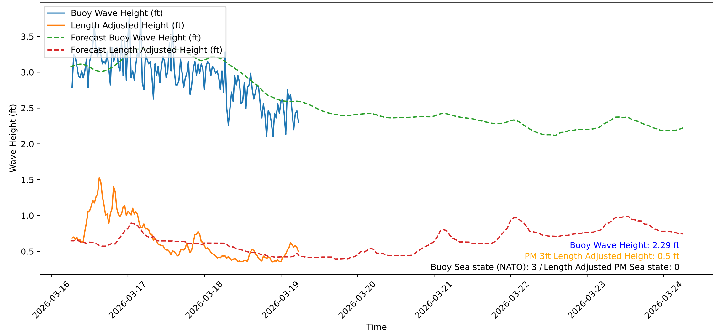
Wave Heights over Time for Red Beach at 2026-03-19 06:20:47
