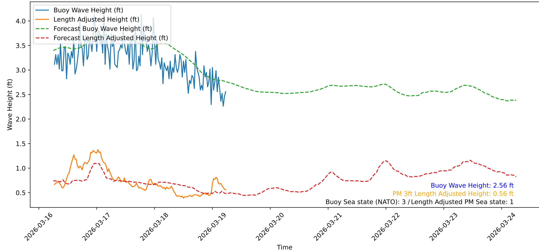
Wave Heights over Time for Green Beach at 2026-03-19 06:21:10
