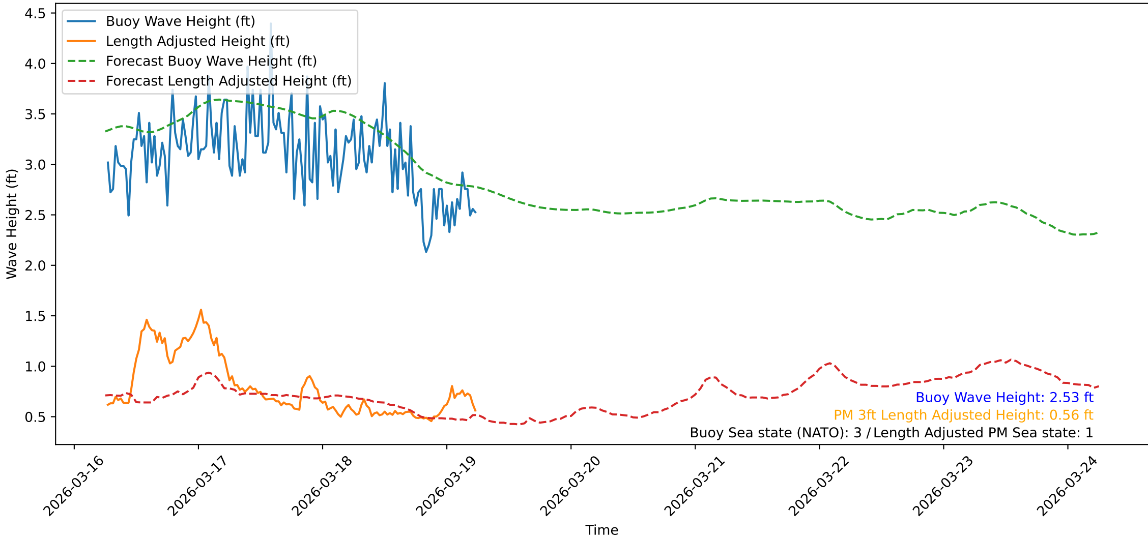
Wave Heights over Time for Oceanside Harbor at 2026-03-19 06:20:32
