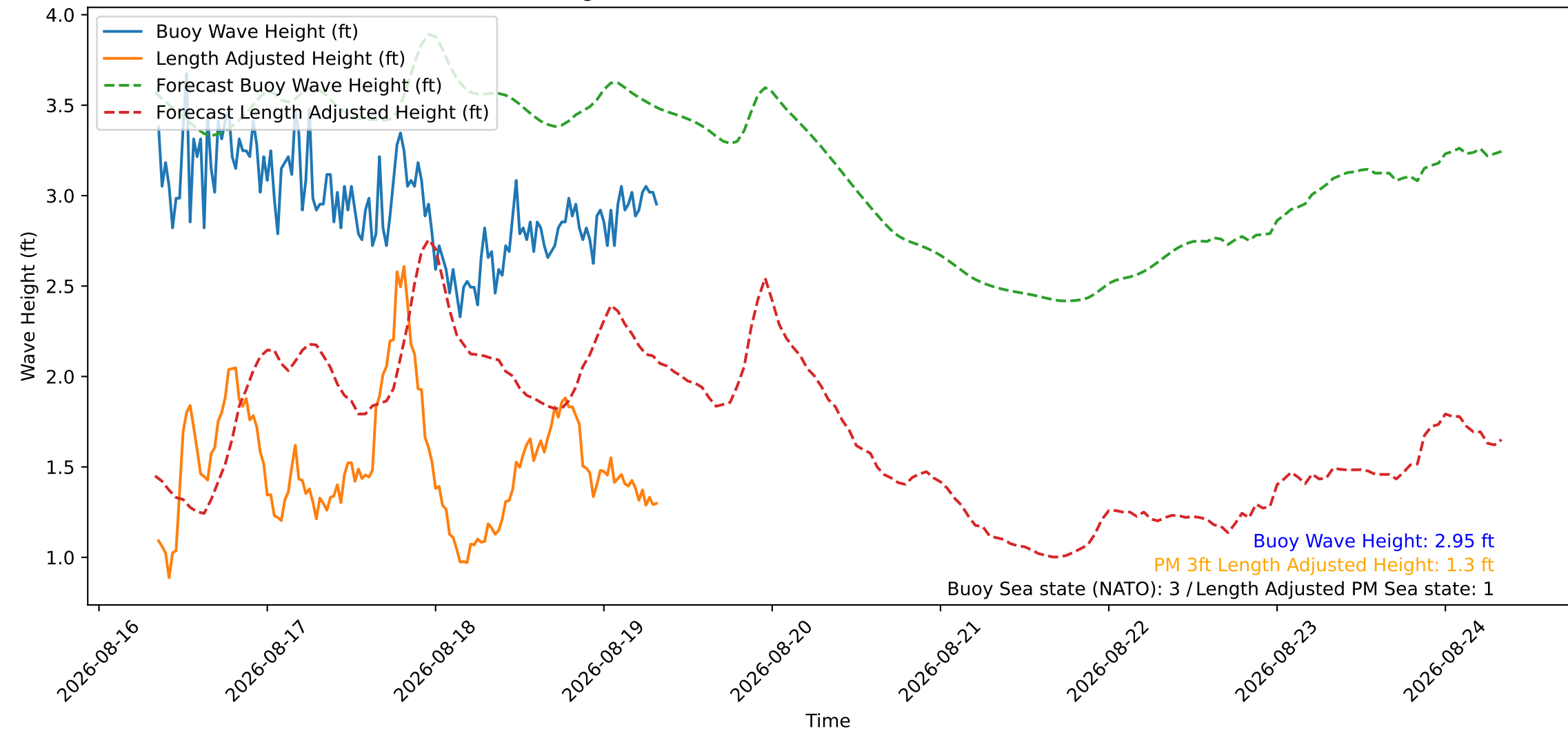
Wave Heights over Time for Red Beach at 2026-08-19 08:10:46
