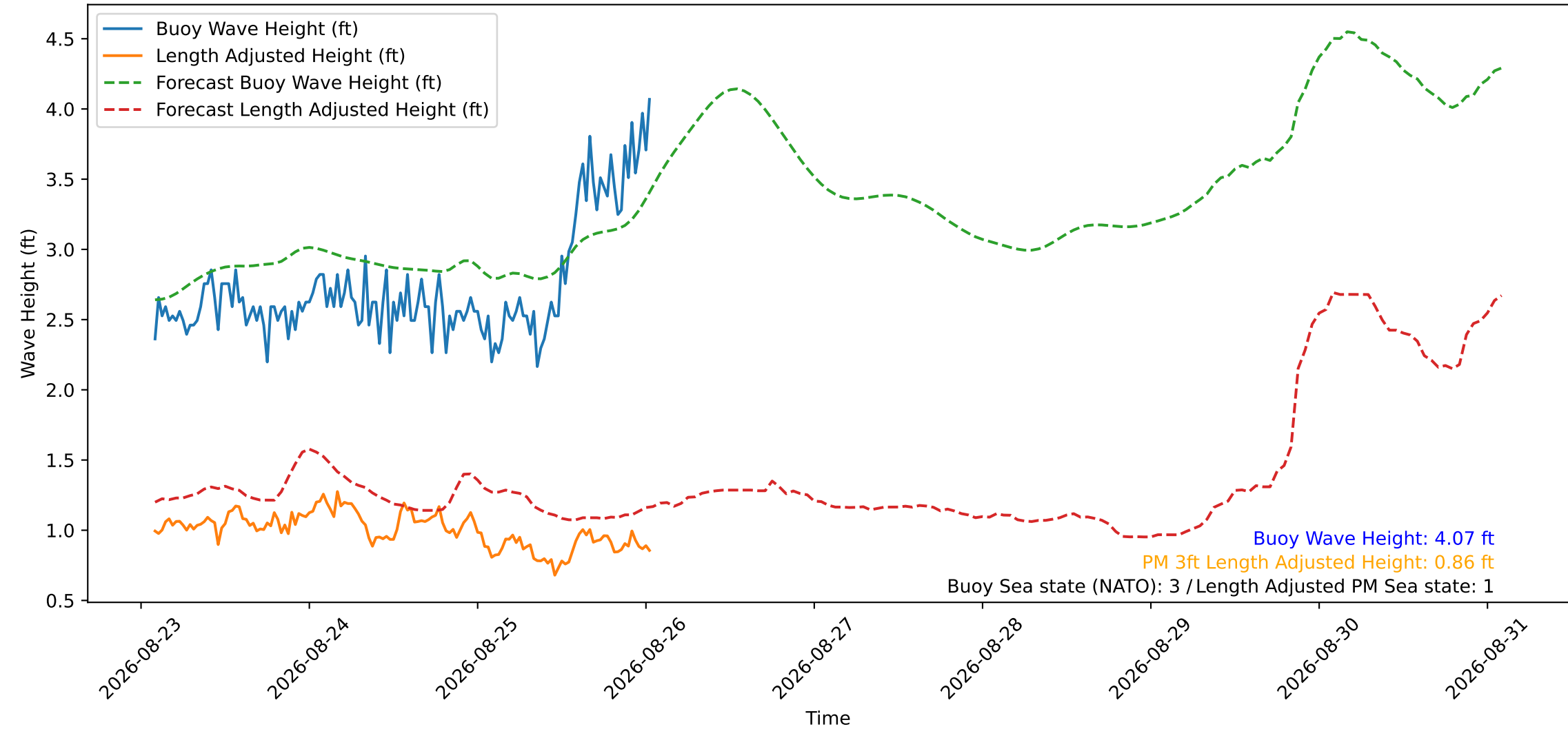
Wave Heights over Time for Red Beach at 2026-08-26 01:30:49
