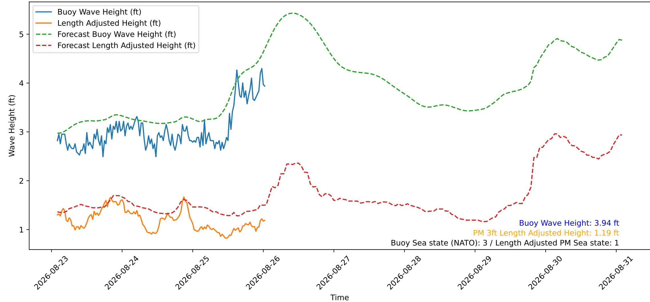
Wave Heights over Time for Green Beach at 2026-08-26 01:31:11
