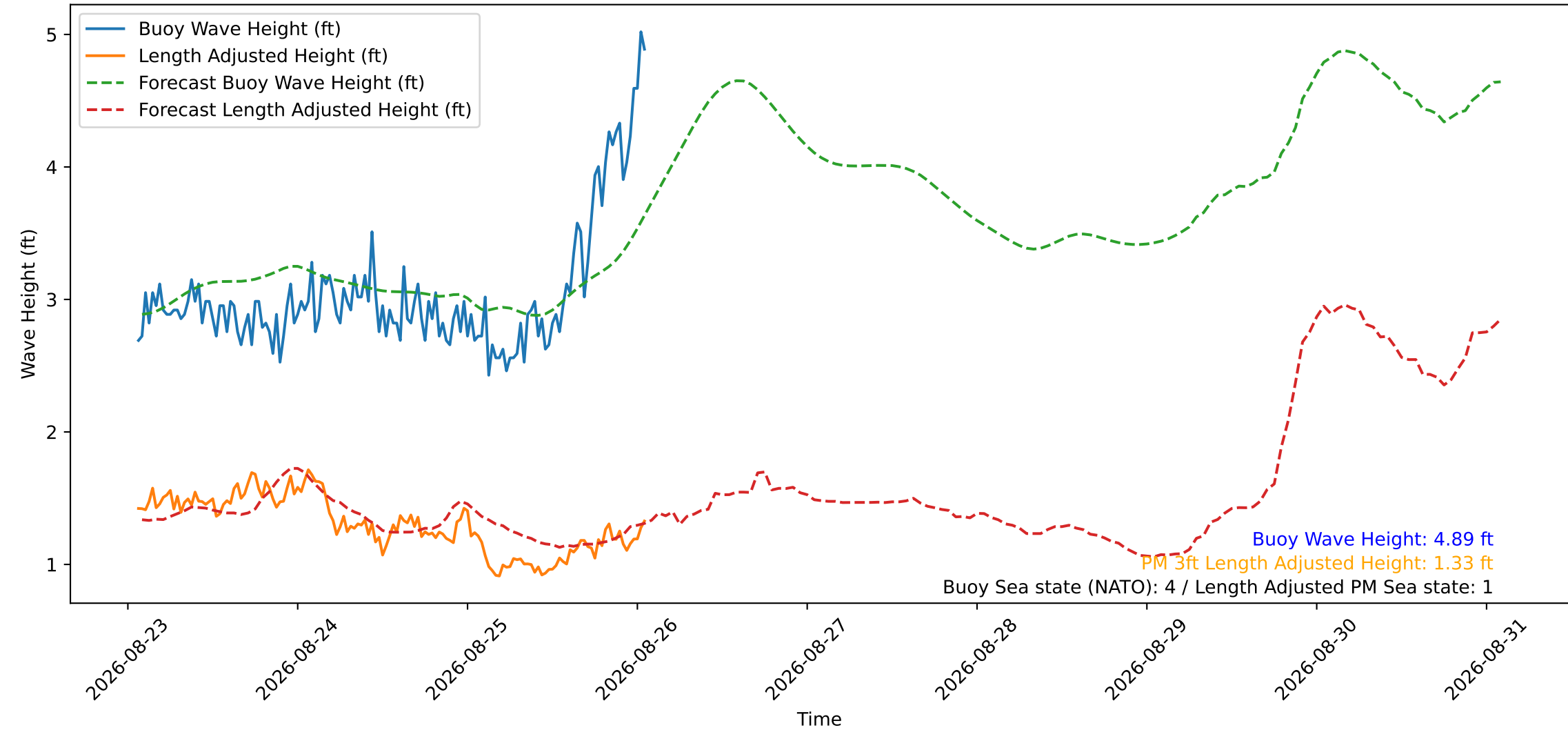
Wave Heights over Time for Oceanside Harbor at 2026-08-26 01:30:30
