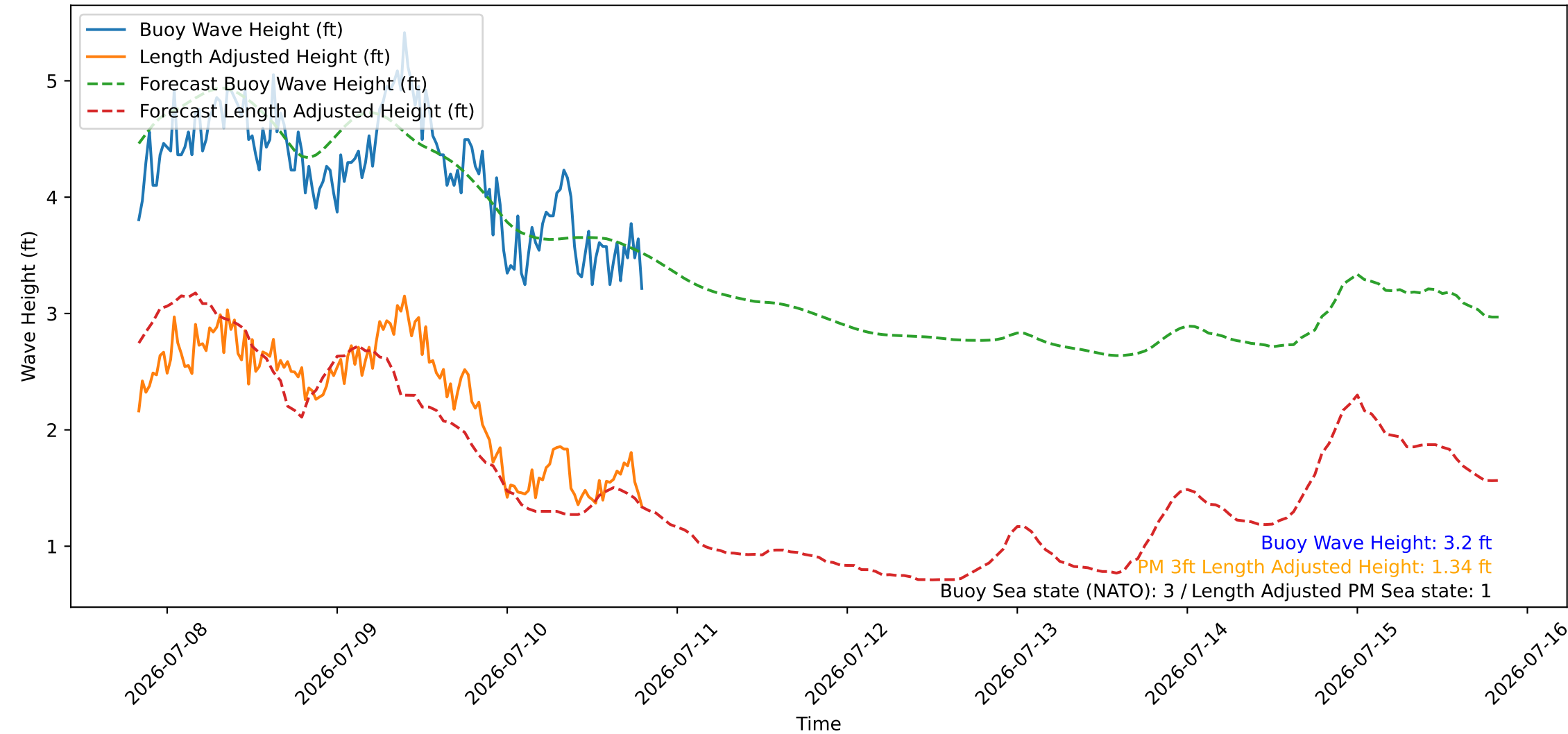
Wave Heights over Time for Oceanside Harbor at 2026-07-10 20:00:26
