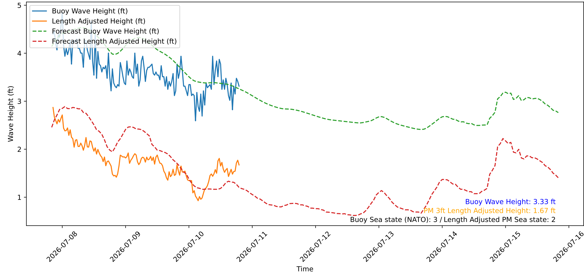
Wave Heights over Time for Red Beach at 2026-07-10 20:00:46
