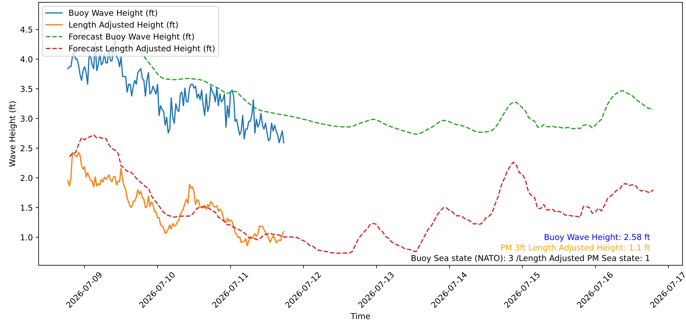
Wave Heights over Time for Green Beach at 2026-07-11 18:41:09
