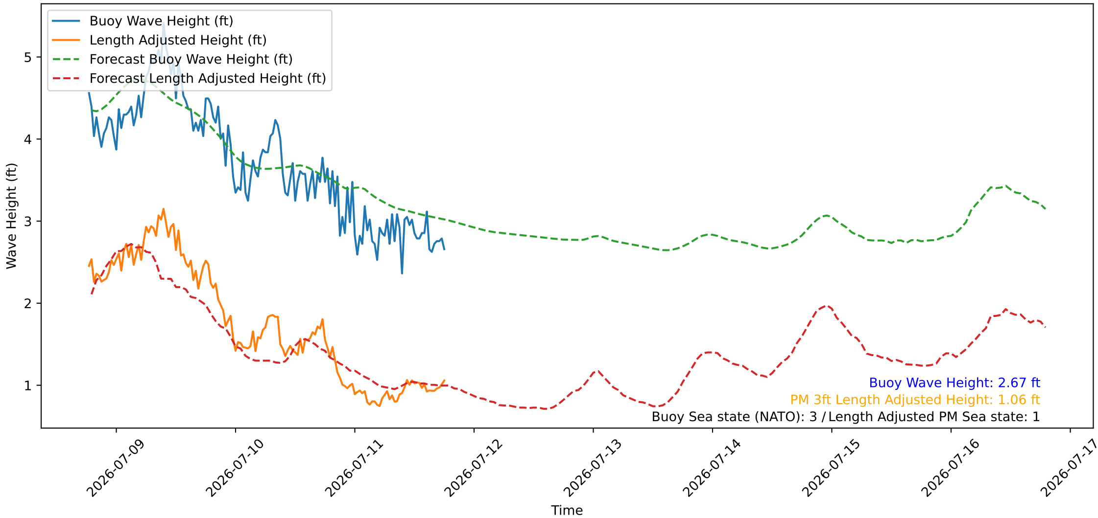
Wave Heights over Time for Oceanside Harbor at 2026-07-11 18:40:26
