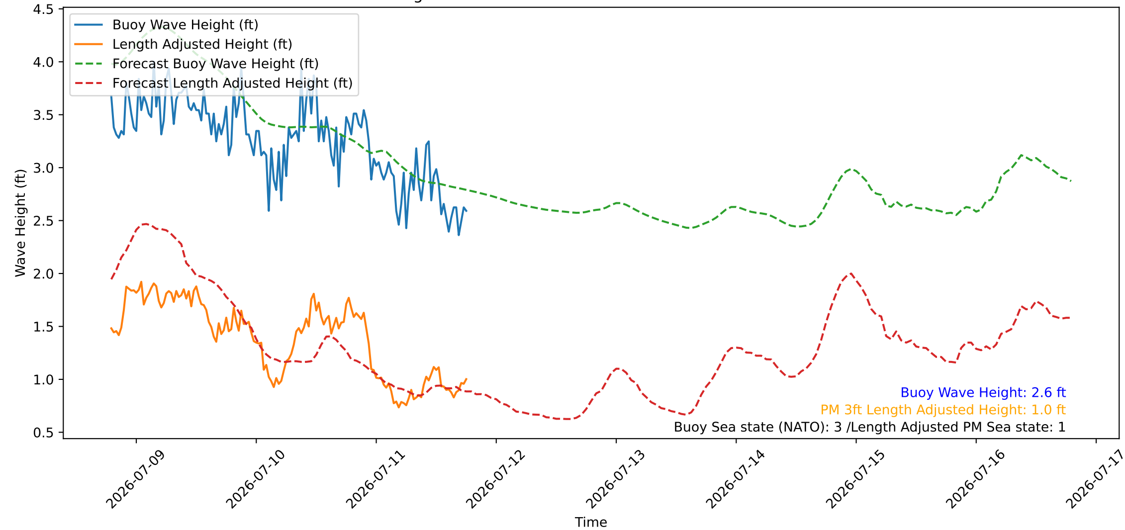
Wave Heights over Time for Red Beach at 2026-07-11 18:40:46
