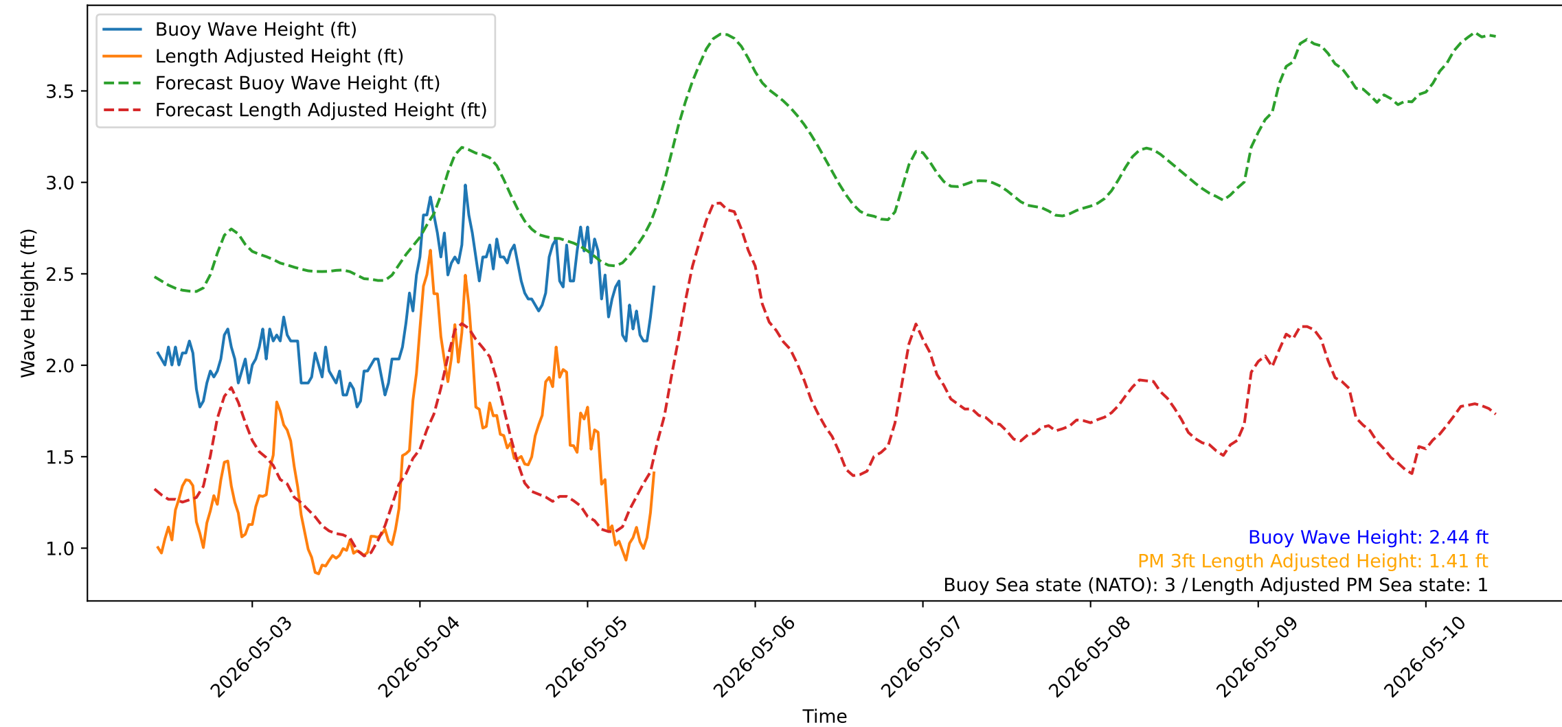
Wave Heights over Time for Green Beach at 2026-05-05 10:21:14
