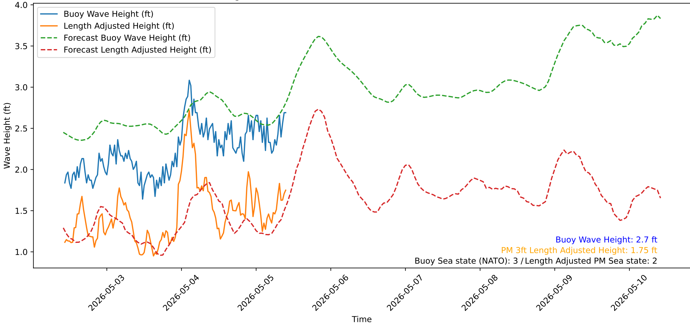
Wave Heights over Time for Oceanside Harbor at 2026-05-05 10:20:31
