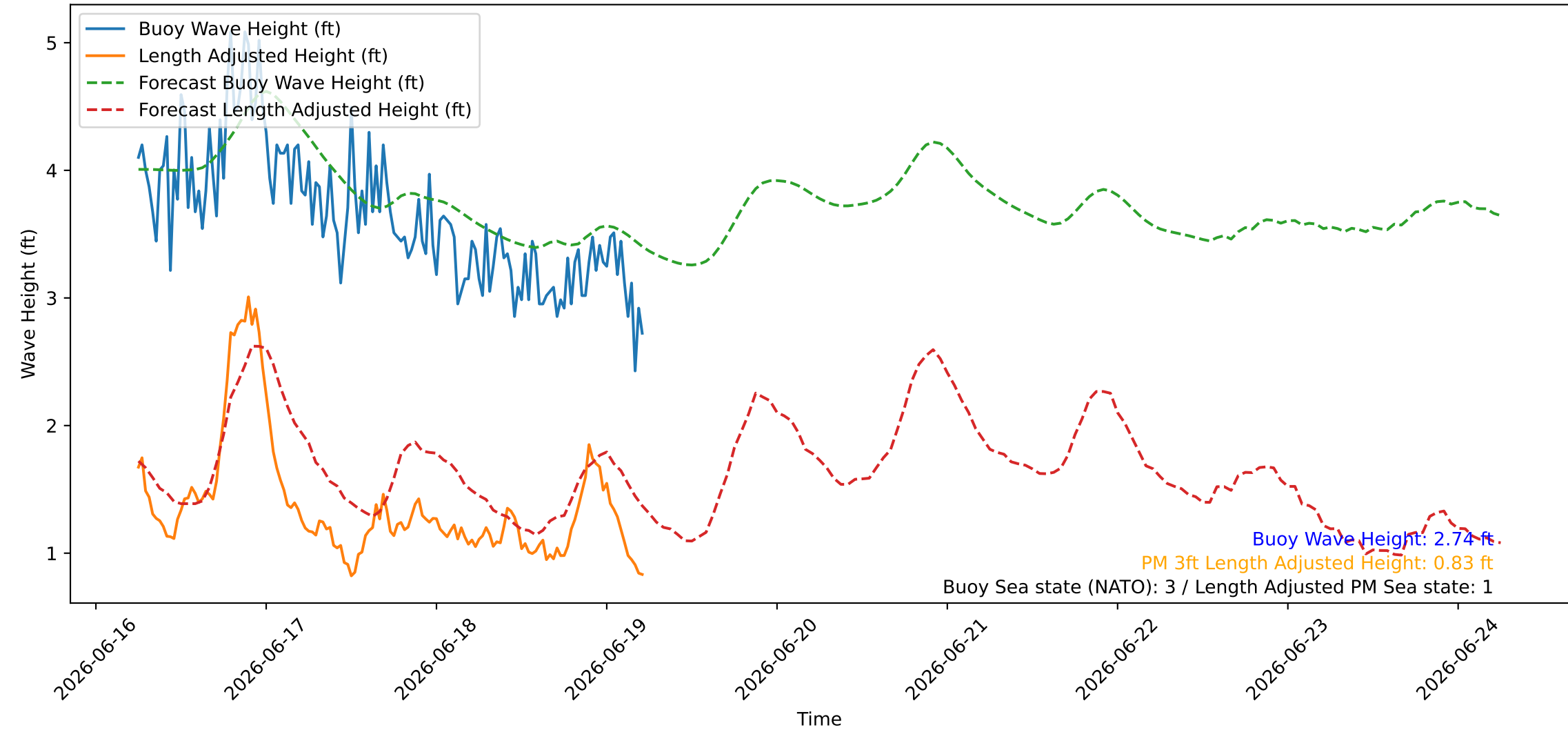
Wave Heights over Time for Green Beach at 2026-06-19 06:01:08
