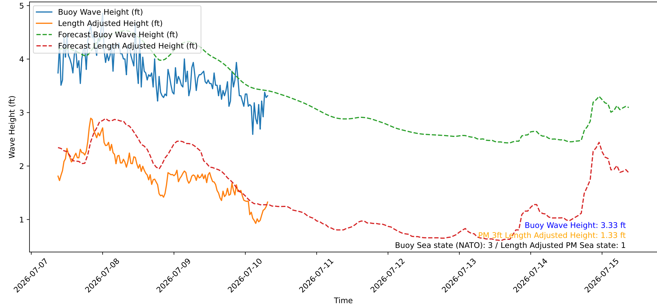
Wave Heights over Time for Red Beach at 2026-07-10 08:30:45
