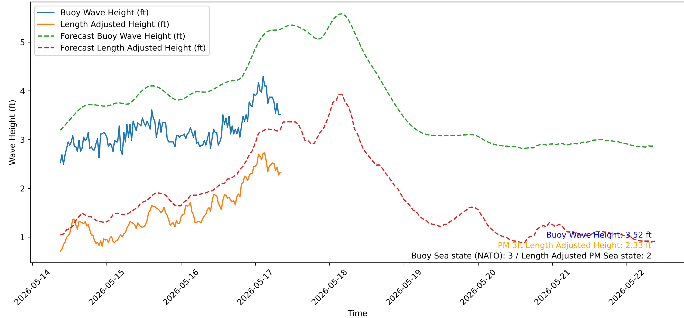
Wave Heights over Time for Oceanside Harbor at 2026-05-17 08:50:31
