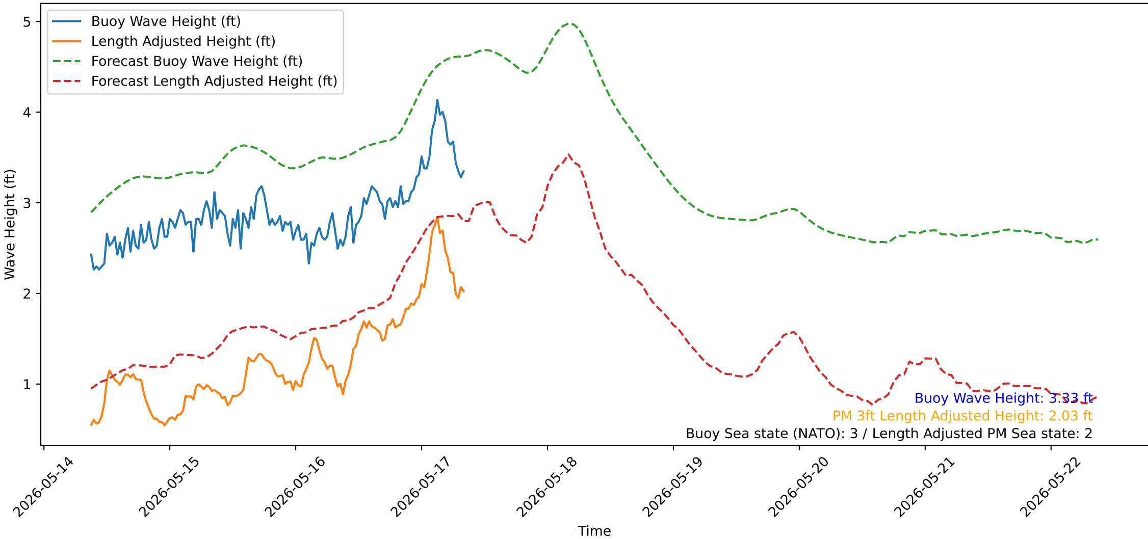
Wave Heights over Time for Red Beach at 2026-05-17 08:50:51
