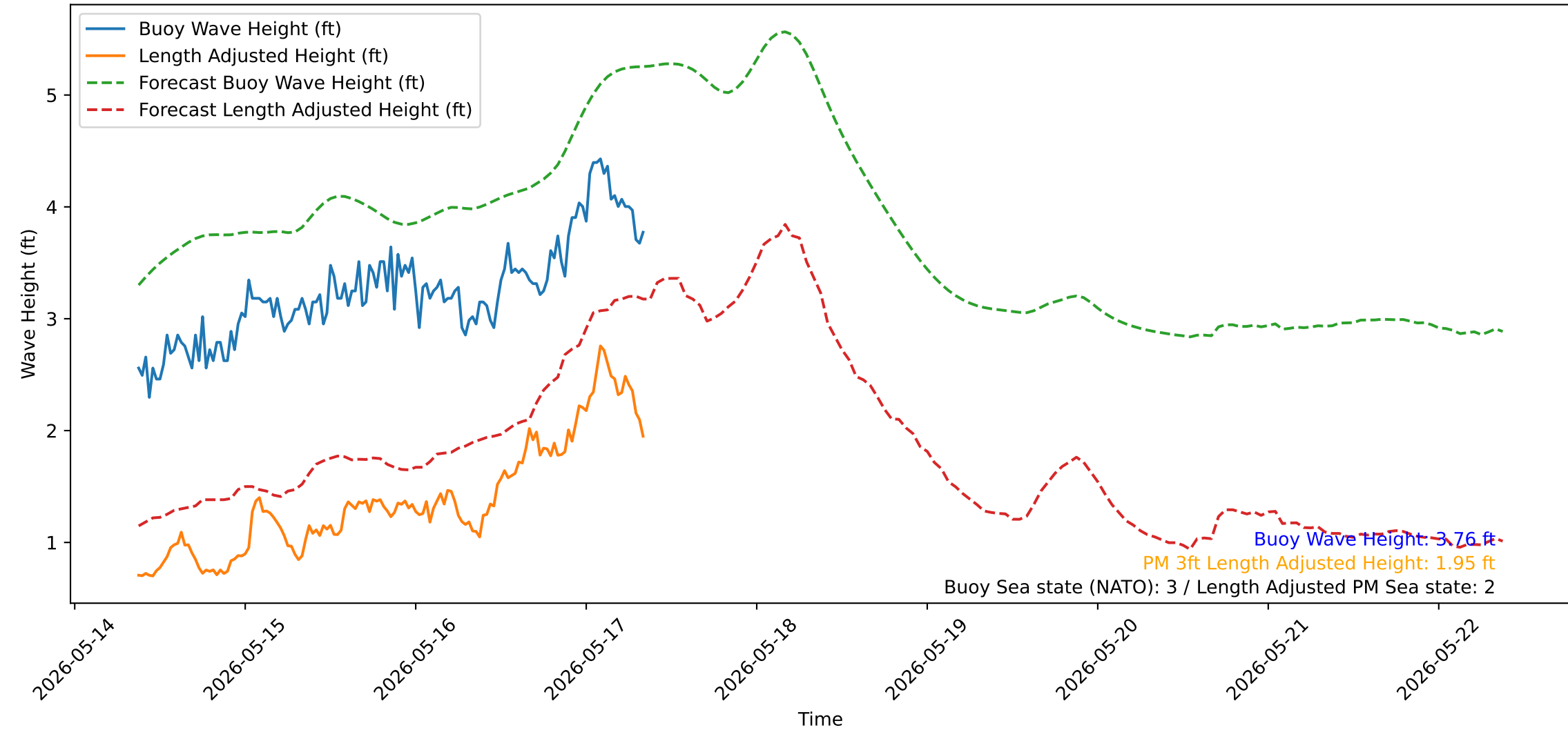
Wave Heights over Time for Green Beach at 2026-05-17 08:51:14
