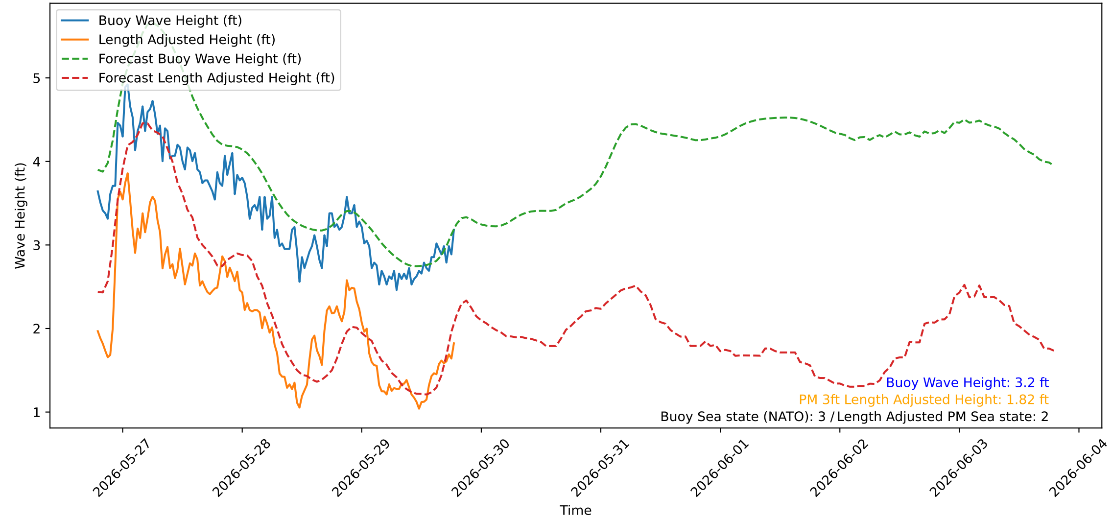
Wave Heights over Time for Green Beach at 2026-05-29 19:11:04
