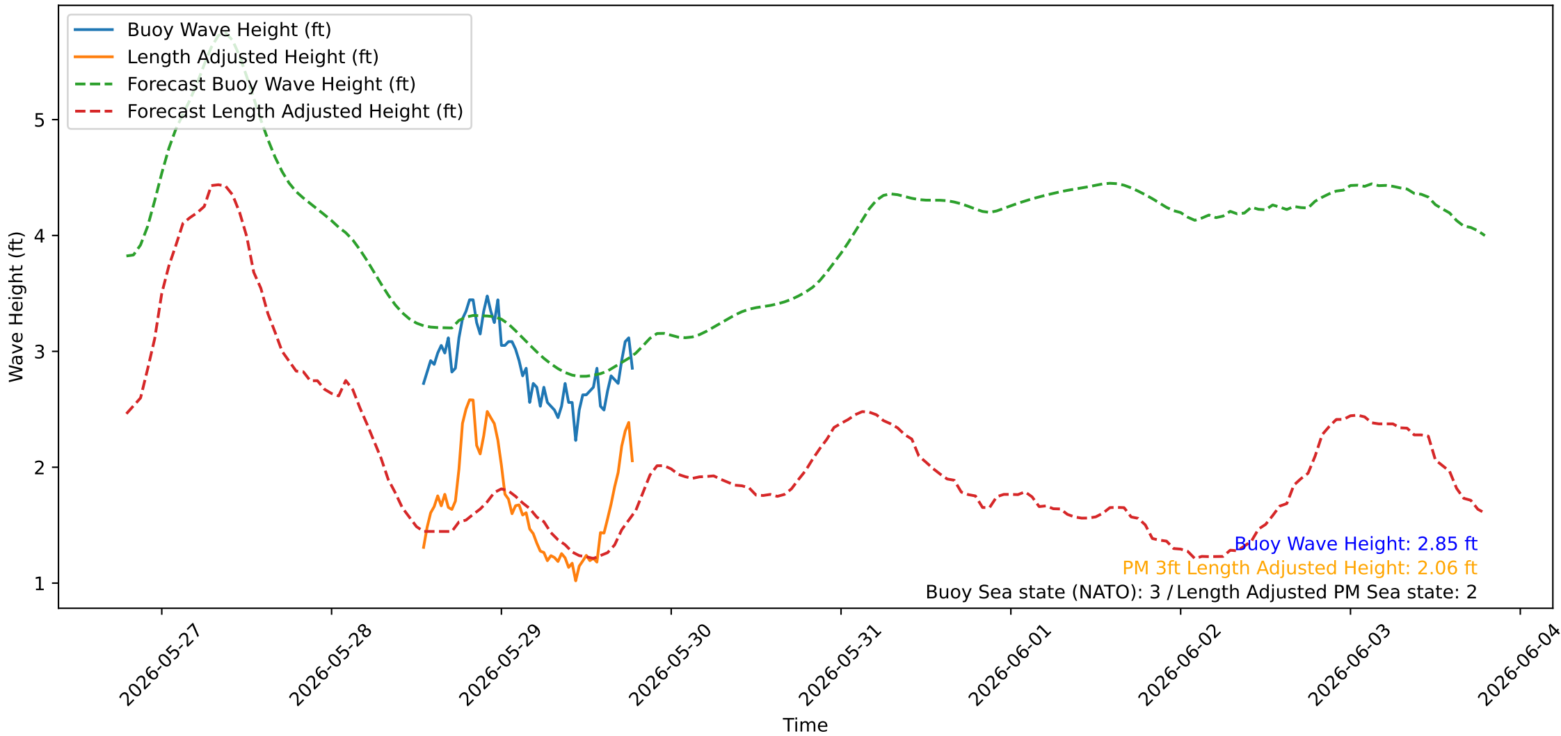
Wave Heights over Time for Oceanside Harbor at 2026-05-29 19:10:22
