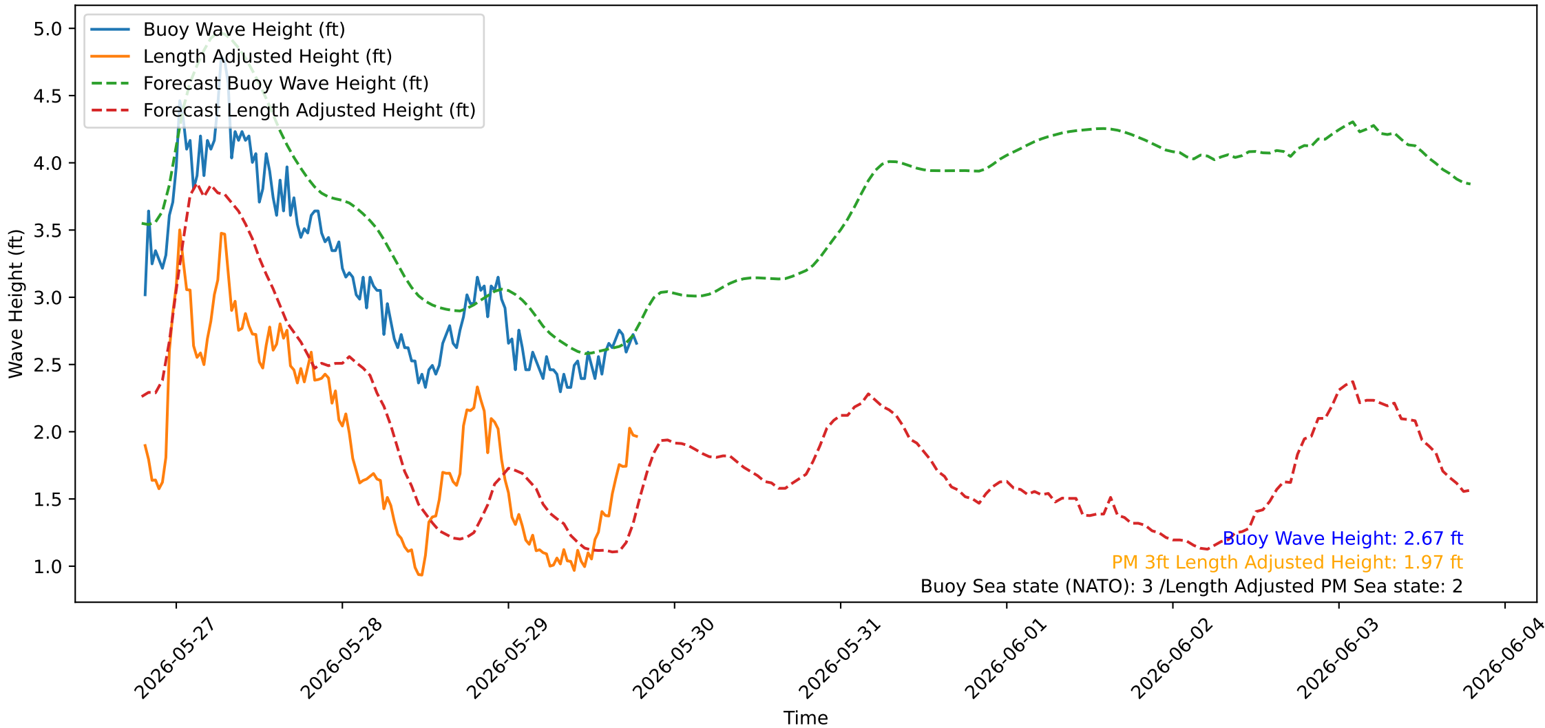
Wave Heights over Time for Red Beach at 2026-05-29 19:10:42
